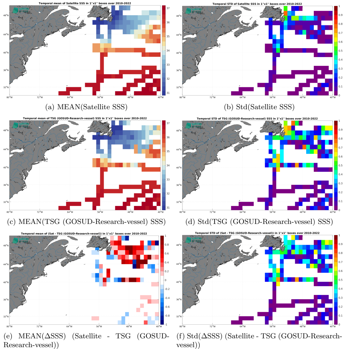
Figure 7: Temporal mean (left) and Std (right) of SSS from SMOS SSS L4 v1 - Monthly (CMEMS-CNR) (top), TSG (GOSUD-Research-vessel) (middle), and of \Delta SSS (Satellite - TSG (GOSUD-Research-vessel)). Only match-up pairs are used to generate these maps.
