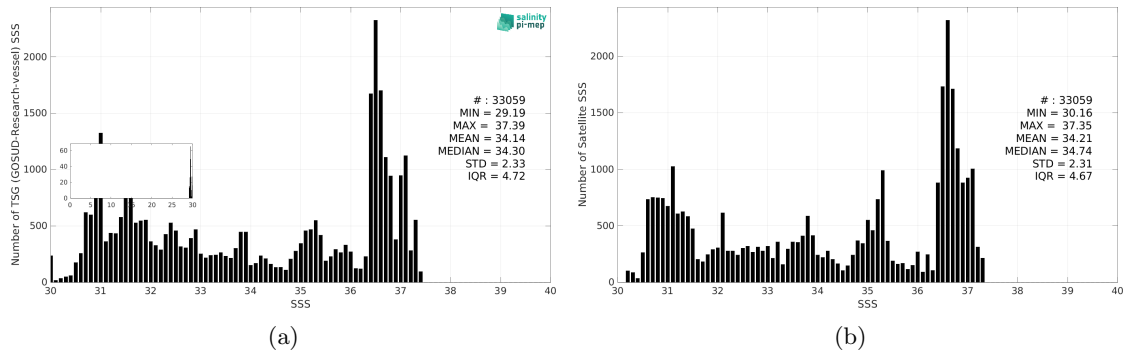
Figure 3: Histograms of SSS from TSG (GOSUD-Research-vessel) (a) and SMOS SSS L4 v1 - Monthly (CMEMS-CNR) (b) considering all match-up pairs per bins of 0.1 over the Gulf Stream Pi-MEP region and for the full satellite product period.
