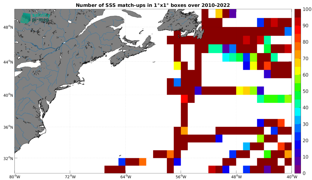
Figure 5: Number of SSS match-ups between TSG (GOSUD-Research-vessel) SSS and the SMOS SSS L4 v1 - Monthly (CMEMS-CNR) SSS product for the Gulf Stream Pi-MEP region over 1^\circ \times 1^\circ boxes and for the full satellite product period.
