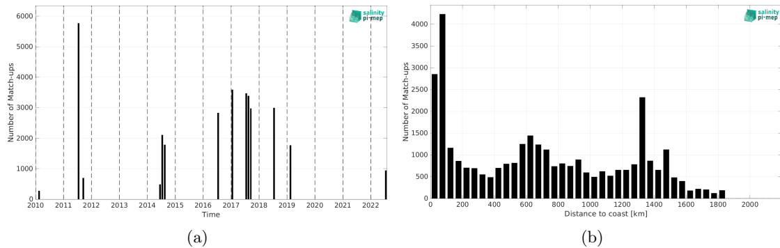
Figure 2: Number of match-ups between TSG (GOSUD-Research-vessel) and SMOS SSS L4 v1 - Monthly (CMEMS-CNR) SSS as a function of time (a) and as function of the distance to coast (b) over the Gulf Stream Pi-MEP region and for the full satellite product period.
