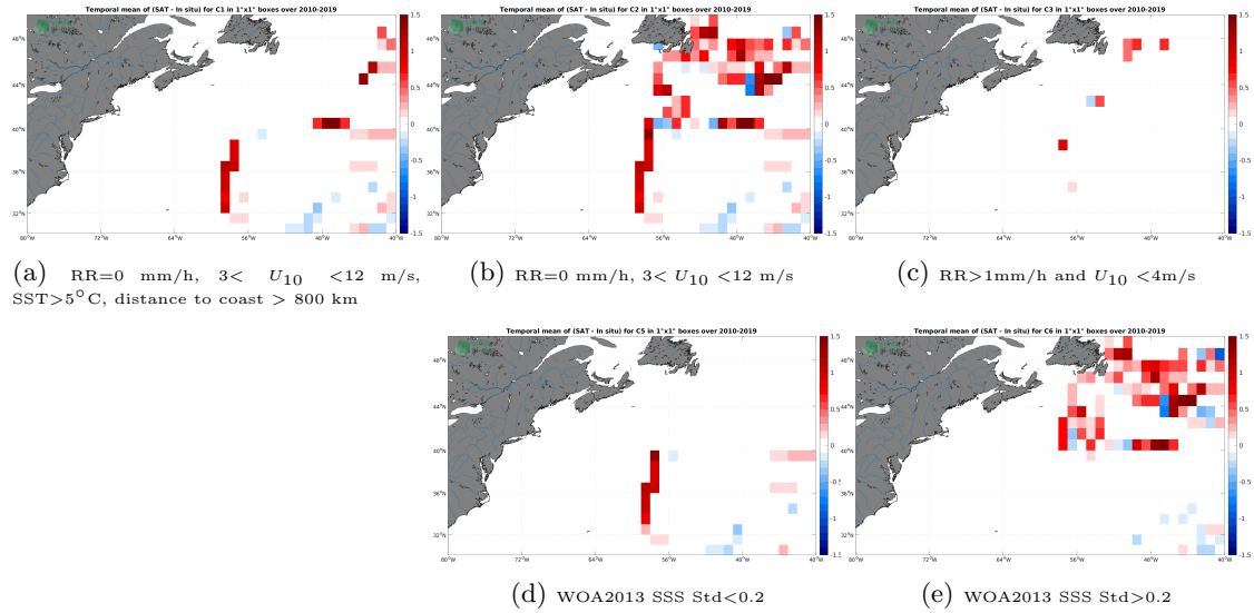
Figure 12: Temporal mean gridded over spatial boxes of size 1^{\circ}\times 1^{\circ} of \Delta SSS (SMOS SSS L4 v1 - Monthly (CMEMS-CNR) - TSG (GOSUD-Research-vessel)) for 5 different subdatasets corresponding to:RR=0 mm/h, 3 < U_{10} < 12 m/s, SST >5^{\circ}\text{C} , distance to coast > 800 km (a), RR=0 mm/h, 3 < U_{10} < 12 m/s (b), RR >1 mm/h and U_{10} < 4 m/s (c), WOA2013 SSS Std <0.2 (d), WOA2013 SSS Std >0.2 (e).
