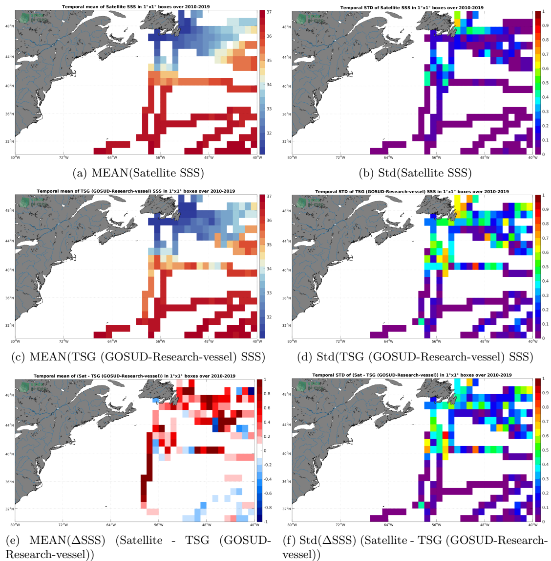
Figure 6: Temporal mean (left) and Std (right) of SSS from SMOS SSS L4 v1 - Monthly (CMEMS-CNR) (top), TSG (GOSUD-Research-vessel) (middle), and of \Delta SSS (Satellite - TSG (GOSUD-Research-vessel)). Only match-up pairs are used to generate these maps.
