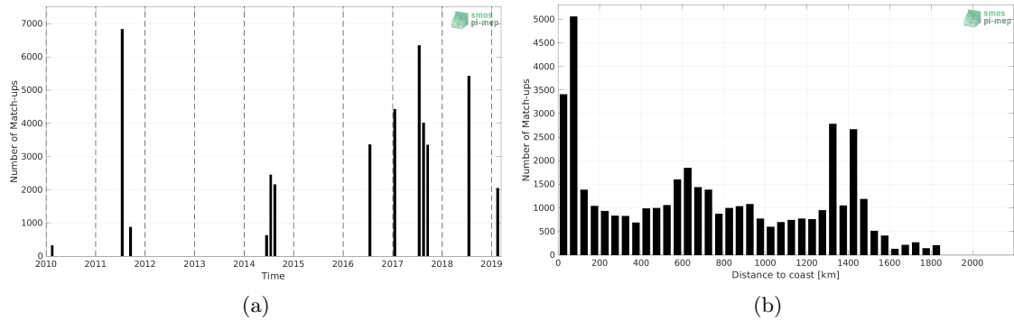
Figure 1: Number of match-ups between TSG (GOSUD-Research-vessel) and SMOS SSS L4 v1 - Monthly (CMEMS-CNR) SSS as a function of time (a) and as function of the distance to coast (b) over the Gulf Stream Pi-MEP region and for the full satellite product period.
