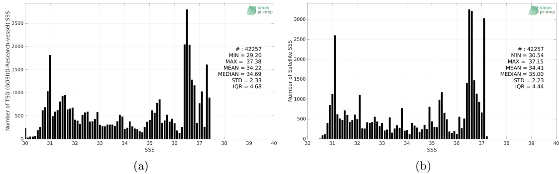
Figure 2: Histograms of SSS from TSG (GOSUD-Research-vessel) (a) and SMOS SSS L4 v1 - Monthly (CMEMS-CNR) (b) considering all match-up pairs per bins of 0.1 over the Gulf Stream Pi-MEP region and for the full satellite product period.
