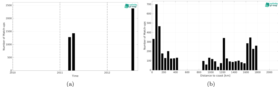
Figure 2: Number of match-ups between TSG (CSIC-UTM) and SMOS SSS L4 v1 - Monthly (CMEMS-CNR) SSS as a function of time (a) and as function of the distance to coast (b) over the Gulf Stream Pi-MEP region and for the full satellite product period.
