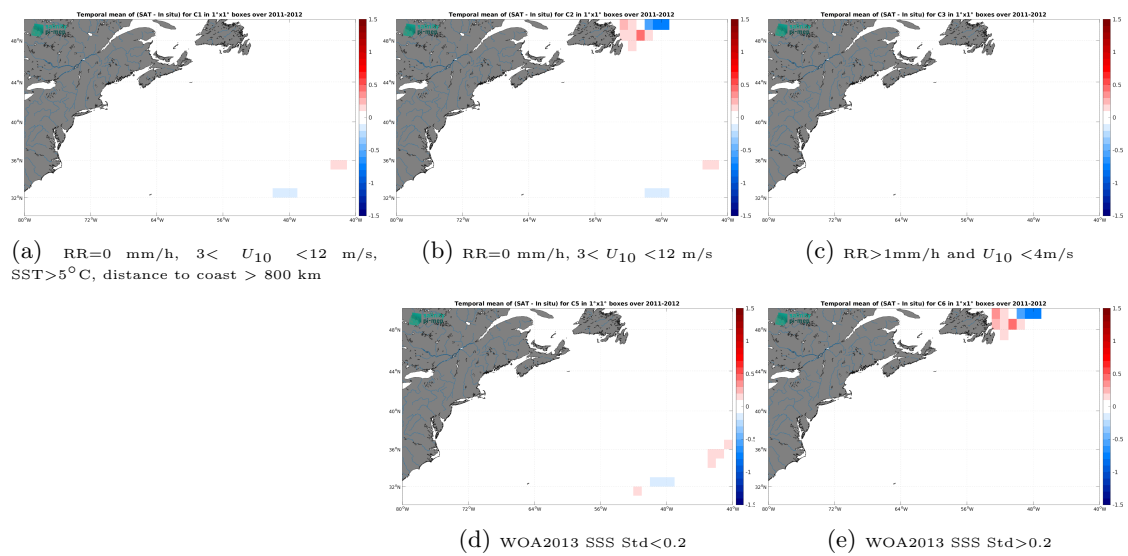
Figure 14: Temporal mean gridded over spatial boxes of size 1^\circ \times 1^\circ of \Delta SSS (SMOS SSS L4 v1 - Monthly (CMEMS-CNR) - TSG (CSIC-UTM)) for 5 different subdatasets corresponding to:RR=0 mm/h, 3 < U_{10} < 12 m/s, SST>5°C, distance to coast > 800 km (a), RR=0 mm/h, 3 < U_{10} < 12 m/s (b), RR>1mm/h and U_{10} < 4 m/s (c), WOA2013 SSS Std<0.2 (d), WOA2013 SSS Std>0.2 (e).
