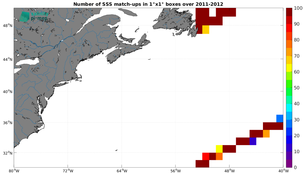
Figure 5: Number of SSS match-ups between TSG (CSIC-UTM) SSS and the SMOS SSS L4 v1 - Monthly (CMEMS-CNR) SSS product for the Gulf Stream Pi-MEP region over 1^\circ \times 1^\circ boxes and for the full satellite product period.
