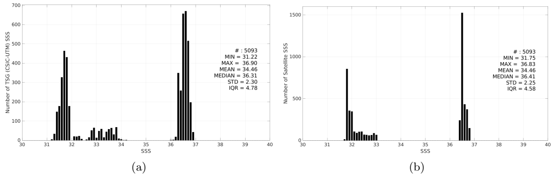
Figure 3: Histograms of SSS from TSG (CSIC-UTM) (a) and SMOS SSS L4 v1 - Monthly (CMEMS-CNR) (b) considering all match-up pairs per bins of 0.1 over the Gulf Stream Pi-MEP region and for the full satellite product period.
