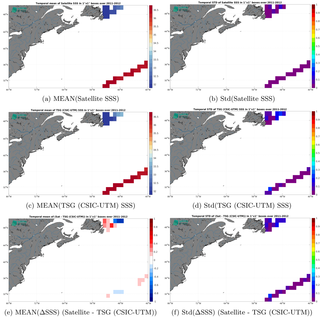
Figure 7: Temporal mean (left) and Std (right) of SSS from SMOS SSS L4 v1 - Monthly (CMEMS-CNR) (top), TSG (CSIC-UTM) (middle), and of \Delta SSS (Satellite - TSG (CSIC-UTM)). Only match-up pairs are used to generate these maps.
