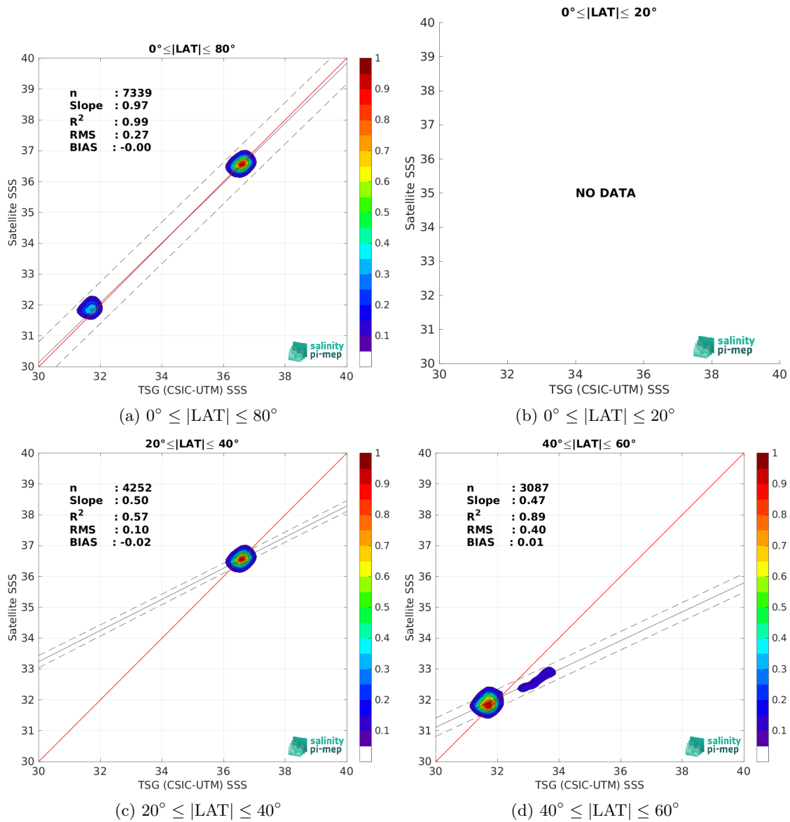
Figure 9: Contour maps of the concentration of SMOS SSS L4 v1 - Monthly (CMEMS-CNR) SSS (y-axis) versus TSG (CSIC-UTM) SSS (x-axis) at match-up pairs for different latitude bands. For each plot, the red line shows x=y . The black thin and dashed lines indicate a linear fit through the data cloud and the \pm 95\% confidence levels, respectively. The number match-up pairs n , the slope and R^2 coefficient of the linear fit, the root mean square (RMS) and the mean bias between satellite and in situ data are indicated for each latitude band in each plots.
