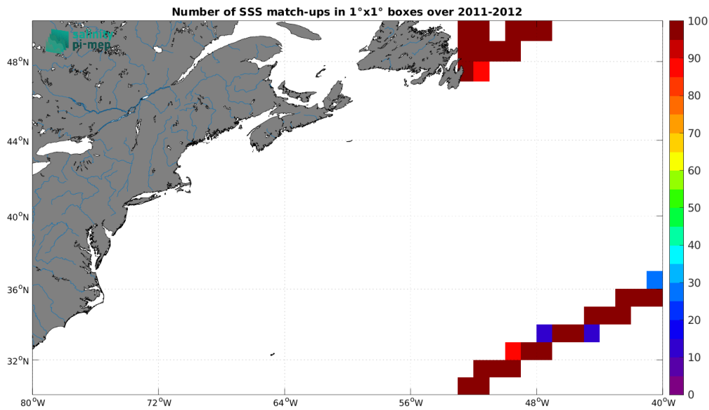
Figure 4: Number of SSS match-ups between TSG (CSIC-UTM) SSS and the SMOS SSS L4 v1 - Monthly (CMEMS-CNR) SSS product for the Gulf Stream Pi-MEP region over 1^\circ \times 1^\circ boxes and for the full satellite product period.
