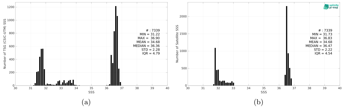
Figure 2: Histograms of SSS from TSG (CSIC-UTM) (a) and SMOS SSS L4 v1 - Monthly (CMEMS-CNR) (b) considering all match-up pairs per bins of 0.1 over the Gulf Stream Pi-MEP region and for the full satellite product period.
