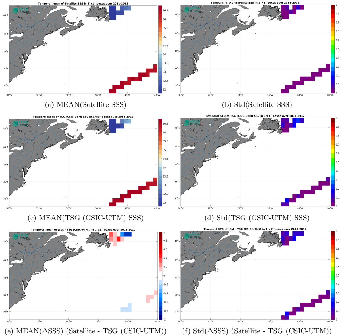
Figure 6: Temporal mean (left) and Std (right) of SSS from SMOS SSS L4 v1 - Monthly (CMEMS-CNR) (top), TSG (CSIC-UTM) (middle), and of \Delta SSS (Satellite - TSG (CSIC-UTM)). Only match-up pairs are used to generate these maps.
