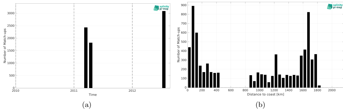
Figure 1: Number of match-ups between TSG (CSIC-UTM) and SMOS SSS L4 v1 - Monthly (CMEMS-CNR) SSS as a function of time (a) and as function of the distance to coast (b) over the Gulf Stream Pi-MEP region and for the full satellite product period.
