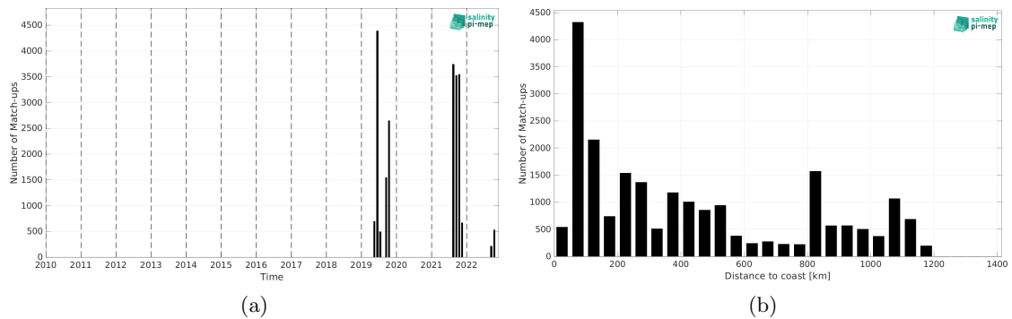
Figure 1: Number of match-ups between Saildrone and SMOS SSS L4 v1 - Monthly (CMEMS-CNR) SSS as a function of time (a) and as function of the distance to coast (b) over the Gulf Stream Pi-MEP region and for the full satellite product period.
