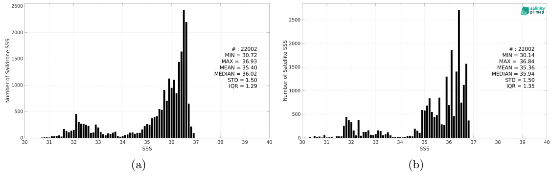
Figure 2: Histograms of SSS from Saildrone (a) and SMOS SSS L4 v1 - Monthly (CMEMS-CNR) (b) considering all match-up pairs per bins of 0.1 over the Gulf Stream Pi-MEP region and for the full satellite product period.
