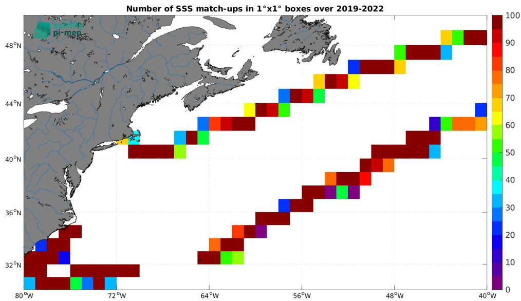
Figure 4: Number of SSS match-ups between Saildrone SSS and the SMOS SSS L4 v1 - Monthly (CMEMS-CNR) SSS product for the Gulf Stream Pi-MEP region over 1^{\circ} \times 1^{\circ} boxes and for the full satellite product period.
