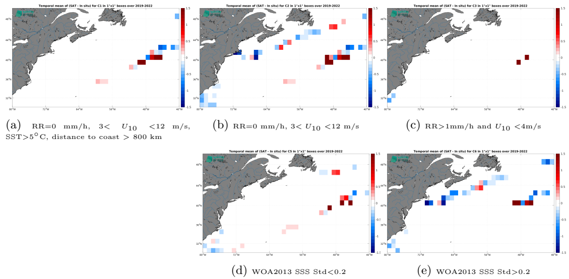
Figure 12: Temporal mean gridded over spatial boxes of size 1^\circ \times 1^\circ of \Delta SSS (SMOS SSS L4 v1 - Monthly (CMEMS-CNR) - Saifdrone) for 5 different subdatasets corresponding to:RR=0 mm/h, 3 < U_{10} < 12 m/s, SST >5^\circ C, distance to coast > 800 km (a), RR=0 mm/h, 3 < U_{10} < 12 m/s (b), RR >1 mm/h and U_{10} < 4 m/s (c), WOA2013 SSS Std <0.2 (d), WOA2013 SSS Std >0.2 (e).
