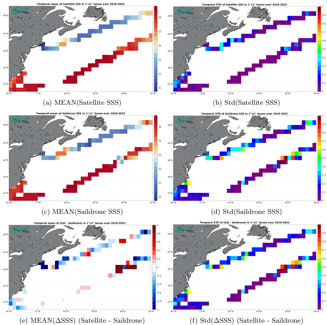
Figure 6: Temporal mean (left) and Std (right) of SSS from SMOS SSS L4 v1 - Monthly (CMEMS-CNR) (top), Saildrone (middle), and of \Delta SSS (Satellite - Saildrone). Only match-up pairs are used to generate these maps.
