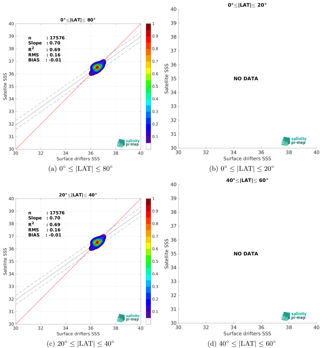
Figure 9: Contour maps of the concentration of SMOS SSS L4 v1 - Monthly (CMEMS-CNR) SSS (y-axis) versus Surface drifters SSS (x-axis) at match-up pairs for different latitude bands. For each plot, the red line shows x=y . The black thin and dashed lines indicate a linear fit through the data cloud and the \pm 95\% confidence levels, respectively. The number match-up pairs n , the slope and R^2 coefficient of the linear fit, the root mean square (RMS) and the mean bias between satellite and in situ data are indicated for each latitude band in each plots.
