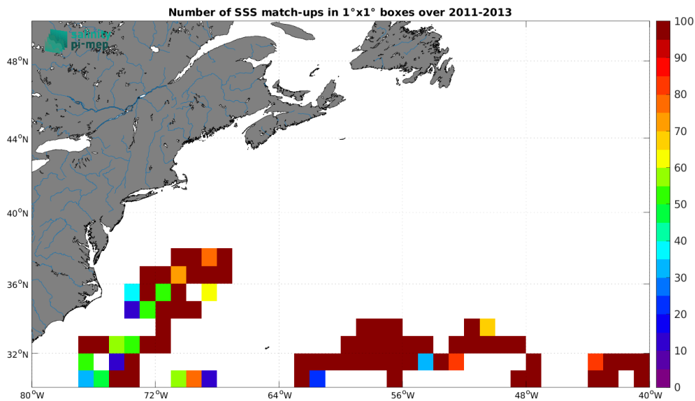
Figure 4: Number of SSS match-ups between Surface drifters SSS and the SMOS SSS L4 v1 - Monthly (CMEMS-CNR) SSS product for the Gulf Stream Pi-MEP region over 1^\circ \times 1^\circ boxes and for the full satellite product period.
