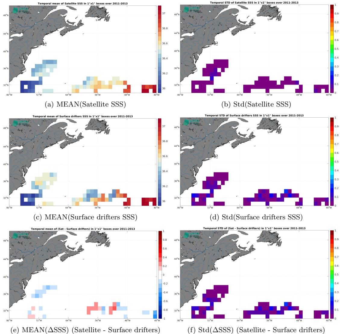
Figure 6: Temporal mean (left) and Std (right) of SSS from SMOS SSS L4 v1 - Monthly (CMEMS-CNR) (top), Surface drifters (middle), and of \Delta SSS (Satellite - Surface drifters). Only match-up pairs are used to generate these maps.
