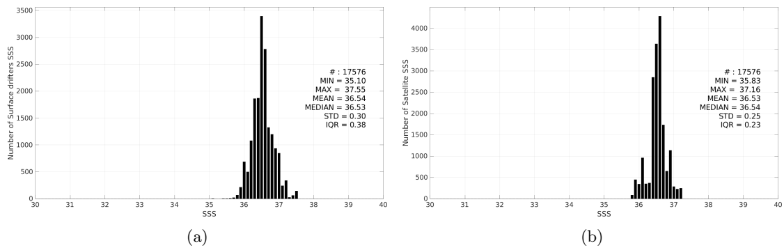
Figure 3: Histograms of SSS from Surface drifters (a) and SMOS SSS L4 v1 - Monthly (CMEMS-CNR) (b) considering all match-up pairs per bins of 0.1 over the Gulf Stream Pi-MEP region and for the full satellite product period.
