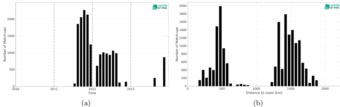
Figure 2: Number of match-ups between Surface drifters and SMOS SSS L4 v1 - Monthly (CMEMS-CNR) SSS as a function of time (a) and as function of the distance to coast (b) over the Gulf Stream Pi-MEP region and for the full satellite product period.
