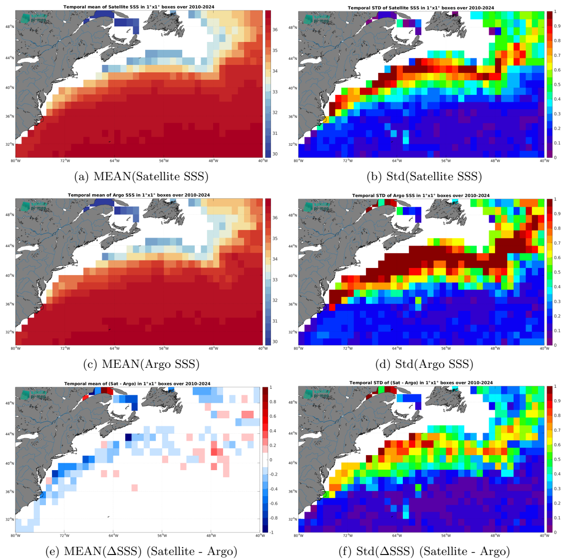
Figure 7: Temporal mean (left) and Std (right) of SSS from SMOS SSS L4 v1 - Monthly (CMEMS-CNR) (top), Argo (middle), and of \Delta SSS (Satellite - Argo). Only match-up pairs are used to generate these maps.
