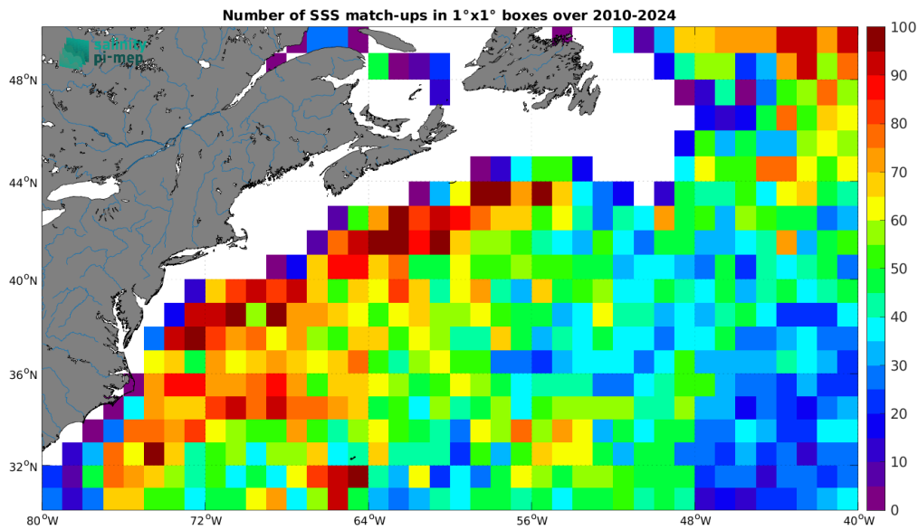
Figure 5: Number of SSS match-ups between Argo SSS and the SMOS SSS L4 v1 - Monthly (CMEMS-CNR) SSS product for the Gulf Stream Pi-MEP region over 1^\circ \times 1^\circ boxes and for the full satellite product period.
