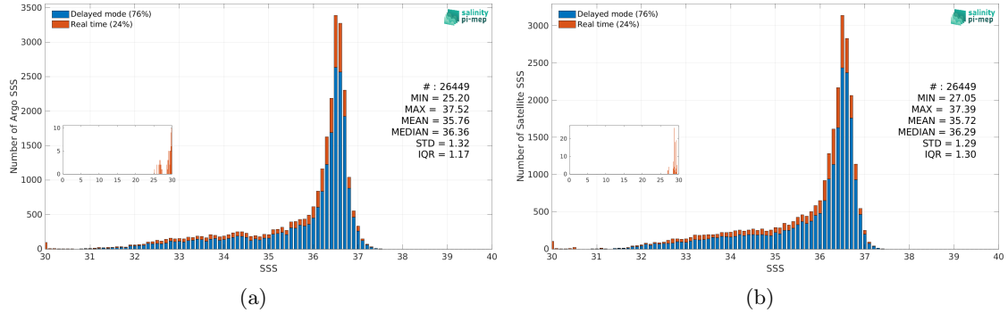
Figure 3: Histograms of SSS from Argo (a) and SMOS SSS L4 v1 - Monthly (CMEMS-CNR) (b) considering all match-up pairs per bins of 0.1 over the Gulf Stream Pi-MEP region and for the full satellite product period.
