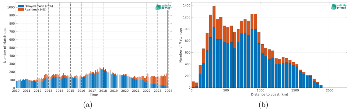
Figure 2: Number of match-ups between Argo and SMOS SSS L4 v1 - Monthly (CMEMS-CNR) SSS as a function of time (a) and as function of the distance to coast (b) over the Gulf Stream Pi-MEP region and for the full satellite product period.
