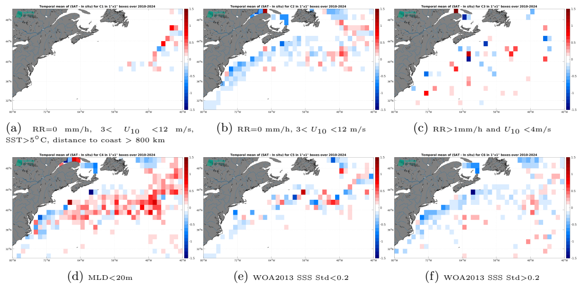
Figure 14: Temporal mean gridded over spatial boxes of size 1^\circ \times 1^\circ of \Delta SSS (SMOS SSS L4 v1 - Monthly (CMEMS-CNR) - Argo) for 6 different subdatasets corresponding to:RR=0 mm/h, 3 < U_{10} < 12 m/s, SST >5^\circ C, distance to coast > 800 km (a), RR=0 mm/h, 3 < U_{10} < 12 m/s (b), RR >1 mm/h and U_{10} < 4 m/s (c),MLD <20 m (d),WOA2013 SSS Std <0.2 (e),WOA2013 SSS Std >0.2 (f).
