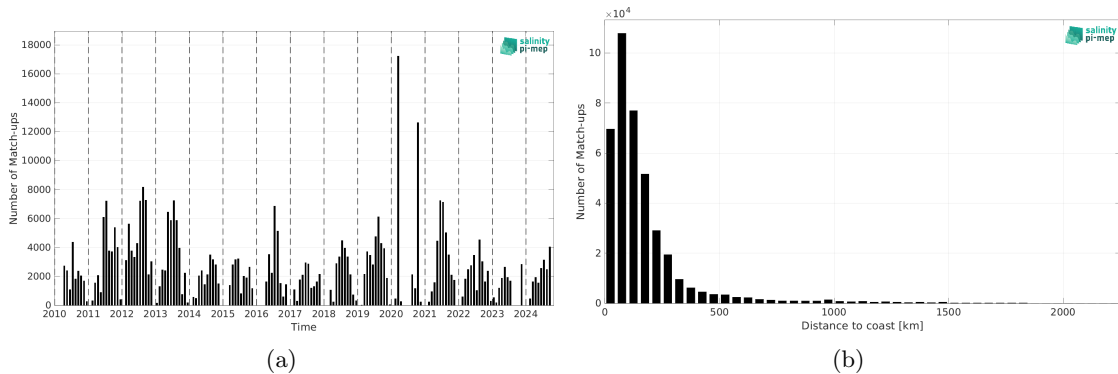
Figure 2: Number of match-ups between TSG (SAMOS) and SMOS SSS L4 v1 - Daily (CMEMS-CNR) SSS as a function of time (a) and as function of the distance to coast (b) over the Gulf Stream Pi-MEP region and for the full satellite product period.
