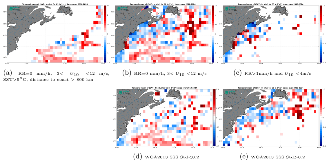
Figure 14: Temporal mean gridded over spatial boxes of size 1^\circ \times 1^\circ of \Delta\text{SSS} (SMOS SSS L4 v1 - Daily (CMEMS-CNR) - TSG (SAMOS)) for 5 different subdatasets corresponding to:RR=0 mm/h, 3 < U_{10} < 12 m/s, SST >5^\circ\text{C} , distance to coast > 800 km (a), RR=0 mm/h, 3 < U_{10} < 12 m/s (b), RR >1 mm/h and U_{10} < 4 m/s (c), WOA2013 SSS Std <0.2 (d), WOA2013 SSS Std >0.2 (e).
