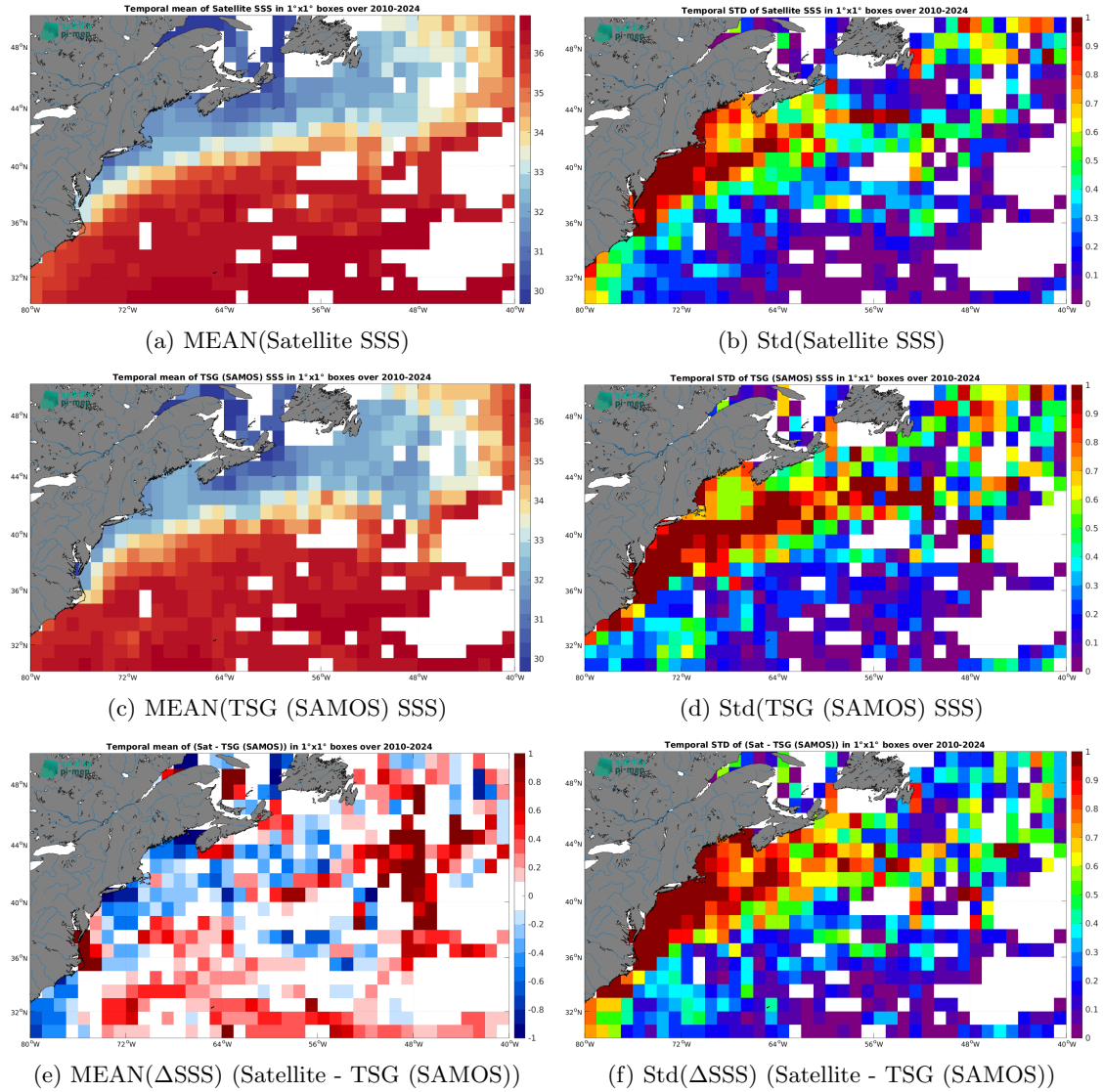
Figure 7: Temporal mean (left) and Std (right) of SSS from SMOS SSS L4 v1 - Daily (CMEMS-CNR) (top), TSG (SAMOS) (middle), and of \Delta SSS (Satellite - TSG (SAMOS)). Only match-up pairs are used to generate these maps.
