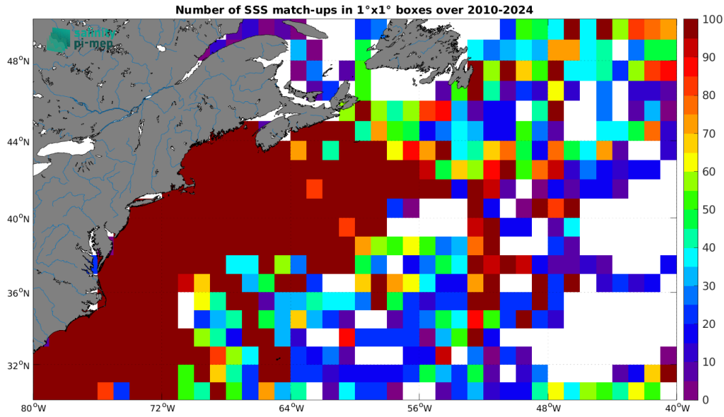
Figure 5: Number of SSS match-ups between TSG (SAMOS) SSS and the SMOS SSS L4 v1 - Daily (CMEMS-CNR) SSS product for the Gulf Stream Pi-MEP region over 1^\circ \times 1^\circ boxes and for the full satellite product period.
