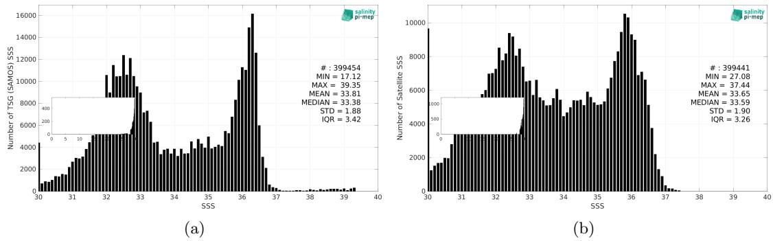
Figure 3: Histograms of SSS from TSG (SAMOS) (a) and SMOS SSS L4 v1 - Daily (CMEMS-CNR) (b) considering all match-up pairs per bins of 0.1 over the Gulf Stream Pi-MEP region and for the full satellite product period.
