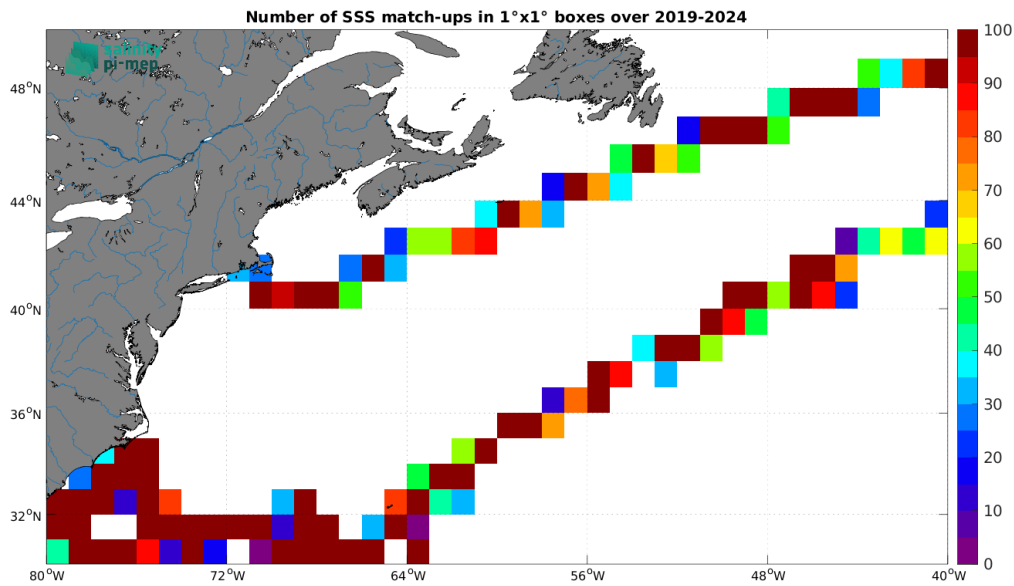
Figure 5: Number of SSS match-ups between Saildrone SSS and the SMOS SSS L4 v1 - Daily (CMEMS-CNR) SSS product for the Gulf Stream Pi-MEP region over 1^\circ \times 1^\circ boxes and for the full satellite product period.
