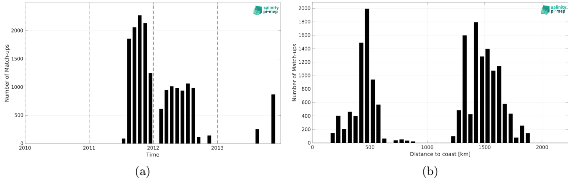
Figure 2: Number of match-ups between Surface drifters and SMOS SSS L4 v1 - Daily (CMEMS-CNR) SSS as a function of time (a) and as function of the distance to coast (b) over the Gulf Stream Pi-MEP region and for the full satellite product period.
