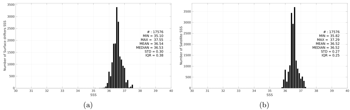
Figure 3: Histograms of SSS from Surface drifters (a) and SMOS SSS L4 v1 - Daily (CMEMS-CNR) (b) considering all match-up pairs per bins of 0.1 over the Gulf Stream Pi-MEP region and for the full satellite product period.
