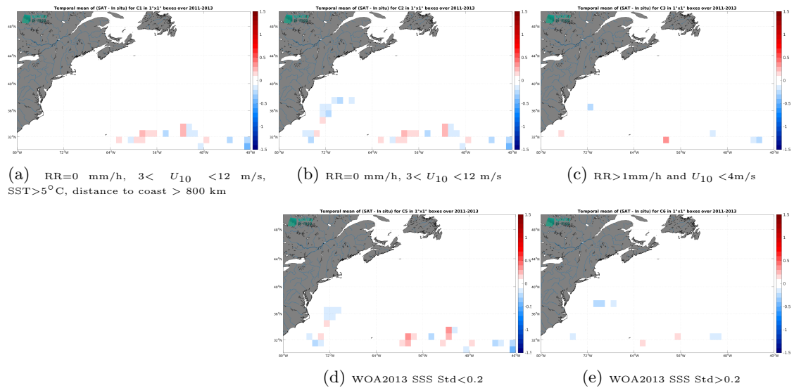
Figure 13: Temporal mean gridded over spatial boxes of size 1^\circ \times 1^\circ of \Delta SSS (SMOS SSS L4 v1 - Daily (CMEMS-CNR) - Surface drifters) for 5 different subdatasets corresponding to:RR=0 mm/h, 3 < U_{10} < 12 m/s, SST >5^\circ C, distance to coast > 800 km (a), RR=0 mm/h, 3 < U_{10} < 12 m/s (b), RR >1 mm/h and U_{10} < 4 m/s (c), WOA2013 SSS Std <0.2 (d), WOA2013 SSS Std >0.2 (e).
