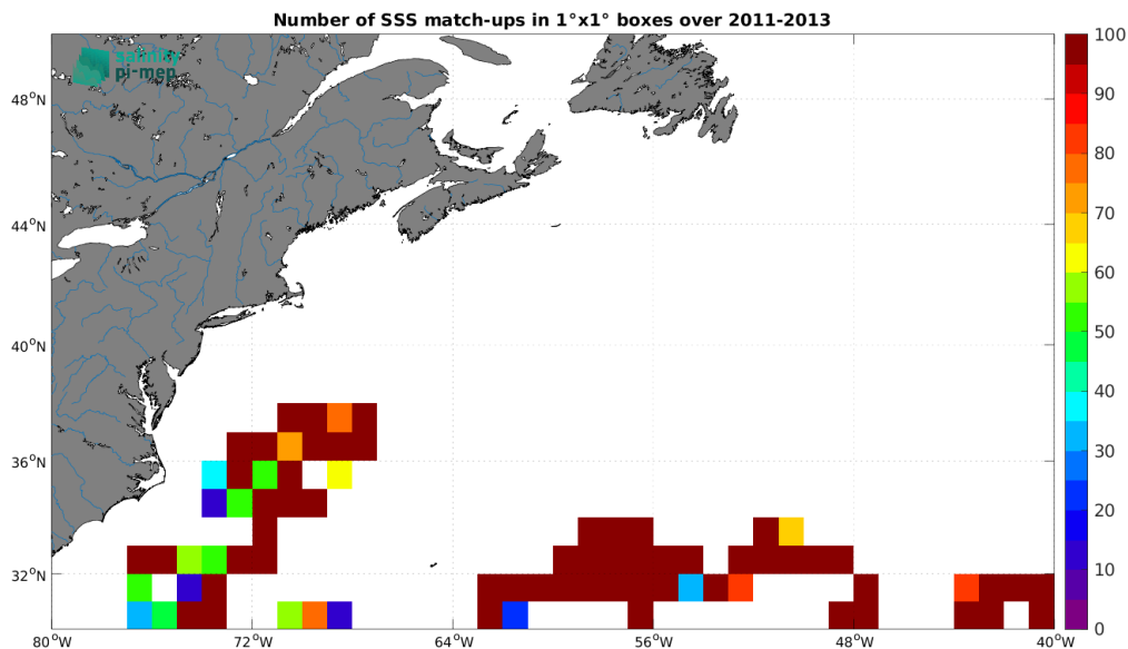
Figure 4: Number of SSS match-ups between Surface drifters SSS and the SMOS SSS L4 v1 - Daily (CMEMS-CNR) SSS product for the Gulf Stream Pi-MEP region over 1^\circ \times 1^\circ boxes and for the full satellite product period.
