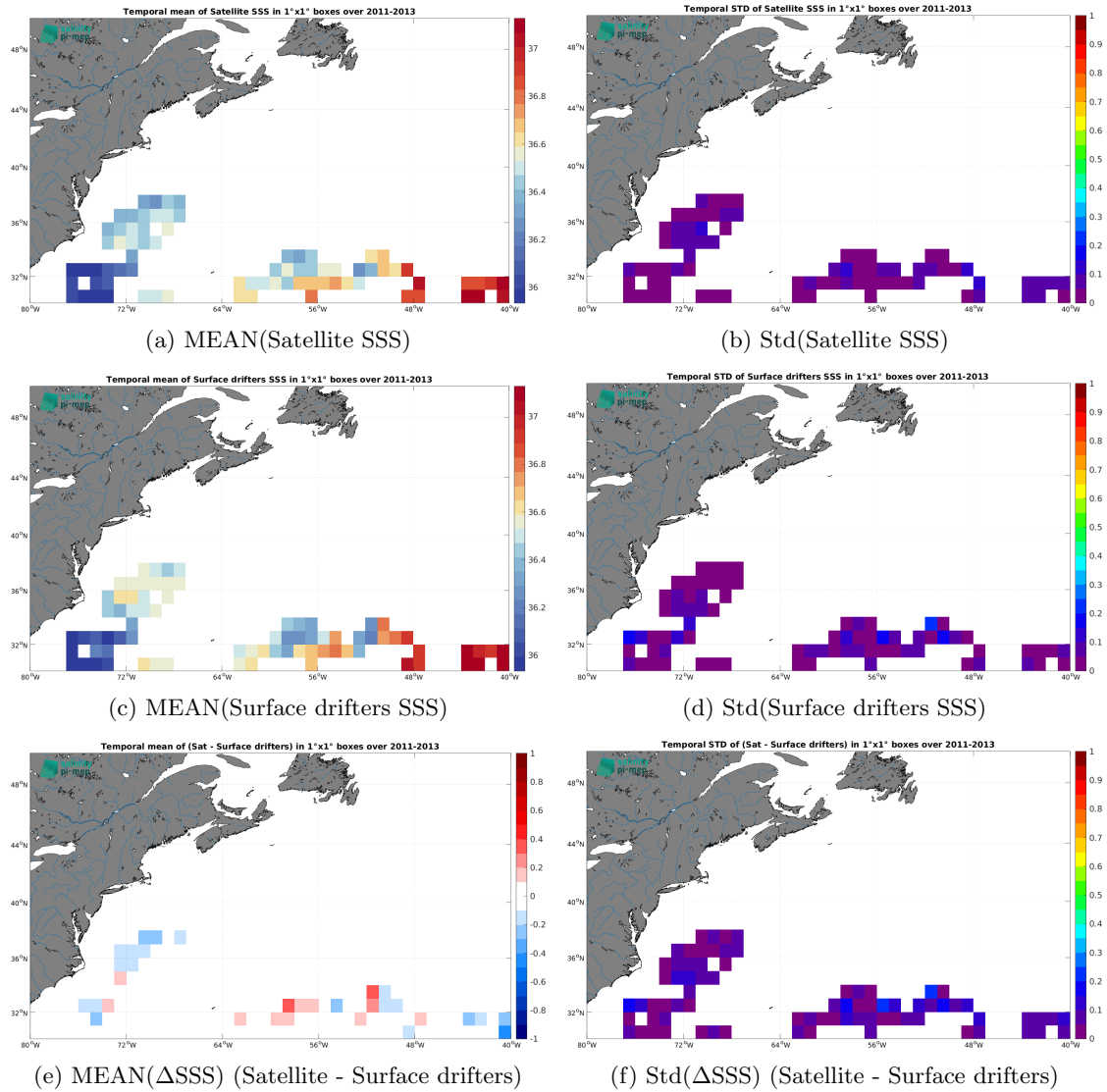
Figure 6: Temporal mean (left) and Std (right) of SSS from SMOS SSS L4 v1 - Daily (CMEMS-CNR) (top), Surface drifters (middle), and of \Delta SSS (Satellite - Surface drifters). Only match-up pairs are used to generate these maps.
