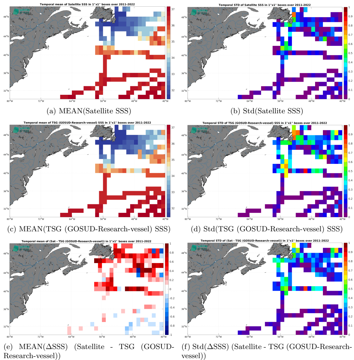
Figure 7: Temporal mean (left) and Std (right) of SSS from SMOS SSS L4 OI v346 - Weekly (CMEMS-CATDS-LOPS) (top), TSG (GOSUD-Research-vessel) (middle), and of \Delta SSS (Satellite - TSG (GOSUD-Research-vessel)). Only match-up pairs are used to generate these maps.
