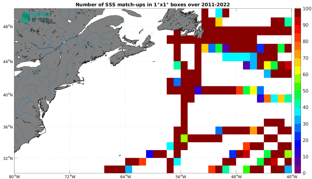
Figure 5: Number of SSS match-ups between TSG (GOSUD-Research-vessel) SSS and the SMOS SSS L4 OI v346 - Weekly (CMEMS-CATDS-LOPS) SSS product for the Gulf Stream Pi-MEP region over 1^\circ \times 1^\circ boxes and for the full satellite product period.
