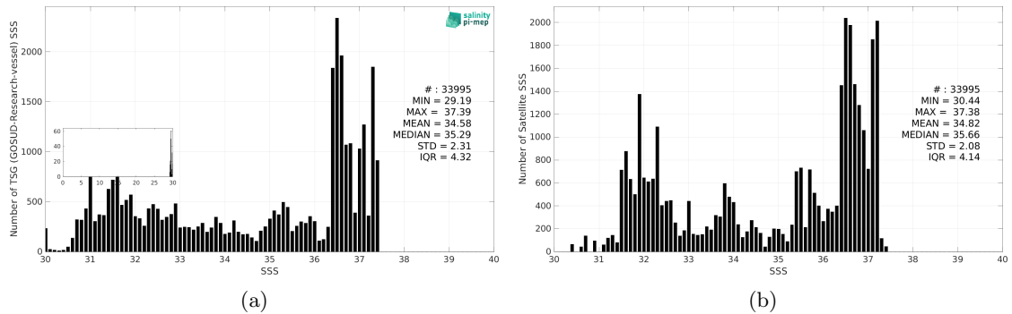
Figure 3: Histograms of SSS from TSG (GOSUD-Research-vessel) (a) and SMOS SSS L4 OI v346 - Weekly (CMEMS-CATDS-LOPS) (b) considering all match-up pairs per bins of 0.1 over the Gulf Stream Pi-MEP region and for the full satellite product period.
