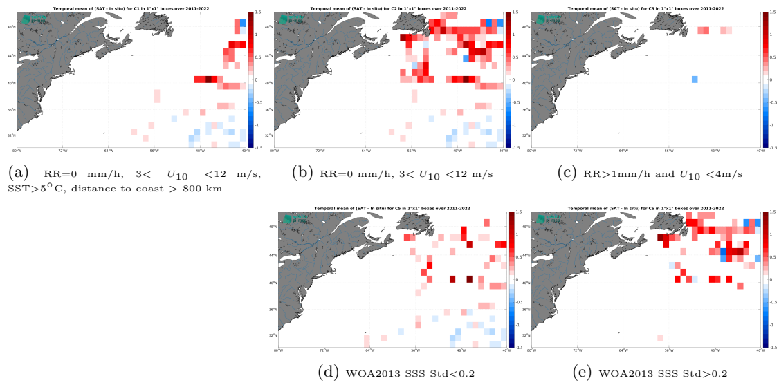
Figure 14: Temporal mean gridded over spatial boxes of size 1^\circ \times 1^\circ of \Delta SSS (SMOS SSS L4 OI v346 - Weekly (CMEMS-CATDS-LOPS) - TSG (GOSUD-Research-vessel)) for 5 different subdatasets corresponding to: RR=0 mm/h, 3 < U_{10} < 12 m/s, SST > 5°C, distance to coast > 800 km (a), RR=0 mm/h, 3 < U_{10} < 12 m/s (b), RR > 1mm/h and U_{10} < 4 m/s (c), WOA2013 SSS Std < 0.2 (d), WOA2013 SSS Std > 0.2 (e).
