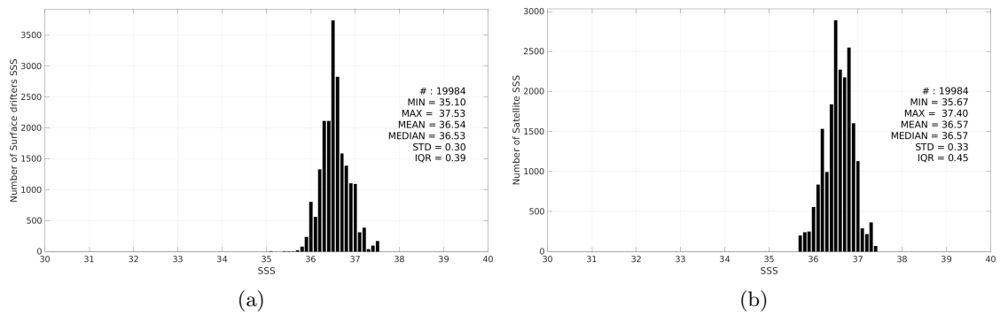
Figure 3: Histograms of SSS from Surface drifters (a) and SMOS SSS L4 OI v346 - Weekly (CMEMS-CATDS-LOPS) (b) considering all match-up pairs per bins of 0.1 over the Gulf Stream Pi-MEP region and for the full satellite product period.
