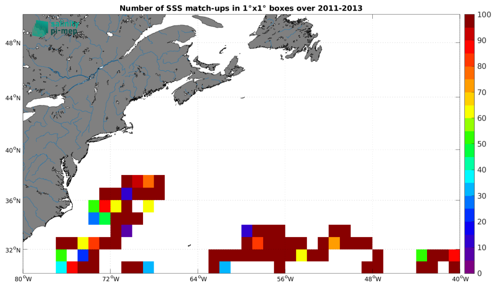
Figure 4: Number of SSS match-ups between Surface drifters SSS and the SMOS SSS L4 OI v346 - Weekly (CMEMS-CATDS-LOPS) SSS product for the Gulf Stream Pi-MEP region over 1^\circ \times 1^\circ boxes and for the full satellite product period.
