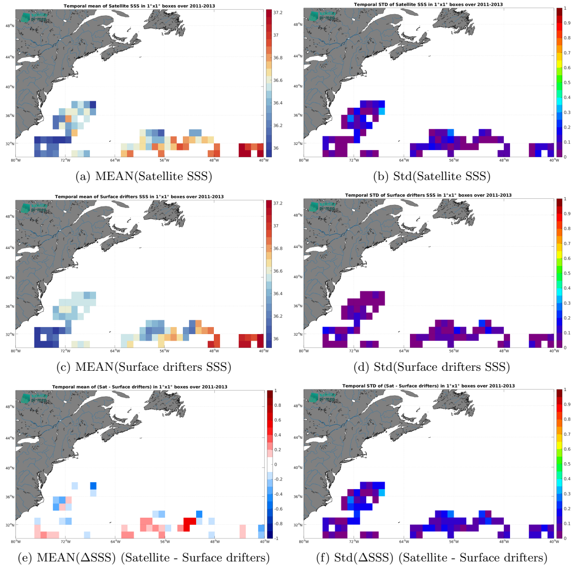
Figure 6: Temporal mean (left) and Std (right) of SSS from SMOS SSS L4 OI v346 - Weekly (CMEMS-CATDS-LOPS) (top), Surface drifters (middle), and of \Delta SSS (Satellite - Surface drifters). Only match-up pairs are used to generate these maps.
