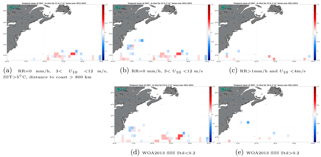
Figure 13: Temporal mean gridded over spatial boxes of size 1^\circ \times 1^\circ of \Delta\text{SSS} (SMOS SSS L4 OI v346 - Weekly (CMEMS-CATDS-LOPS) - Surface drifters) for 5 different subdatasets corresponding to:RR=0 mm/h, 3 < U_{10} < 12 m/s, SST >5^\circ\text{C} , distance to coast > 800 km (a), RR=0 mm/h, 3 < U_{10} < 12 m/s (b), RR >1 mm/h and U_{10} < 4 m/s (c), WOA2013 SSS Std <0.2 (d), WOA2013 SSS Std >0.2 (e).
