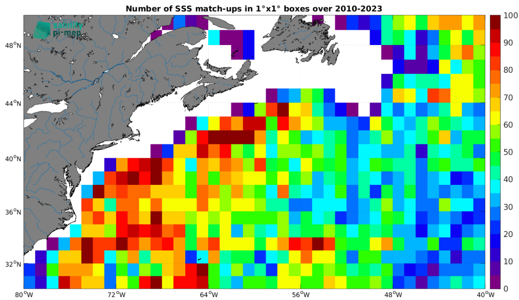
Figure 5: Number of SSS match-ups between Argo SSS and the SMOS SSS L4 OI v346 - Weekly (CMEMS-CATDS-LOPS) SSS product for the Gulf Stream Pi-MEP region over 1^\circ \times 1^\circ boxes and for the full satellite product period.
