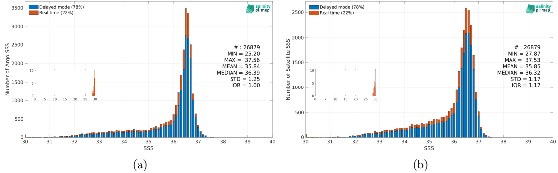
Figure 3: Histograms of SSS from Argo (a) and SMOS SSS L4 OI v346 - Weekly (CMEMS-CATDS-LOPS) (b) considering all match-up pairs per bins of 0.1 over the Gulf Stream Pi-MEP region and for the full satellite product period.
