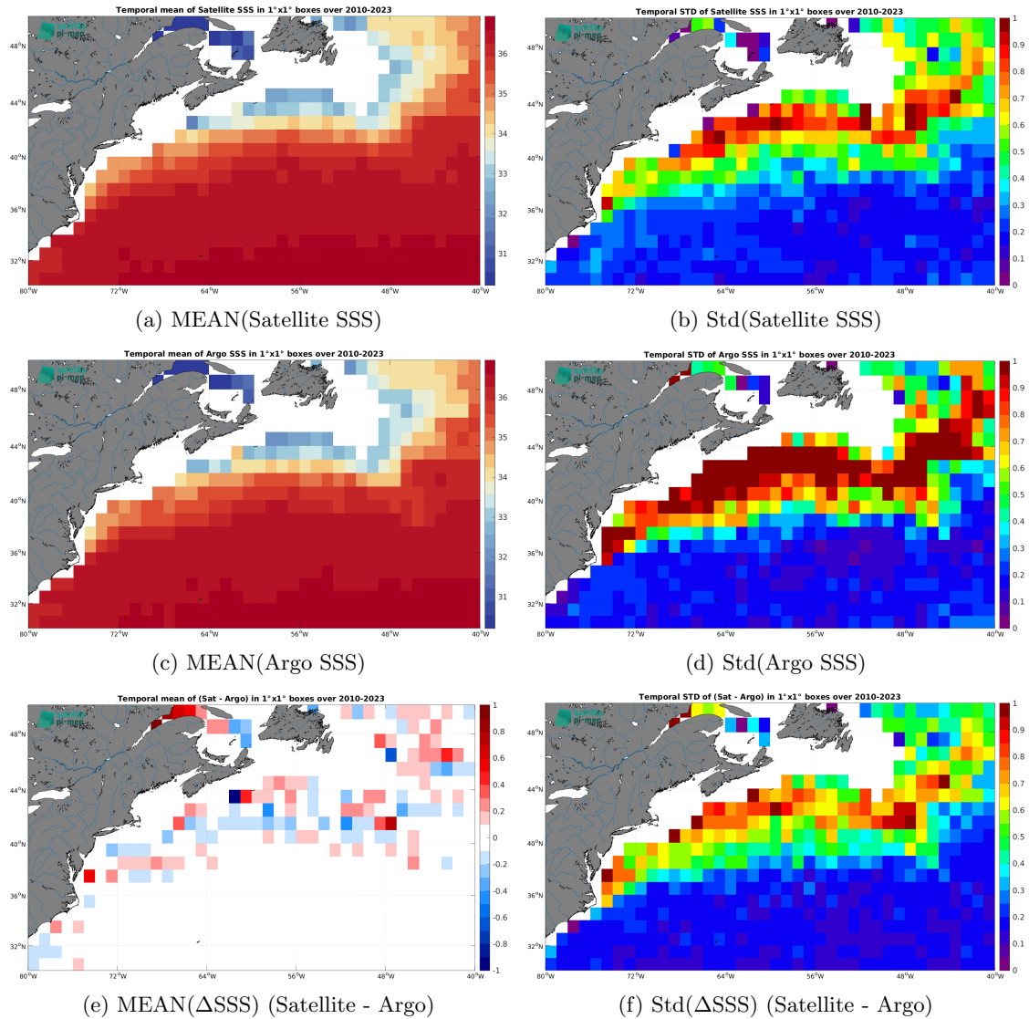
Figure 7: Temporal mean (left) and Std (right) of SSS from SMOS SSS L4 OI v346 - Weekly (CMEMS-CATDS-LOPS) (top), Argo (middle), and of \Delta SSS (Satellite - Argo). Only match-up pairs are used to generate these maps.
