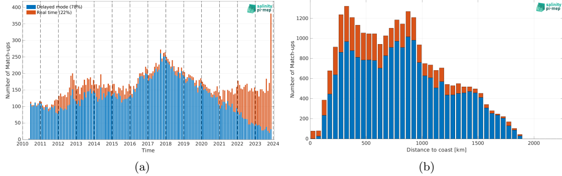
Figure 2: Number of match-ups between Argo and SMOS SSS L4 OI v346 - Weekly (CMEMS-CATDS-LOPS) SSS as a function of time (a) and as function of the distance to coast (b) over the Gulf Stream Pi-MEP region and for the full satellite product period.
