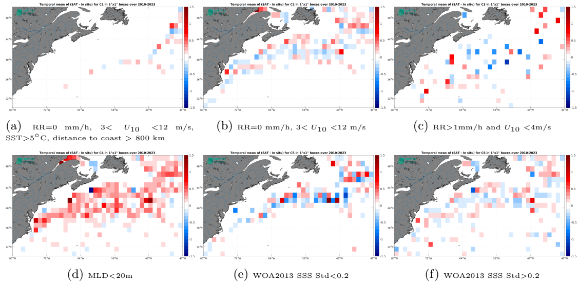
Figure 14: Temporal mean gridded over spatial boxes of size 1^\circ \times 1^\circ of \Delta\text{SSS} (SMOS SSS L4 OI v346 - Weekly (CMEMS-CATDS-LOPS) - Argo) for 6 different subdatasets corresponding to:RR=0 mm/h, 3 < U_{10} < 12 m/s, SST>5°C, distance to coast > 800 km (a), RR=0 mm/h, 3 < U_{10} < 12 m/s (b), RR>1mm/h and U_{10} < 4 m/s (c),MLD<20m (d),WOA2013 SSS Std<0.2 (e),WOA2013 SSS Std>0.2 (f).
