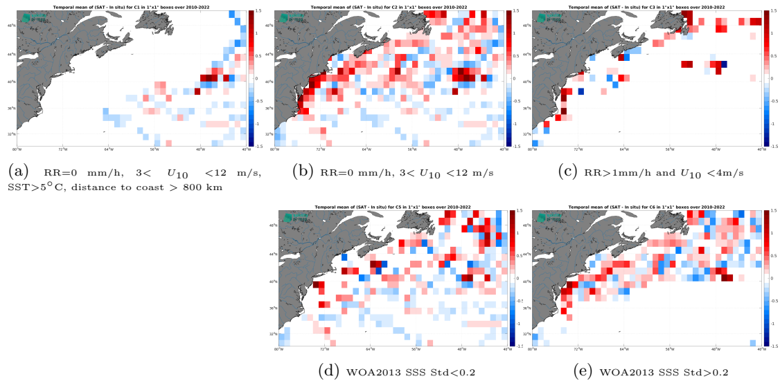
Figure 12: Temporal mean gridded over spatial boxes of size 1^{\circ}\times 1^{\circ} of \Delta\text{SSS} (SMOS SSS L4 OI v342 - Weekly (CMEMS-CATDS-LOPS) - TSG (LEGOS-DM)) for 5 different subdatasets corresponding to:RR=0 mm/h, 3 < U_{10} < 12 m/s, SST >5^{\circ}\text{C} , distance to coast > 800 km (a), RR=0 mm/h, 3 < U_{10} < 12 m/s (b), RR >1 mm/h and U_{10} < 4 m/s (c), WOA2013 SSS Std <0.2 (d), WOA2013 SSS Std >0.2 (e).
