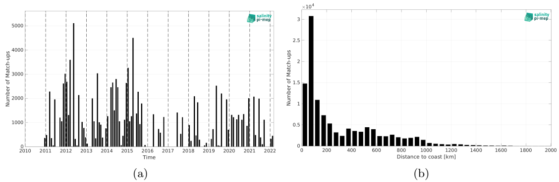
Figure 1: Number of match-ups between TSG (LEGOS-DM) and SMOS SSS L4 OI v342 - Weekly (CMEMS-CATDS-LOPS) SSS as a function of time (a) and as function of the distance to coast (b) over the Gulf Stream Pi-MEP region and for the full satellite product period.
