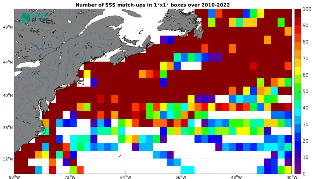
Figure 4: Number of SSS match-ups between TSG (LEGOS-DM) SSS and the SMOS SSS L4 OI v342 - Weekly (CMEMS-CATDS-LOPS) SSS product for the Gulf Stream Pi-MEP region over 1^\circ \times 1^\circ boxes and for the full satellite product period.
