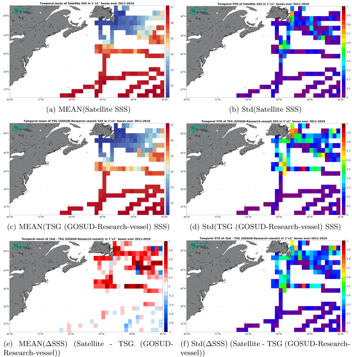
Figure 6: Temporal mean (left) and Std (right) of SSS from SMOS SSS L4 OI v342 - Weekly (CMEMS-CATDS-LOPS) (top), TSG (GOSUD-Research-vessel) (middle), and of \Delta SSS (Satellite - TSG (GOSUD-Research-vessel)). Only match-up pairs are used to generate these maps.
