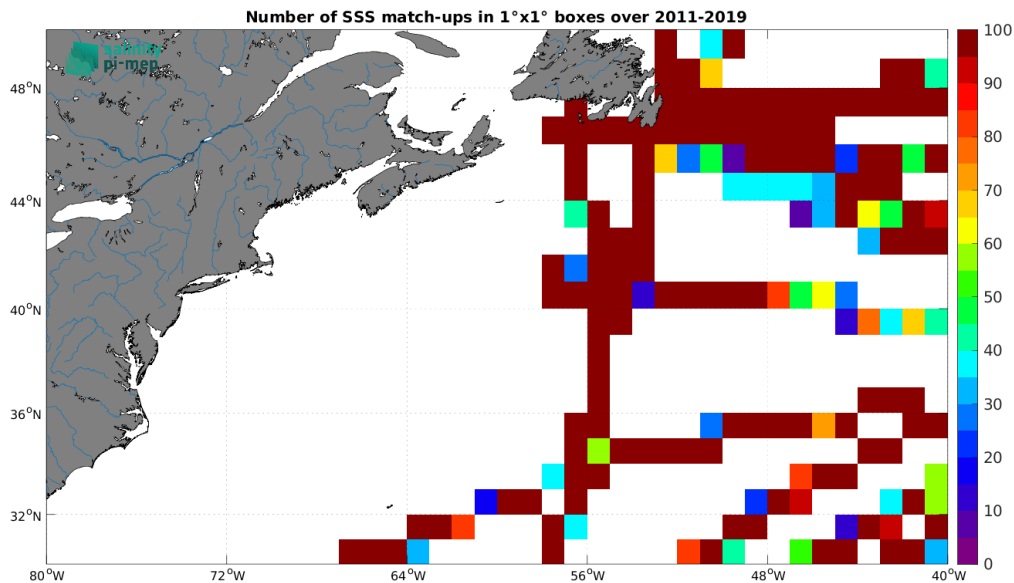
Figure 4: Number of SSS match-ups between TSG (GOSUD-Research-vessel) SSS and the SMOS SSS L4 OI v342 - Weekly (CMEMS-CATDS-LOPS) SSS product for the Gulf Stream Pi-MEP region over 1^\circ \times 1^\circ boxes and for the full satellite product period.
