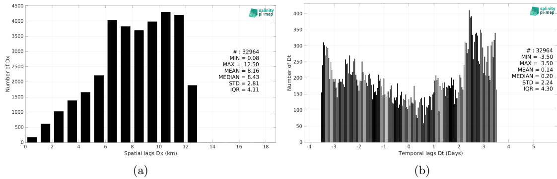
Figure 5: Histograms of the spatial (a) and temporal (b) lags between the location/time of the TSG (GOSUD-Research-vessel) measurement and the date of the corresponding SMOS SSS L4 OI v342 - Weekly (CMEMS-CATDS-LOPS) SSS pixel.
