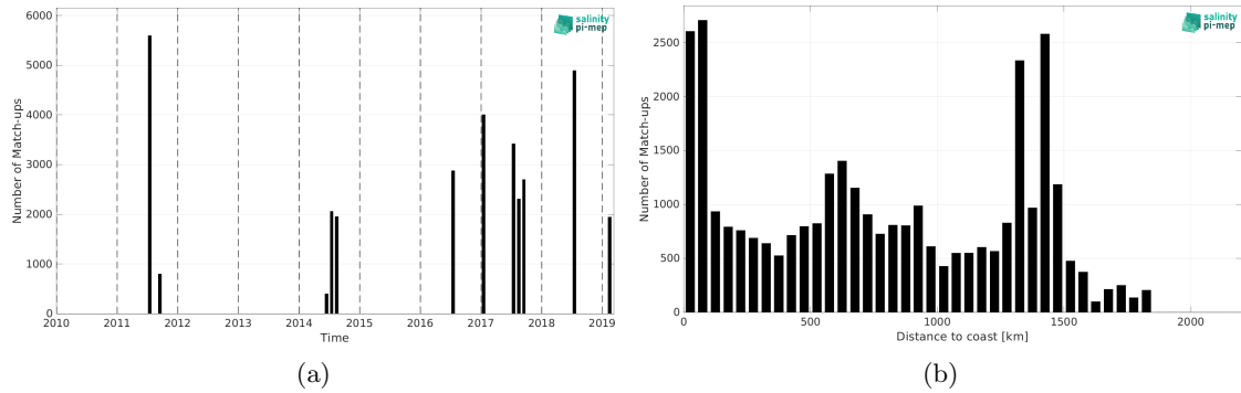
Figure 1: Number of match-ups between TSG (GOSUD-Research-vessel) and SMOS SSS L4 OI v342 - Weekly (CMEMS-CATDS-LOPS) SSS as a function of time (a) and as function of the distance to coast (b) over the Gulf Stream Pi-MEP region and for the full satellite product period.
