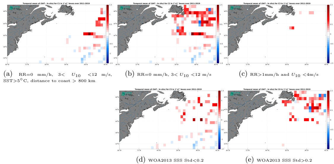
Figure 12: Temporal mean gridded over spatial boxes of size 1^{\circ}\times 1^{\circ} of \Delta SSS (SMOS SSS L4 OI v342 - Weekly (CMEMS-CATDS-LOPS) - TSG (GOSUD-Research-vessel)) for 5 different subdatasets corresponding to:RR=0 mm/h, 3 < U_{10} < 12 m/s, SST >5^{\circ}\text{C} , distance to coast > 800 km (a), RR=0 mm/h, 3 < U_{10} < 12 m/s (b), RR >1 mm/h and U_{10} < 4 m/s (c), WOA2013 SSS Std <0.2 (d), WOA2013 SSS Std >0.2 (e).
