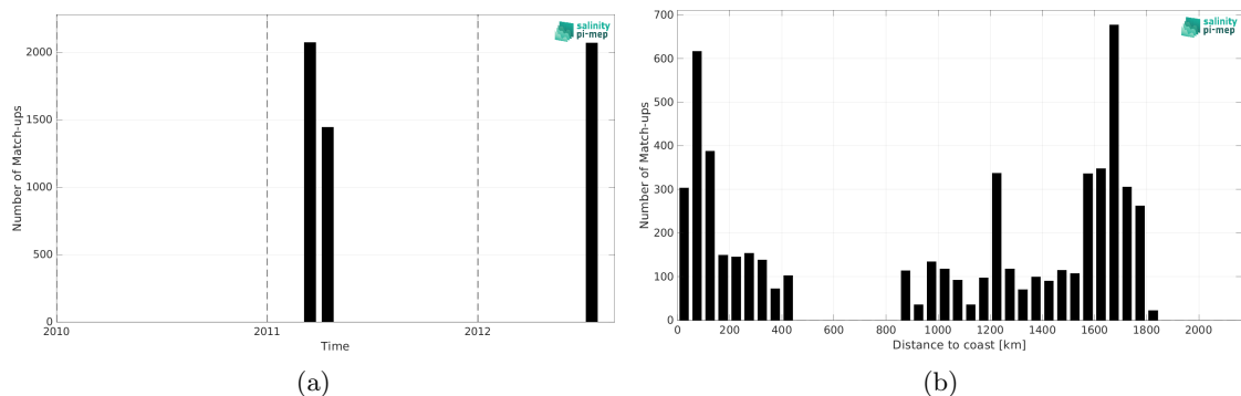
Figure 1: Number of match-ups between TSG (CSIC-UTM) and SMOS SSS L4 OI v342 - Weekly (CMEMS-CATDS-LOPS) SSS as a function of time (a) and as function of the distance to coast (b) over the Gulf Stream Pi-MEP region and for the full satellite product period.
