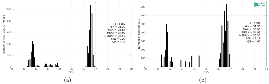
Figure 2: Histograms of SSS from TSG (CSIC-UTM) (a) and SMOS SSS L4 OI v342 - Weekly (CMEMS-CATDS-LOPS) (b) considering all match-up pairs per bins of 0.1 over the Gulf Stream Pi-MEP region and for the full satellite product period.
