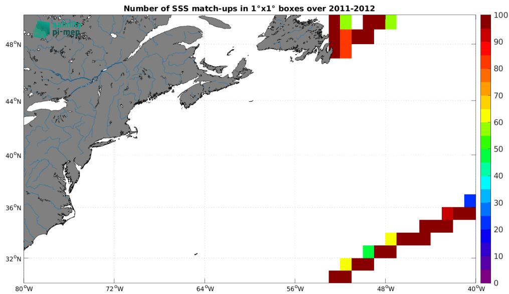
Figure 4: Number of SSS match-ups between TSG (CSIC-UTM) SSS and the SMOS SSS L4 OI v342 - Weekly (CMEMS-CATDS-LOPS) SSS product for the Gulf Stream Pi-MEP region over 1^\circ \times 1^\circ boxes and for the full satellite product period.
