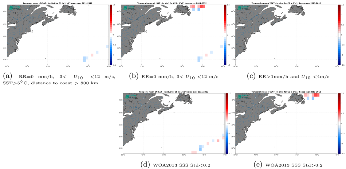
Figure 12: Temporal mean gridded over spatial boxes of size 1^{\circ}\times 1^{\circ} of \Delta\text{SSS} (SMOS SSS L4 OI v342 - Weekly (CMEMS-CATDS-LOPS) - TSG (CSIC-UTM)) for 5 different subdatasets corresponding to:RR=0 mm/h, 3 < U_{10} < 12 m/s, SST >5^{\circ}\text{C} , distance to coast > 800 km (a), RR=0 mm/h, 3 < U_{10} < 12 m/s (b), RR >1 mm/h and U_{10} < 4 m/s (c), WOA2013 SSS Std <0.2 (d), WOA2013 SSS Std >0.2 (e).
