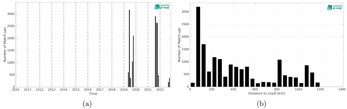
Figure 1: Number of match-ups between Saildrone and SMOS SSS L4 OI v342 - Weekly (CMEMS-CATDS-LOPS) SSS as a function of time (a) and as function of the distance to coast (b) over the Gulf Stream Pi-MEP region and for the full satellite product period.
