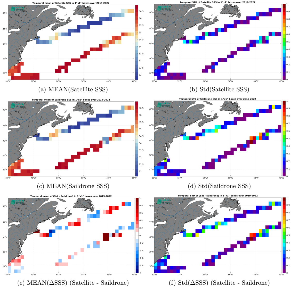
Figure 6: Temporal mean (left) and Std (right) of SSS from SMOS SSS L4 OI v342 - Weekly (CMEMS-CATDS-LOPS) (top), Saildrone (middle), and of \Delta SSS (Satellite - Saildrone). Only match-up pairs are used to generate these maps.
