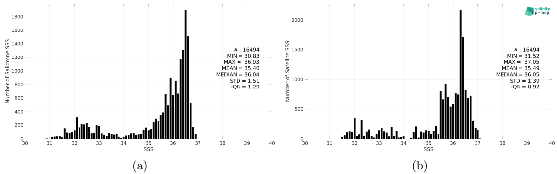
Figure 2: Histograms of SSS from Saildrone (a) and SMOS SSS L4 OI v342 - Weekly (CMEMS-CATDS-LOPS) (b) considering all match-up pairs per bins of 0.1 over the Gulf Stream Pi-MEP region and for the full satellite product period.
