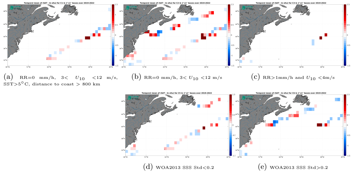
Figure 12: Temporal mean gridded over spatial boxes of size 1^\circ \times 1^\circ of \Delta SSS (SMOS SSS L4 OI v342 - Weekly (CMEMS-CATDS-LOPS) - Saildrone) for 5 different subdatasets corresponding to:RR=0 mm/h, 3 < U_{10} < 12 m/s, SST >5^\circ\text{C} , distance to coast > 800 km (a), RR=0 mm/h, 3 < U_{10} < 12 m/s (b), RR >1 mm/h and U_{10} < 4 m/s (c), WOA2013 SSS Std <0.2 (d), WOA2013 SSS Std >0.2 (e).
