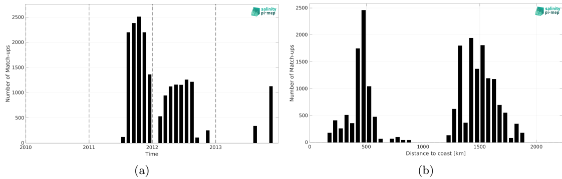
Figure 1: Number of match-ups between Surface drifters and SMOS SSS L4 OI v342 - Weekly (CMEMS-CATDS-LOPS) SSS as a function of time (a) and as function of the distance to coast (b) over the Gulf Stream Pi-MEP region and for the full satellite product period.
