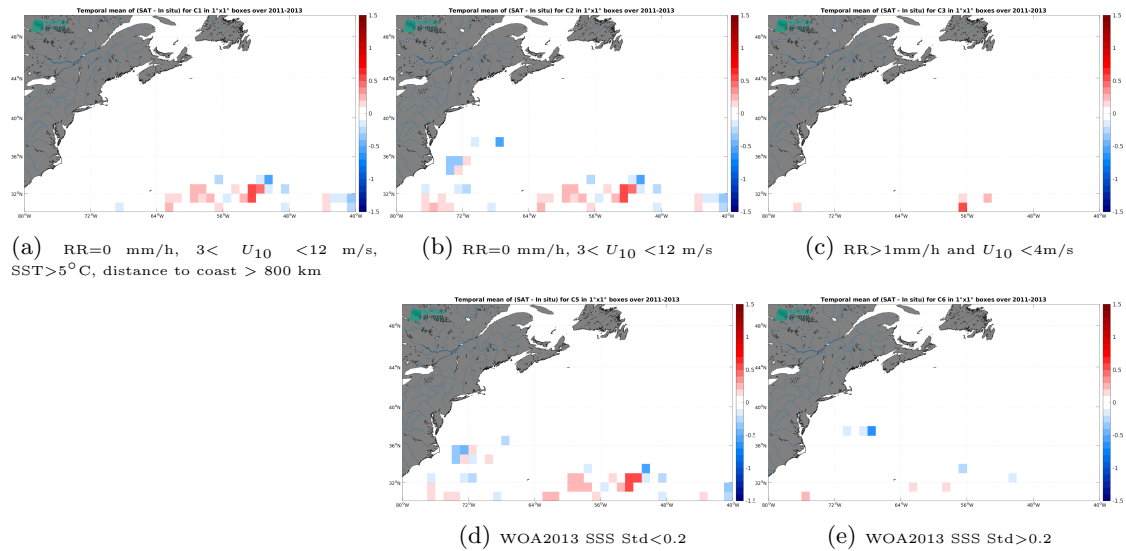
Figure 11: Temporal mean gridded over spatial boxes of size 1^{\circ}\times 1^{\circ} of \Delta\text{SSS} (SMOS SSS L4 OI v342 - Weekly (CMEMS-CATDS-LOPS) - Surface drifters) for 5 different subdatasets corresponding to:RR=0 mm/h, 3 < U_{10} < 12 m/s, SST >5^{\circ}\text{C} , distance to coast > 800 km (a), RR=0 mm/h, 3 < U_{10} < 12 m/s (b), RR >1 mm/h and U_{10} < 4 m/s (c), WOA2013 SSS Std <0.2 (d), WOA2013 SSS Std >0.2 (e).
