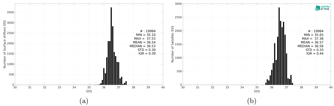
Figure 2: Histograms of SSS from Surface drifters (a) and SMOS SSS L4 OI v342 - Weekly (CMEMS-CATDS-LOPS) (b) considering all match-up pairs per bins of 0.1 over the Gulf Stream Pi-MEP region and for the full satellite product period.
