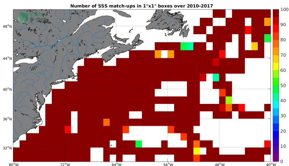
Figure 4: Number of SSS match-ups between TSG-SAMOS SSS and the SMOS-L4-CATDS-CECOS-IFREMER-V2-WEEKLY-0.5DEG SSS product for the Gulf Stream Pi-MEP region over 1°x1° boxes and for the full satellite product period.
