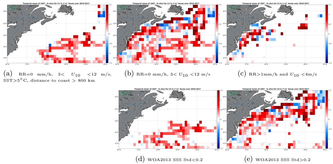
Figure 12: Temporal mean gridded over spatial boxes of size 1^\circ \times 1^\circ of \Delta SSS (SMOS-L4-CATDS-CECOS-IFREMER-V2-WEEKLY-0.5DEG - TSG-SAMOS) for 5 different subdatasets corresponding to: RR=0 mm/h, 3 < U_{10} < 12 m/s, SST > 5^\circ C , distance to coast > 800 km (a), RR=0 mm/h, 3 < U_{10} < 12 m/s (b), RR > 1 mm/h and U_{10} < 4 m/s (c), WOA2013 SSS Std < 0.2 (d), WOA2013 SSS Std > 0.2 (e).
