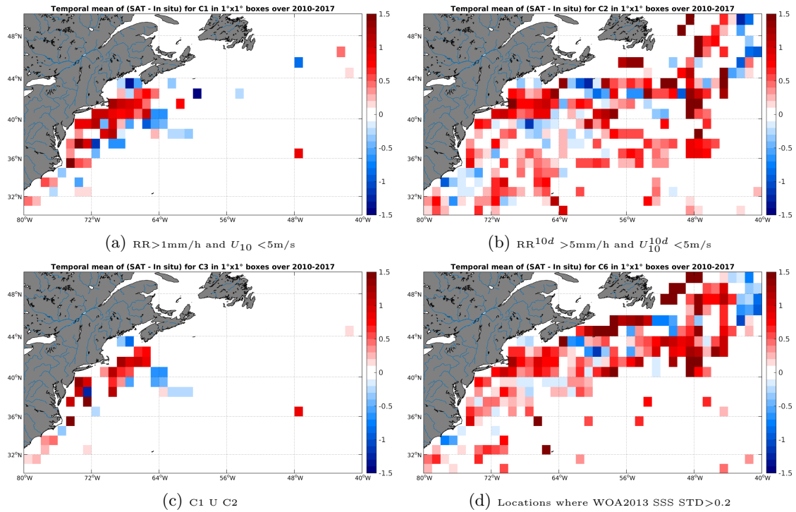
Figure 12: Temporal mean gridded over spatial boxes of size 1^\circ \times 1^\circ of \Delta SSS (SMOS-L4-CATDS-CECOS-IFREMER-V2-WEEKLY-0.5DEG - TSG-SAMOS) for 4 different subdatasets corresponding to: RR > 1\text{mm/h} and U_{10} < 5\text{m/s} (a), RR^{10d} > 5\text{mm/h} and U_{10}^{10d} < 5\text{m/s} (b), C1 U C2 (c), Locations where WOA2013 SSS STD > 0.2 (d).
