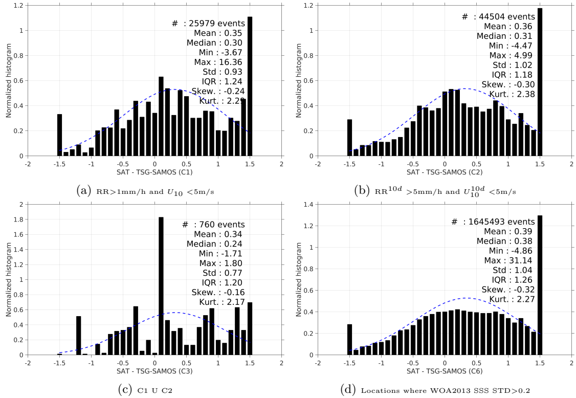
Figure 13: Normalized histogram of \Delta\text{SSS} (SMOS-L4-CATDS-CECOS-IFREMER-V2-WEEKLY-0.5DEG - TSG-SAMOS) for 6 different subdatasets corresponding to: RR>1mm/h and U_{10} < 5\text{m/s} (a), RR^{10d} > 5\text{mm/h} and U_{10}^{10d} < 5\text{m/s} (b), C1 U C2 (c), Locations where WOA2013 SSS STD>0.2 (d).
