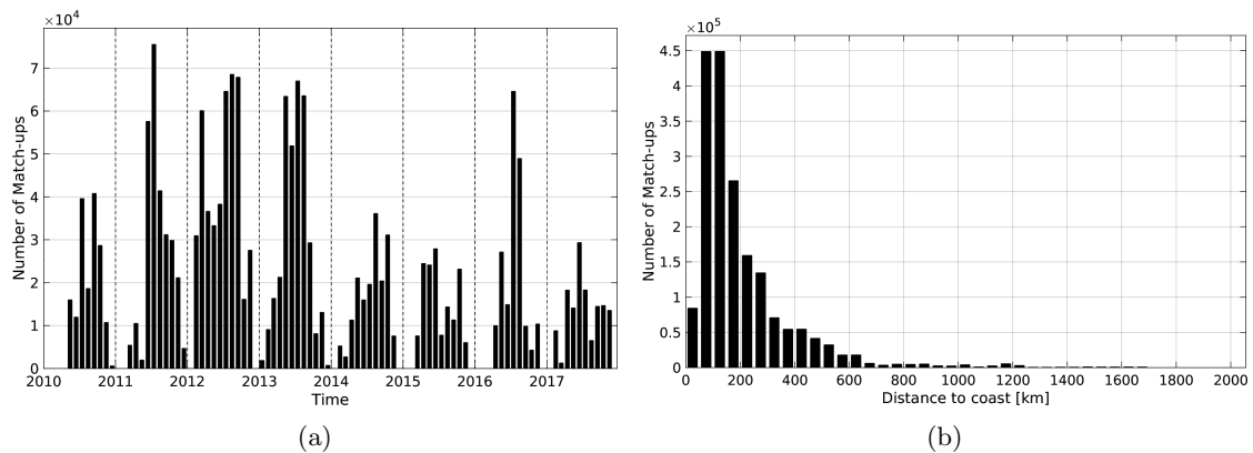
Figure 1: Number of match-ups between TSG-SAMOS and SMOS-L4-CATDS-CECOS-IFREMER-V2-WEEKLY-0.5DEG SSS as a function of time (a) and as function of the distance to coast (b) over the Gulf Stream Pi-MEP region and for the full satellite product period.
