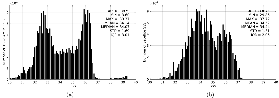
Figure 2: Histograms of SSS from TSG-SAMOS (a) and SMOS-L4-CATDS-CECOS-IFREMER-V2-WEEKLY-0.5DEG (b) considering all match-up pairs per bins of 0.1 over the Gulf Stream Pi-MEP region and for the full satellite product period.
