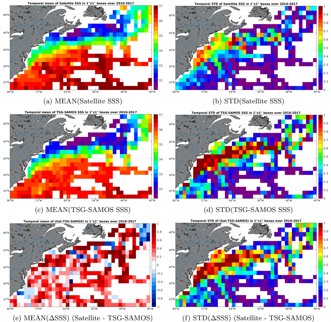
Figure 6: Temporal mean (left) and STD (right) of SSS from SMOS-L4-CATDS-CECOS-IFREMER-V2-WEEKLY-0.5DEG (top), TSG-SAMOS (middle), and of \Delta SSS (Satellite - TSG-SAMOS). Only match-up pairs are used to generate these maps.
