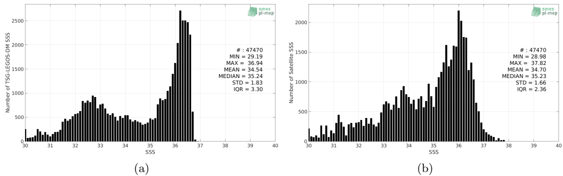
Figure 2: Histograms of SSS from TSG-LEGOS-DM (a) and SMOS-L4-CATDS-CECOS-IFREMER-V2-WEEKLY-0.5DEG (b) considering all match-up pairs per bins of 0.1 over the Gulf Stream Pi-MEP region and for the full satellite product period.
