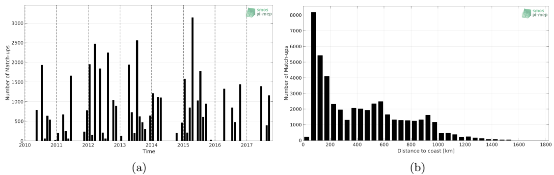
Figure 1: Number of match-ups between TSG-LEGOS-DM and SMOS-L4-CATDS-CECOS-IFREMER-V2-WEEKLY-0.5DEG SSS as a function of time (a) and as function of the distance to coast (b) over the Gulf Stream Pi-MEP region and for the full satellite product period.
