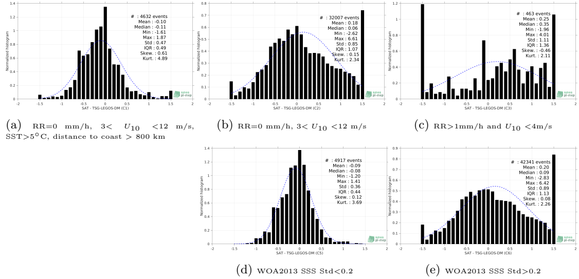
Figure 13: Normalized histogram of \Delta\text{SSS} (SMOS-L4-CATDS-CECOS-IFREMER-V2-WEEKLY-0.5DEG - TSG-LEGOS-DM) for 5 different subdatasets corresponding to: RR=0 mm/h, 3 < U_{10} < 12 m/s, SST>5°C, distance to coast > 800 km (a), RR=0 mm/h, 3 < U_{10} < 12 m/s (b), RR>1mm/h and U_{10} < 4 m/s (c), WOA2013 SSS Std<0.2 (d), WOA2013 SSS Std>0.2 (e).
