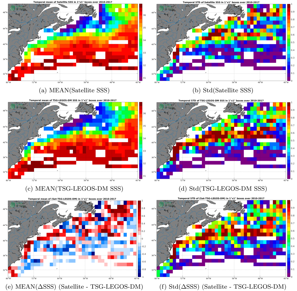
Figure 6: Temporal mean (left) and Std (right) of SSS from SMOS-L4-CATDS-CECOS-IFREMER-V2-WEEKLY-0.5DEG (top), TSG-LEGOS-DM (middle), and of \Delta\text{SSS} (Satellite - TSG-LEGOS-DM). Only match-up pairs are used to generate these maps.
