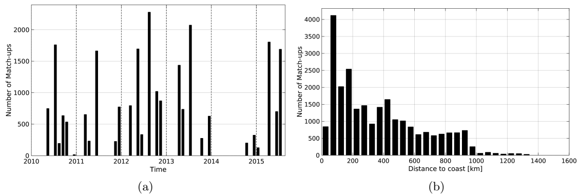
Figure 1: Number of match-ups between TSG-LEGOS-DM and SMOS-L4-CATDS-CECOS-IFREMER-V2-WEEKLY-0.5DEG SSS as a function of time (a) and as function of the distance to coast (b) over the Gulf Stream Pi-MEP region and for the full satellite product period.
