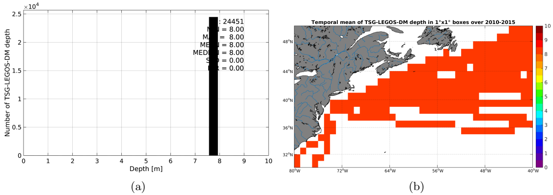
Figure 3: Histograms of the depth of the upper level SSS measurements from TSG-LEGOS-DM in the Match-up DataBase for the Gulf Stream Pi-MEP region (a) and temporal mean spatial distribution of pressure of the in situ SSS data over 1^\circ \times 1^\circ boxes and for the full satellite product period (b).
