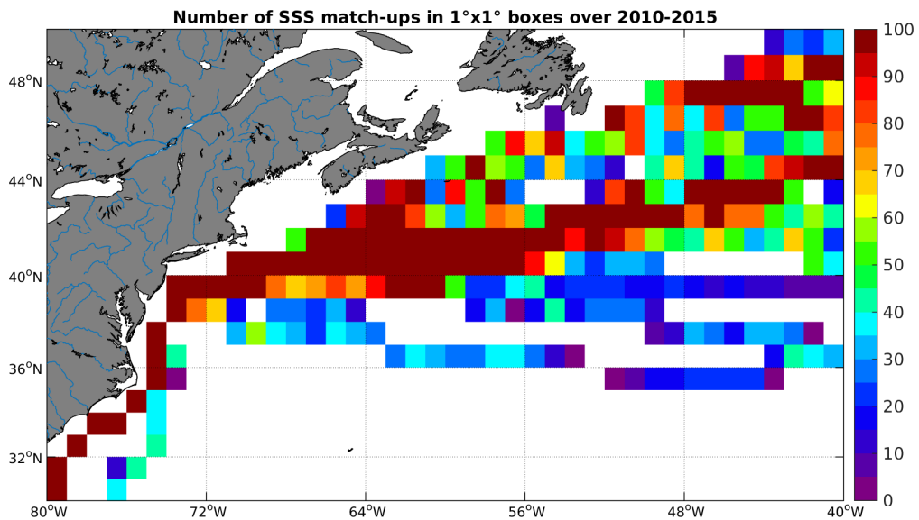
Figure 4: Number of SSS match-ups between TSG-LEGOS-DM SSS and the SMOS-L4-CATDS-CECOS-IFREMER-V2-WEEKLY-0.5DEG SSS product for the Gulf Stream Pi-MEP region over 1^\circ \times 1^\circ boxes and for the full satellite product period.
