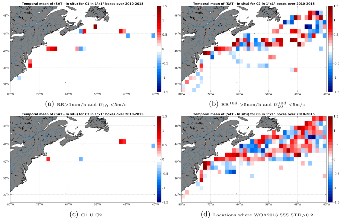
Figure 12: Temporal mean gridded over spatial boxes of size 1^\circ \times 1^\circ of \Delta SSS (SMOS-L4-CATDS-CECOS-IFREMER-V2-WEEKLY-0.5DEG - TSG-LEGOS-DM) for 4 different subdatasets corresponding to:RR>1mm/h and U_{10} < 5\text{m/s} (a), RR^{10d} > 5\text{mm/h} and U_{10}^{10d} < 5\text{m/s} (b), C1 U C2 (c),Locations where WOA2013 SSS STD>0.2 (d).
