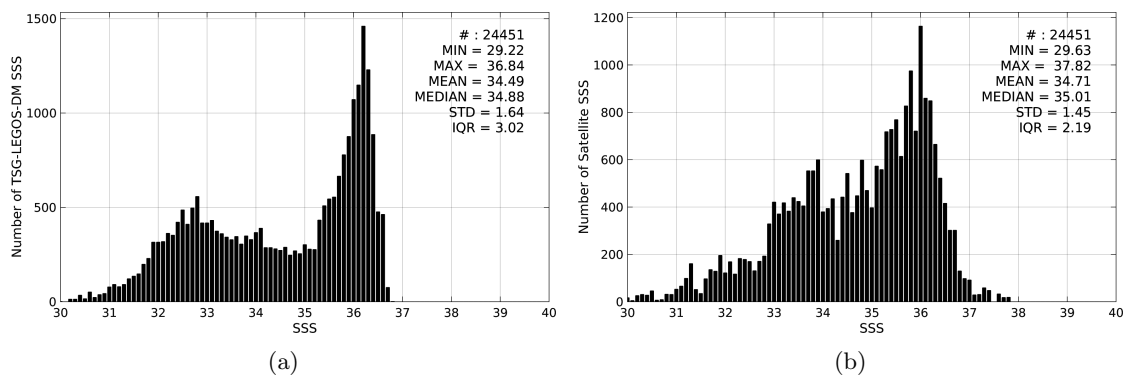
Figure 2: Histograms of SSS from TSG-LEGOS-DM (a) and SMOS-L4-CATDS-CECOS-IFREMER-V2-WEEKLY-0.5DEG (b) considering all match-up pairs per bins of 0.1 over the Gulf Stream Pi-MEP region and for the full satellite product period.
