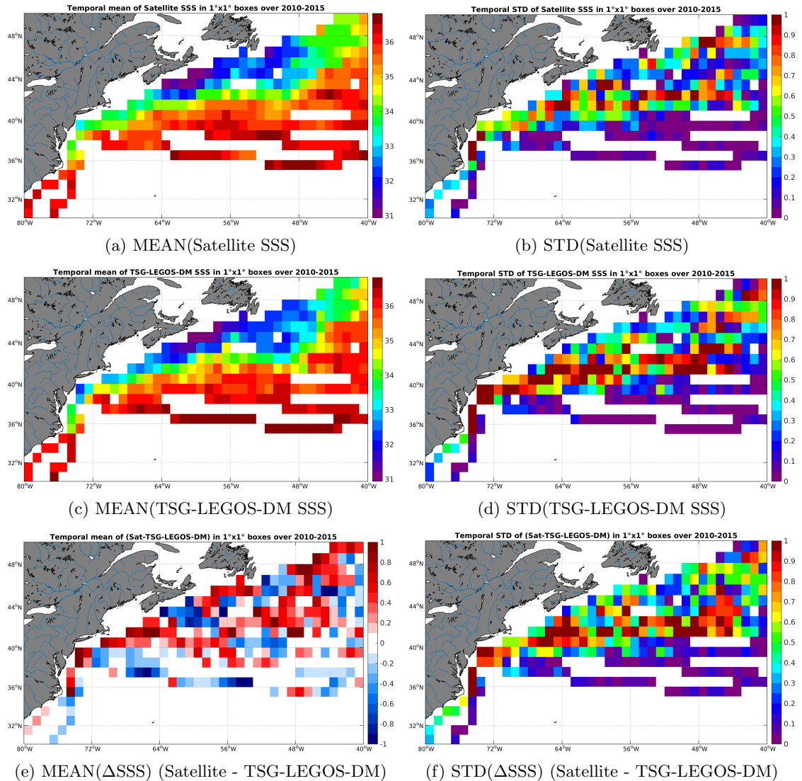
Figure 6: Temporal mean (left) and STD (right) of SSS from SMOS-L4-CATDS-CECOS-IFREMER-V2-WEEKLY-0.5DEG (top), TSG-LEGOS-DM (middle), and of \Delta SSS (Satellite - TSG-LEGOS-DM). Only match-up pairs are used to generate these maps.
