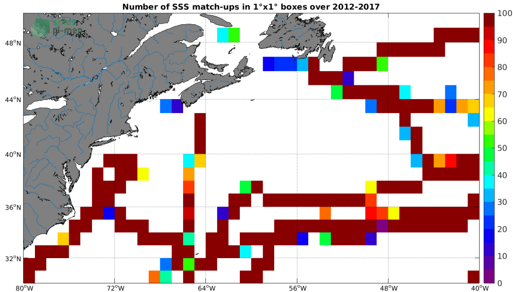
Figure 4: Number of SSS match-ups between TSG (GOSUD-Sailing-ship) SSS and the SMOS L4 v2 Weekly (CATDS-CECOS-IFREMER) SSS product for the Gulf Stream Pi-MEP region over 1^\circ \times 1^\circ boxes and for the full satellite product period.
