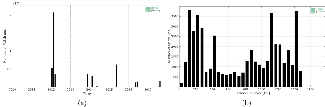
Figure 1: Number of match-ups between TSG (GOSUD-Sailing-ship) and SMOS L4 v2 Weekly (CATDS-CECOS-IFREMER) SSS as a function of time (a) and as function of the distance to coast (b) over the Gulf Stream Pi-MEP region and for the full satellite product period.
