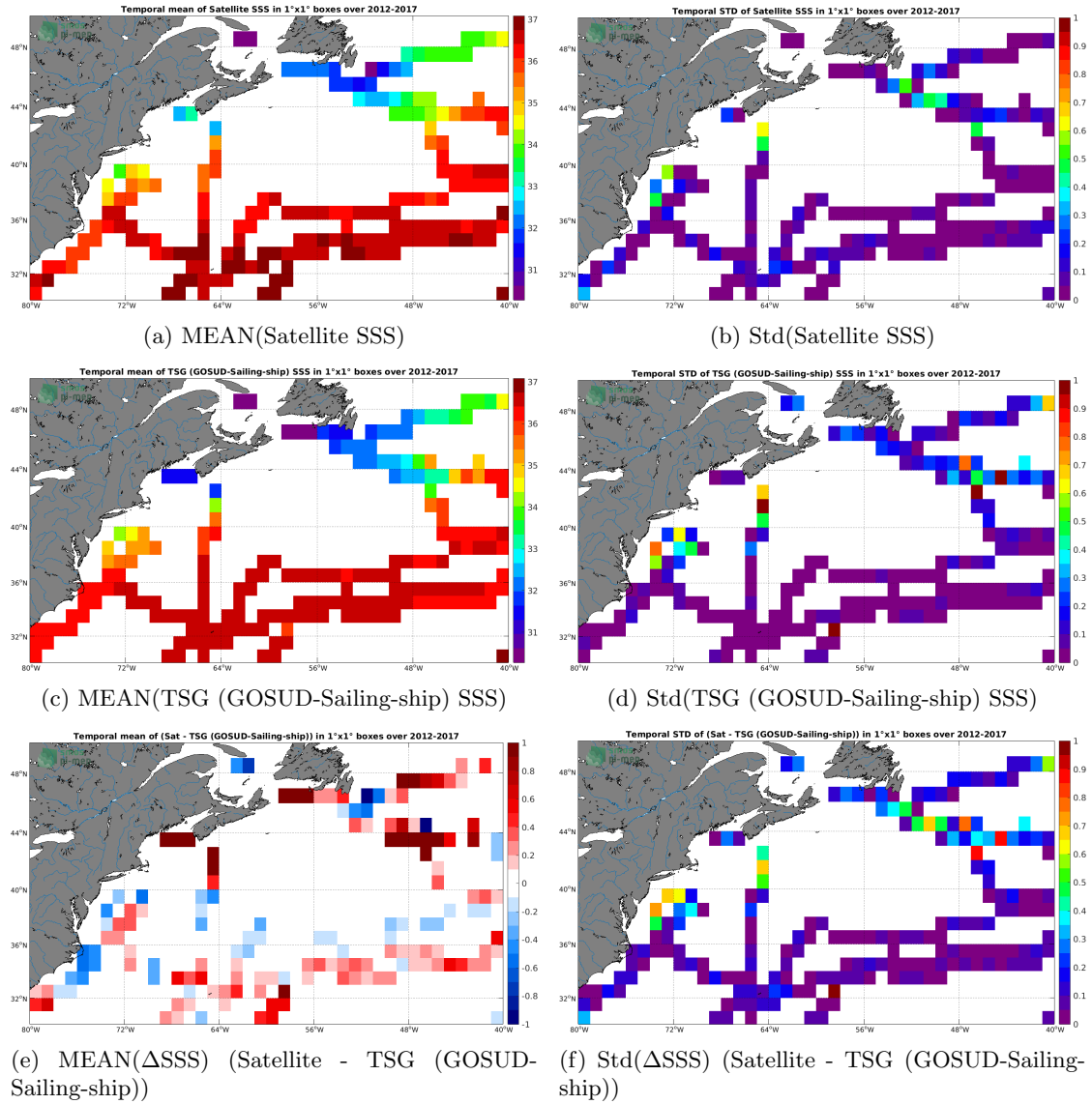
Figure 6: Temporal mean (left) and Std (right) of SSS from SMOS L4 v2 Weekly (CATDS-CECOS-IFREMER) (top), TSG (GOSUD-Sailing-ship) (middle), and of \Delta\text{SSS} (Satellite - TSG (GOSUD-Sailing-ship)). Only match-up pairs are used to generate these maps.
