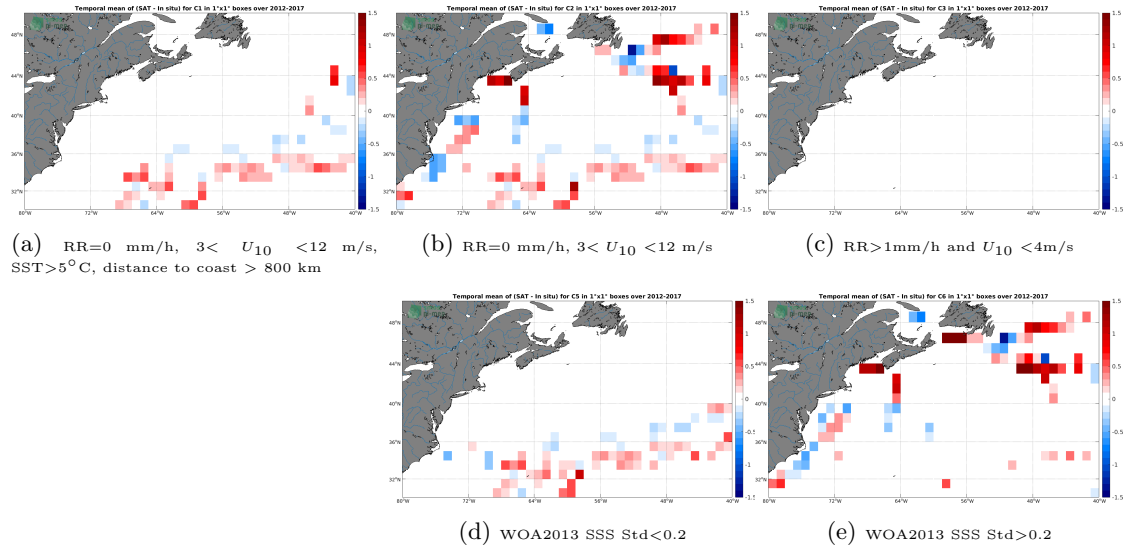
Figure 12: Temporal mean gridded over spatial boxes of size 1^{\circ}\times 1^{\circ} of \Delta SSS (SMOS L4 v2 Weekly (CATDS-CECOS-IFREMER) - TSG (GOSUD-Sailing-ship)) for 5 different subdatasets corresponding to:RR=0 mm/h, 3 < U_{10} < 12 m/s, SST >5^{\circ}\text{C} , distance to coast > 800 km (a), RR=0 mm/h, 3 < U_{10} < 12 m/s (b), RR >1 mm/h and U_{10} < 4 m/s (c), WOA2013 SSS Std <0.2 (d), WOA2013 SSS Std >0.2 (e).
