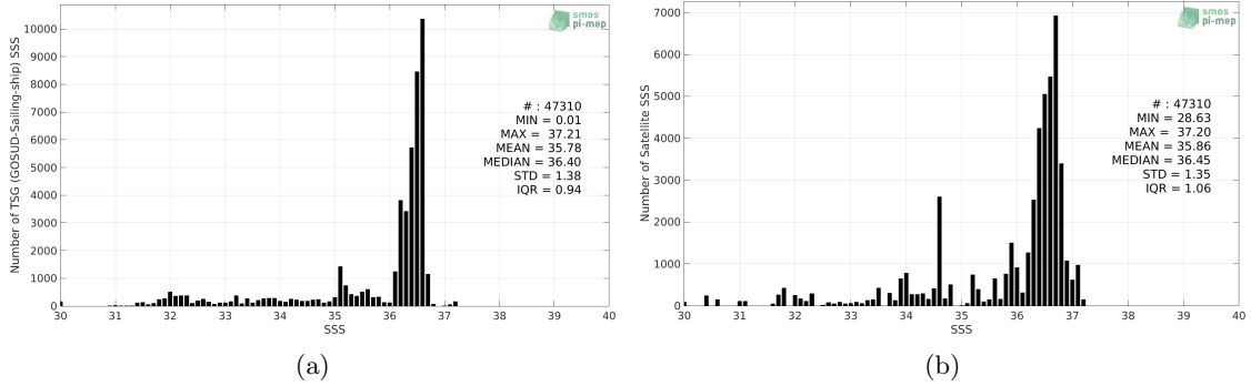
Figure 2: Histograms of SSS from TSG (GOSUD-Sailing-ship) (a) and SMOS L4 v2 Weekly (CATDS-CECOS-IFREMER) (b) considering all match-up pairs per bins of 0.1 over the Gulf Stream Pi-MEP region and for the full satellite product period.
