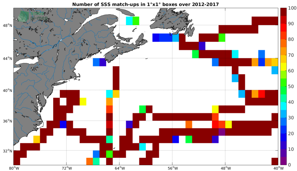
Figure 4: Number of SSS match-ups between TSG-GOSUD-Sailing-ship SSS and the SMOS-L4-CATDS-CECOS-IFREMER-V2-WEEKLY-0.5DEG SSS product for the Gulf Stream Pi-MEP region over 1°x1° boxes and for the full satellite product period.
