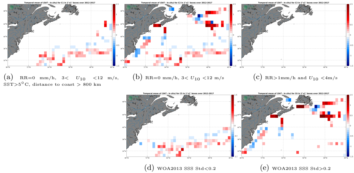
Figure 12: Temporal mean gridded over spatial boxes of size 1^{\circ}\times 1^{\circ} of \Delta SSS (SMOS-L4-CATDS-CECOS-IFREMER-V2-WEEKLY-0.5DEG - TSG-GOSUD-Sailing-ship) for 5 different subdatasets corresponding to:RR=0 mm/h, 3 < U_{10} < 12 m/s, SST >5^{\circ}\text{C} , distance to coast > 800 km (a), RR=0 mm/h, 3 < U_{10} < 12 m/s (b), RR >1 mm/h and U_{10} < 4 m/s (c), WOA2013 SSS Std <0.2 (d), WOA2013 SSS Std >0.2 (e).
