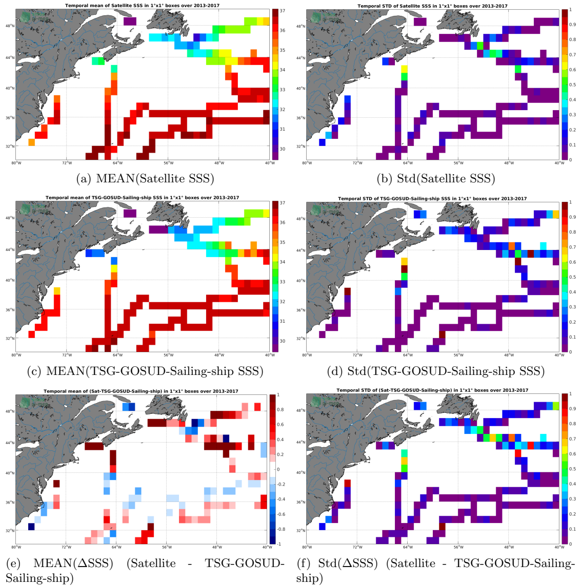
Figure 6: Temporal mean (left) and Std (right) of SSS from SMOS-L4-CATDS-CECOS-IFREMER-V2-WEEKLY-0.5DEG (top), TSG-GOSUD-Sailing-ship (middle), and of \Delta\text{SSS} (Satellite - TSG-GOSUD-Sailing-ship). Only match-up pairs are used to generate these maps.
