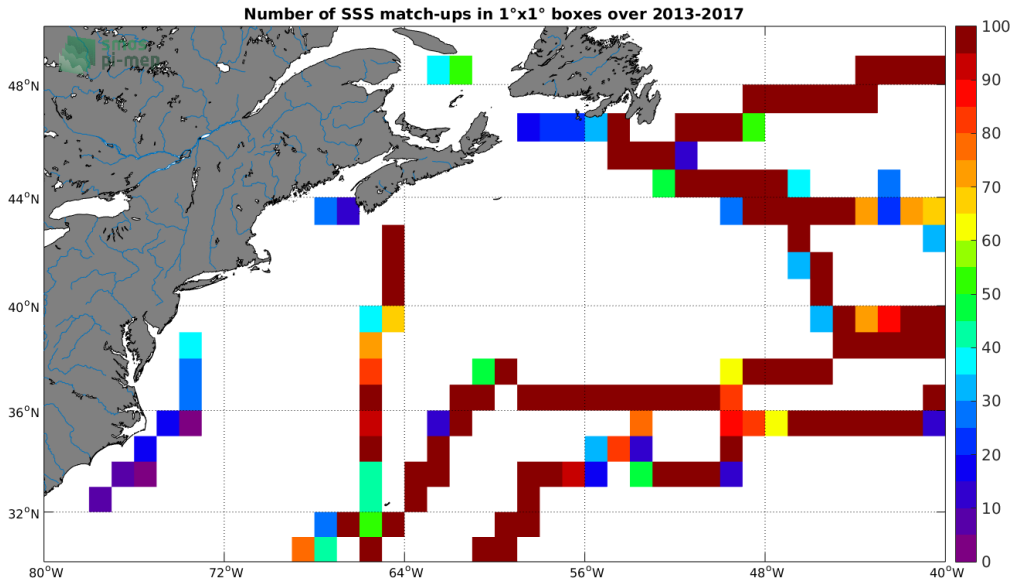
Figure 4: Number of SSS match-ups between TSG-GOSUD-Sailing-ship SSS and the SMOS-L4-CATDS-CECOS-IFREMER-V2-WEEKLY-0.5DEG SSS product for the Gulf Stream Pi-MEP region over 1^\circ \times 1^\circ boxes and for the full satellite product period.
