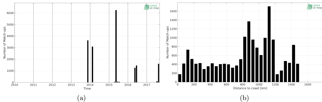
Figure 1: Number of match-ups between TSG-GOSUD-Sailing-ship and SMOS-L4-CATDS-CECOS-IFREMER-V2-WEEKLY-0.5DEG SSS as a function of time (a) and as function of the distance to coast (b) over the Gulf Stream Pi-MEP region and for the full satellite product period.
