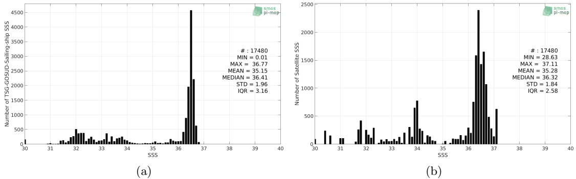
Figure 2: Histograms of SSS from TSG-GOSUD-Sailing-ship (a) and SMOS-L4-CATDS-CECOS-IFREMER-V2-WEEKLY-0.5DEG (b) considering all match-up pairs per bins of 0.1 over the Gulf Stream Pi-MEP region and for the full satellite product period.
