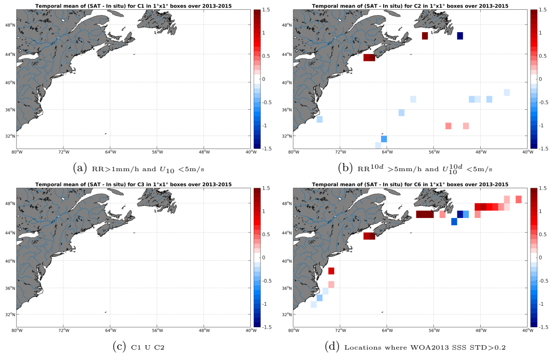
Figure 12: Temporal mean gridded over spatial boxes of size 1^\circ \times 1^\circ of \Delta SSS (SMOS-L4-CATDS-CECOS-IFREMER-V2-WEEKLY-0.5DEG - TSG-GOSUD-Sailing-ship) for 4 different subdatasets corresponding to:RR>1mm/h and U_{10} < 5\text{m/s} (a), RR^{10d} > 5\text{mm/h} and U_{10}^{10d} < 5\text{m/s} (b), C1 U C2 (c),Locations where WOA2013 SSS STD>0.2 (d).
