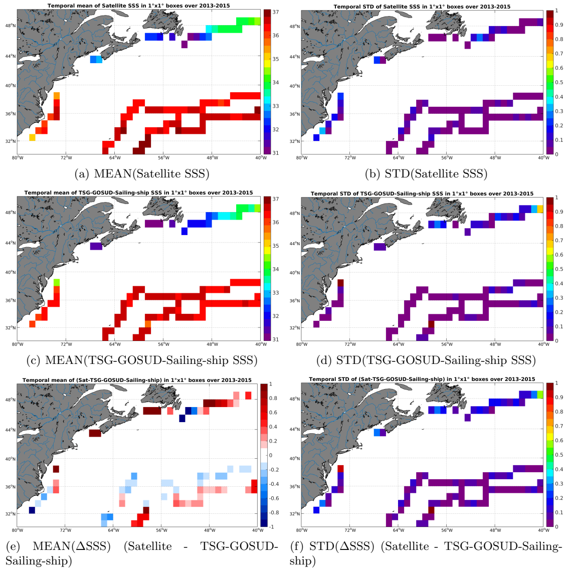
Figure 6: Temporal mean (left) and STD (right) of SSS from SMOS-L4-CATDS-CECOS-IFREMER-V2-WEEKLY-0.5DEG (top), TSG-GOSUD-Sailing-ship (middle), and of \Delta SSS (Satellite - TSG-GOSUD-Sailing-ship). Only match-up pairs are used to generate these maps.
