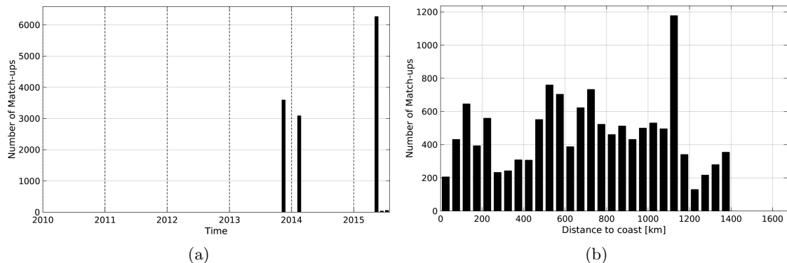
Figure 1: Number of match-ups between TSG-GOSUD-Sailing-ship and SMOS-L4-CATDS-CECOS-IFREMER-V2-WEEKLY-0.5DEG SSS as a function of time (a) and as function of the distance to coast (b) over the Gulf Stream Pi-MEP region and for the full satellite product period.
