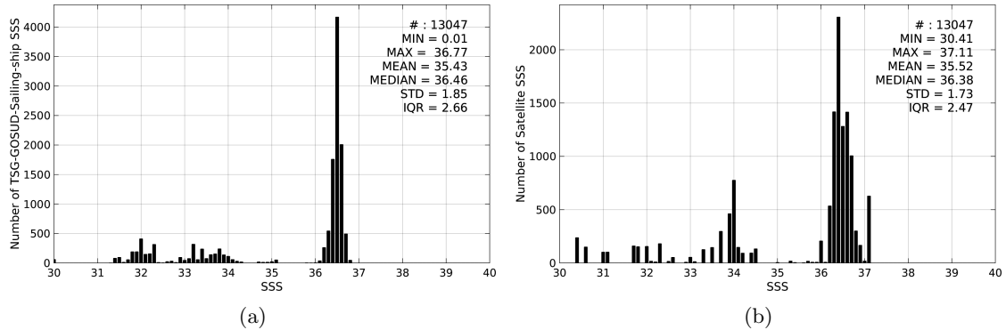
Figure 2: Histograms of SSS from TSG-GOSUD-Sailing-ship (a) and SMOS-L4-CATDS-CECOS-IFREMER-V2-WEEKLY-0.5DEG (b) considering all match-up pairs per bins of 0.1 over the Gulf Stream Pi-MEP region and for the full satellite product period.
