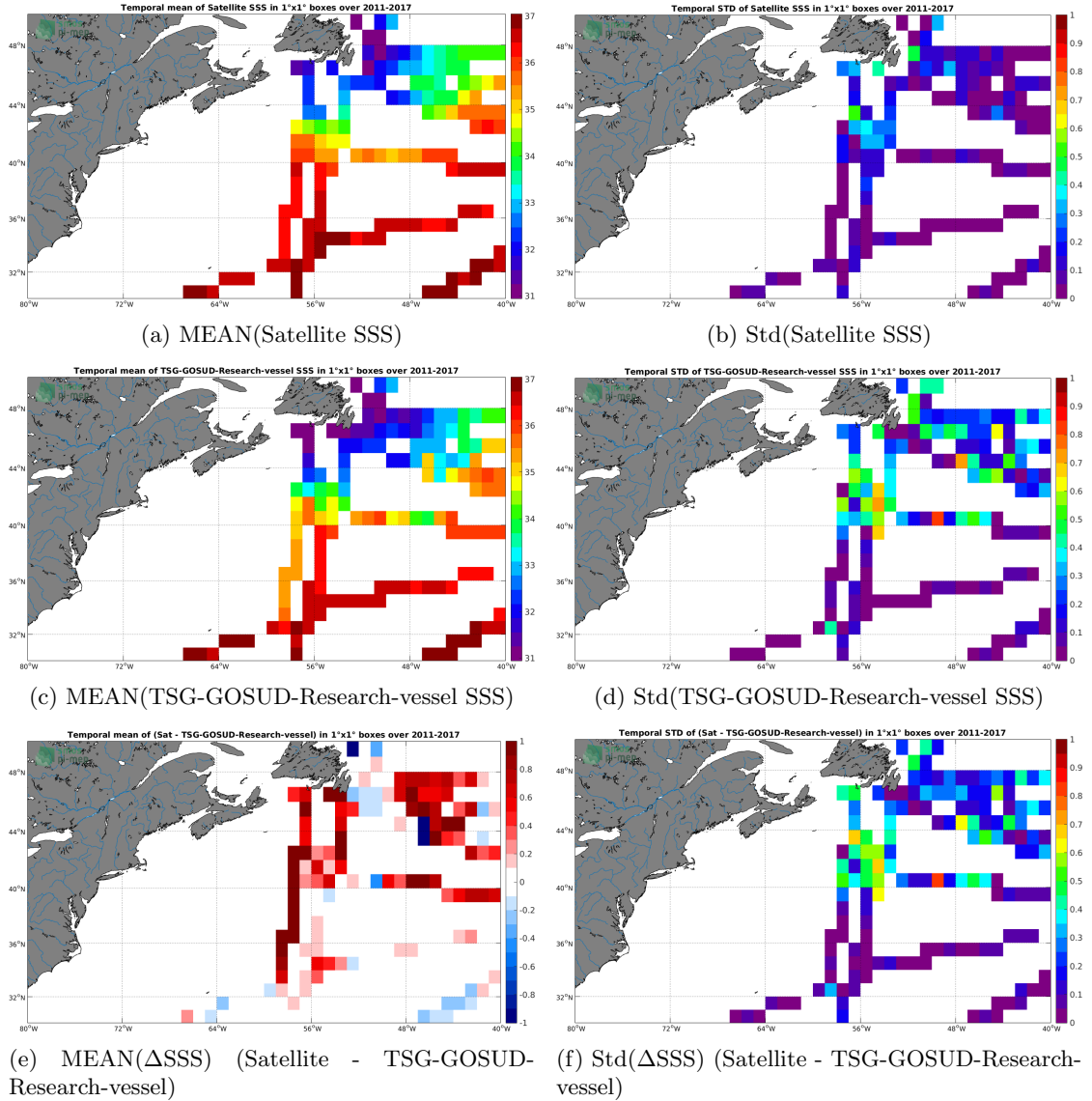
Figure 6: Temporal mean (left) and Std (right) of SSS from SMOS-L4-CATDS-CECOS-IFREMER-V2-WEEKLY-0.5DEG (top), TSG-GOSUD-Research-vessel (middle), and of \Delta SSS (Satellite - TSG-GOSUD-Research-vessel). Only match-up pairs are used to generate these maps.
