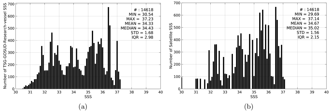
Figure 2: Histograms of SSS from TSG-GOSUD-Research-vessel (a) and SMOS-L4-CATDS-CECOS-IFREMER-V2-WEEKLY-0.5DEG (b) considering all match-up pairs per bins of 0.1 over the Gulf Stream Pi-MEP region and for the full satellite product period.
