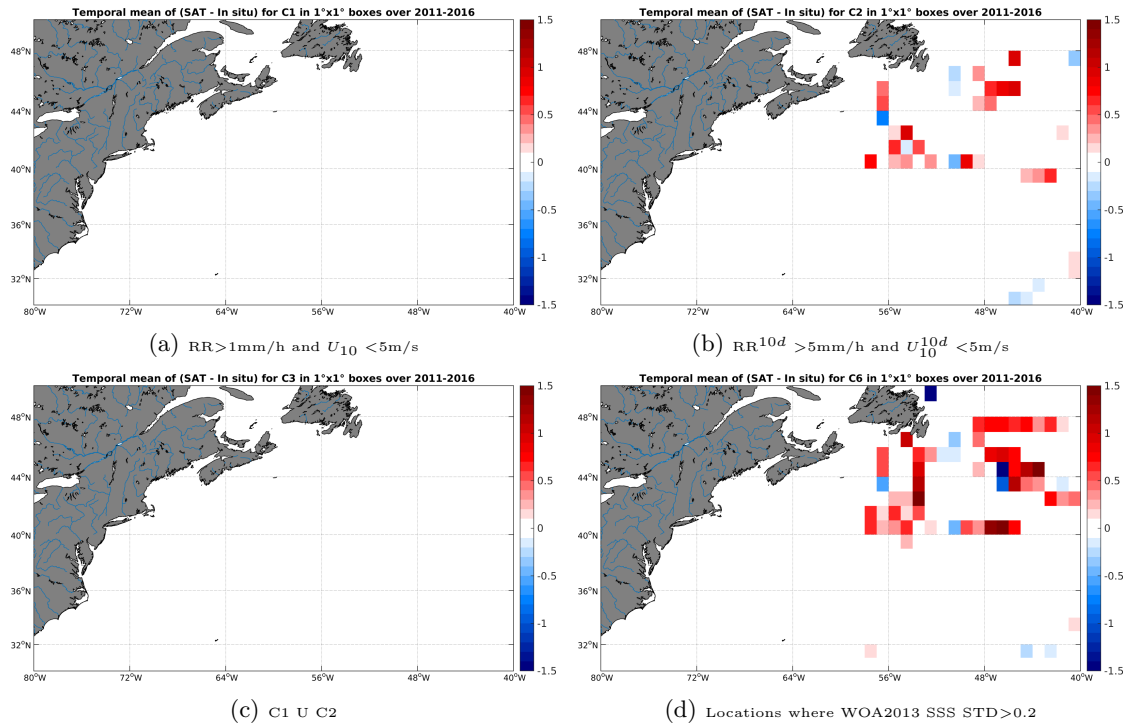
Figure 12: Temporal mean gridded over spatial boxes of size 1^\circ \times 1^\circ of \Delta SSS (SMOS-L4-CATDS-CECOS-IFREMER-V2-WEEKLY-0.5DEG - TSG-GOSUD-Research-vessel) for 4 different sub-datasets corresponding to:RR >1 mm/h and U_{10} < 5 m/s (a), RR ^{10d} > 5 mm/h and U_{10}^{10d} < 5 m/s (b), C1 U C2 (c),Locations where WOA2013 SSS STD >0.2 (d).
