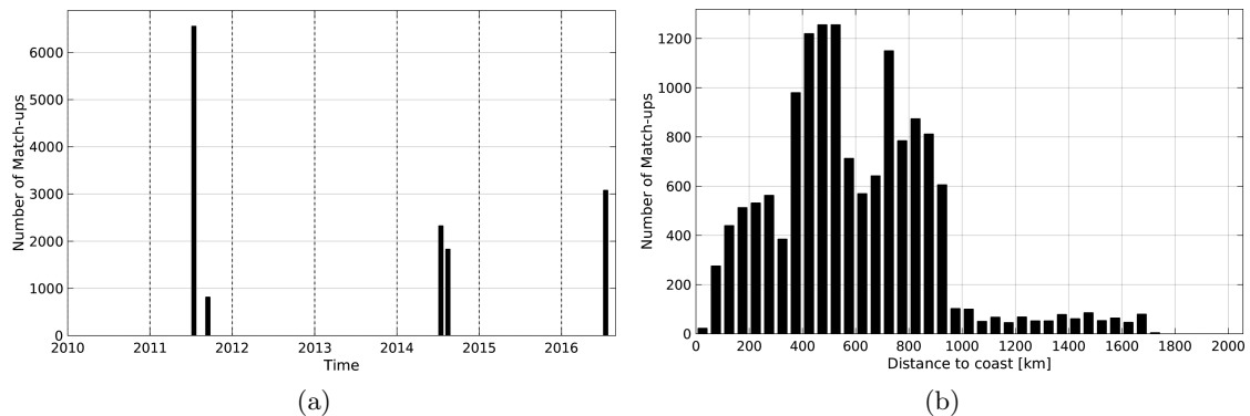
Figure 1: Number of match-ups between TSG-GOSUD-Research-vessel and SMOS-L4-CATDS-CECOS-IFREMER-V2-WEEKLY-0.5DEG SSS as a function of time (a) and as function of the distance to coast (b) over the Gulf Stream Pi-MEP region and for the full satellite product period.
