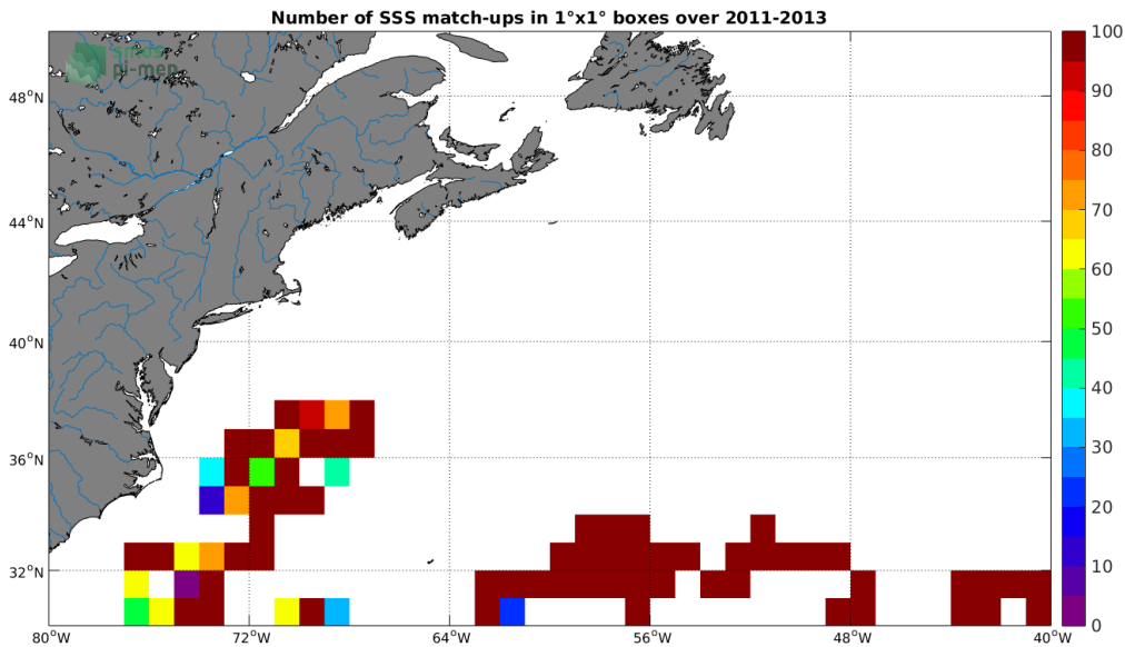
Figure 3: Number of SSS match-ups between Surface drifters SSS and the SMOS-L4-CATDS-CECOS-IFREMER-V2-WEEKLY-0.5DEG SSS product for the Gulf Stream Pi-MEP region over 1°x1° boxes and for the full satellite product period.
