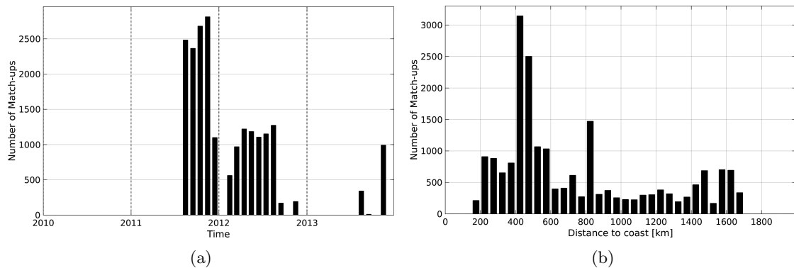
Figure 1: Number of match-ups between Surface drifters and SMOS-L4-CATDS-CECOS-IFREMER-V2-WEEKLY-0.5DEG SSS as a function of time (a) and as function of the distance to coast (b) over the Gulf Stream Pi-MEP region and for the full satellite product period.
