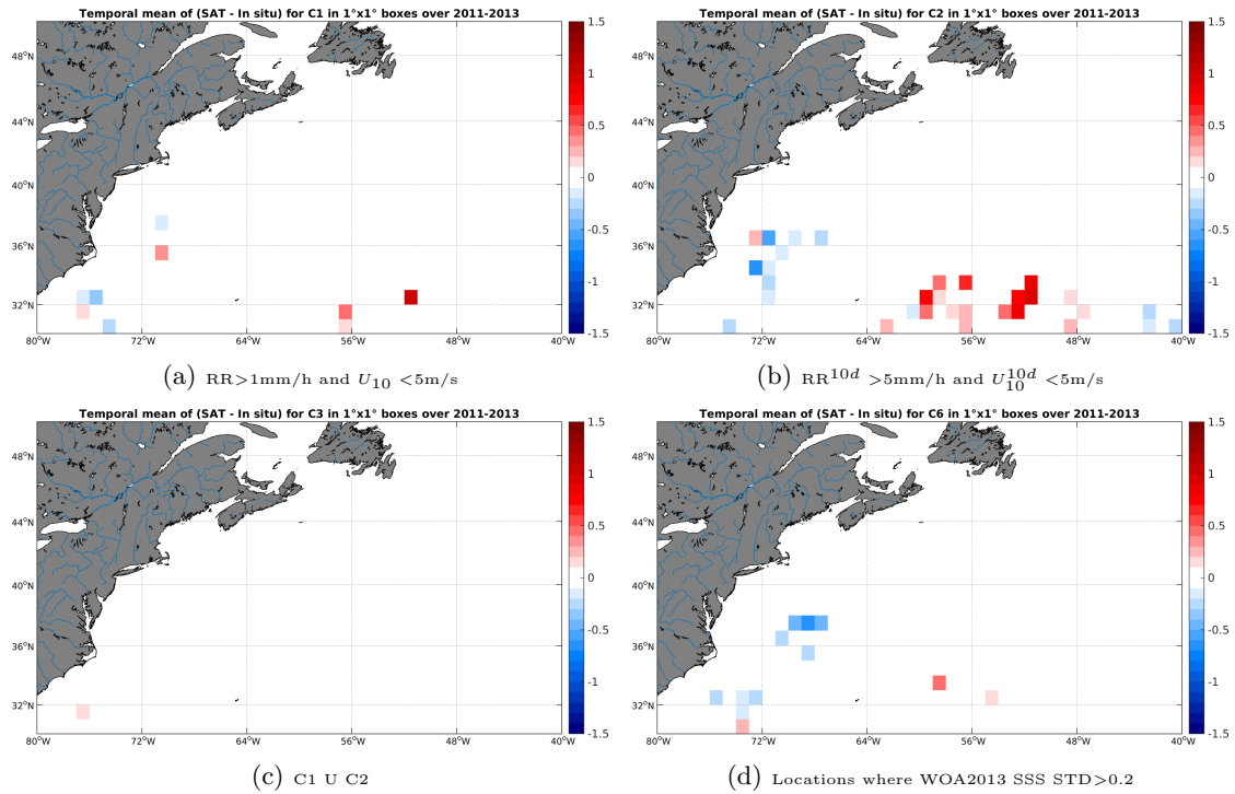
Figure 11: Temporal mean gridded over spatial boxes of size 1^\circ \times 1^\circ of \Delta SSS (SMOS-L4-CATDS-CECOS-IFREMER-V2-WEEKLY-0.5DEG - Surface drifters) for 4 different subdatasets corresponding to:RR>1mm/h and U_{10} < 5 m/s (a), RR^{10d} > 5 mm/h and U_{10}^{10d} < 5 m/s (b), C1 U C2 (c),Locations where WOA2013 SSS STD>0.2 (d).
