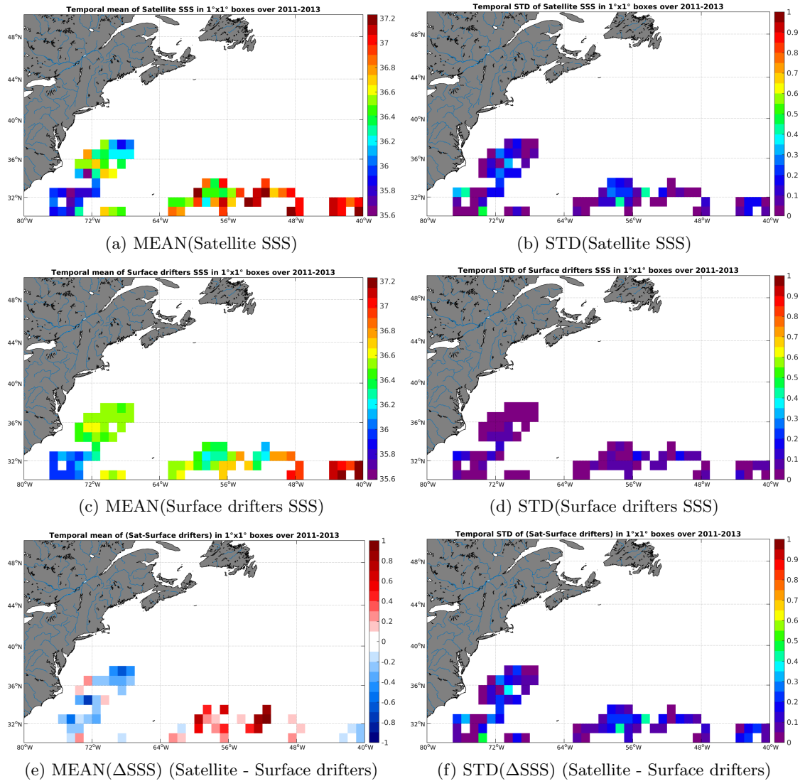
Figure 5: Temporal mean (left) and STD (right) of SSS from SMOS-L4-CATDS-CECOS-IFREMER-V2-WEEKLY-0.5DEG (top), Surface drifters (middle), and of \Delta SSS (Satellite - Surface drifters). Only match-up pairs are used to generate these maps.
