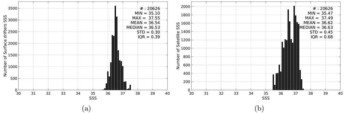
Figure 2: Histograms of SSS from Surface drifters (a) and SMOS-L4-CATDS-CECOS-IFREMER-V2-WEEKLY-0.5DEG (b) considering all match-up pairs per bins of 0.1 over the Gulf Stream Pi-MEP region and for the full satellite product period.
