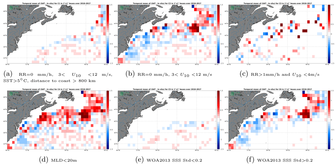
Figure 12: Temporal mean gridded over spatial boxes of size 1^\circ \times 1^\circ of \Delta SSS (SMOS L4 v2 Weekly (CATDS-CECOS-IFREMER) - Argo) for 6 different subdatasets corresponding to:RR=0 mm/h, 3 < U_{10} < 12 m/s, SST >5^\circ\text{C} , distance to coast > 800 km (a), RR=0 mm/h, 3 < U_{10} < 12 m/s (b), RR >1 mm/h and U_{10} < 4 m/s (c),MLD <20 m (d),WOA2013 SSS Std <0.2 (e),WOA2013 SSS Std >0.2 (f).
