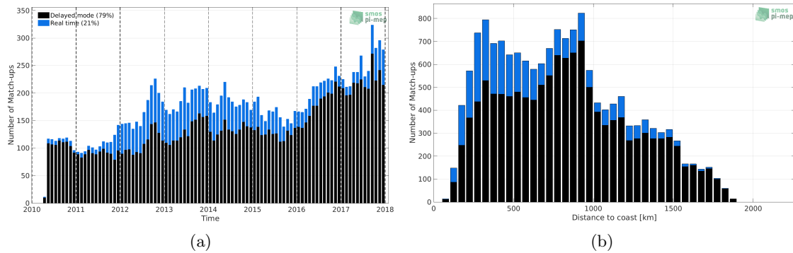
Figure 1: Number of match-ups between Argo and SMOS L4 v2 Weekly (CATDS-CECOS-IFREMER) SSS as a function of time (a) and as function of the distance to coast (b) over the Gulf Stream Pi-MEP region and for the full satellite product period.
