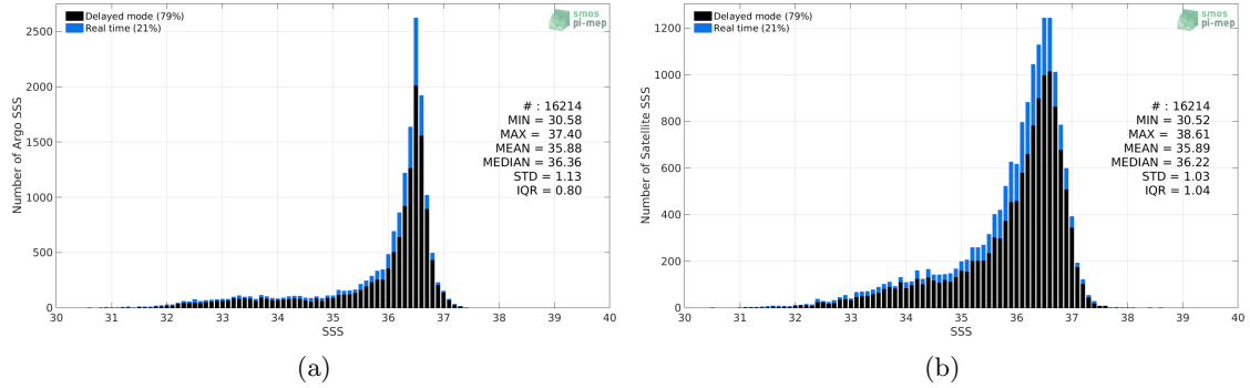
Figure 2: Histograms of SSS from Argo (a) and SMOS L4 v2 Weekly (CATDS-CECOS-IFREMER) (b) considering all match-up pairs per bins of 0.1 over the Gulf Stream Pi-MEP region and for the full satellite product period.
