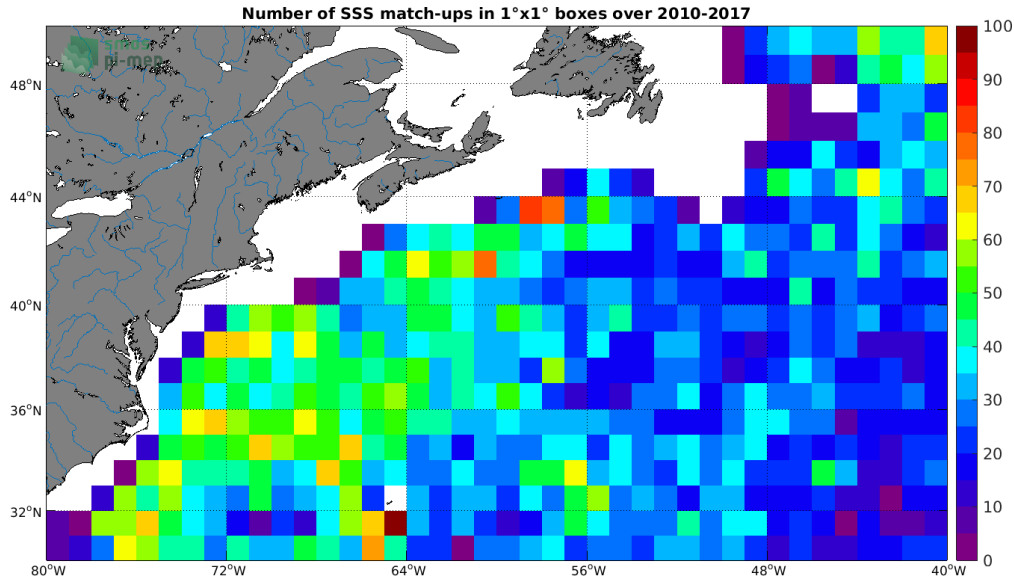
Figure 4: Number of SSS match-ups between Argo SSS and the SMOS L4 v2 Weekly (CATDS-CECOS-IFREMER) SSS product for the Gulf Stream Pi-MEP region over 1^\circ \times 1^\circ boxes and for the full satellite product period.
