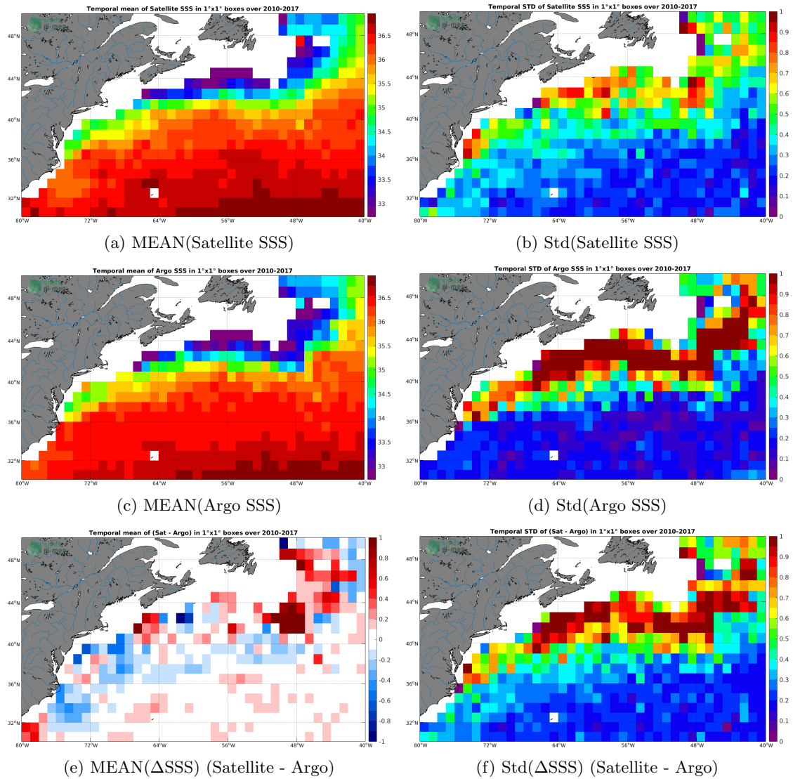
Figure 6: Temporal mean (left) and Std (right) of SSS from SMOS L4 v2 Weekly (CATDS-CECOS-IFREMER) (top), Argo (middle), and of \Delta\text{SSS} (Satellite - Argo). Only match-up pairs are used to generate these maps.
