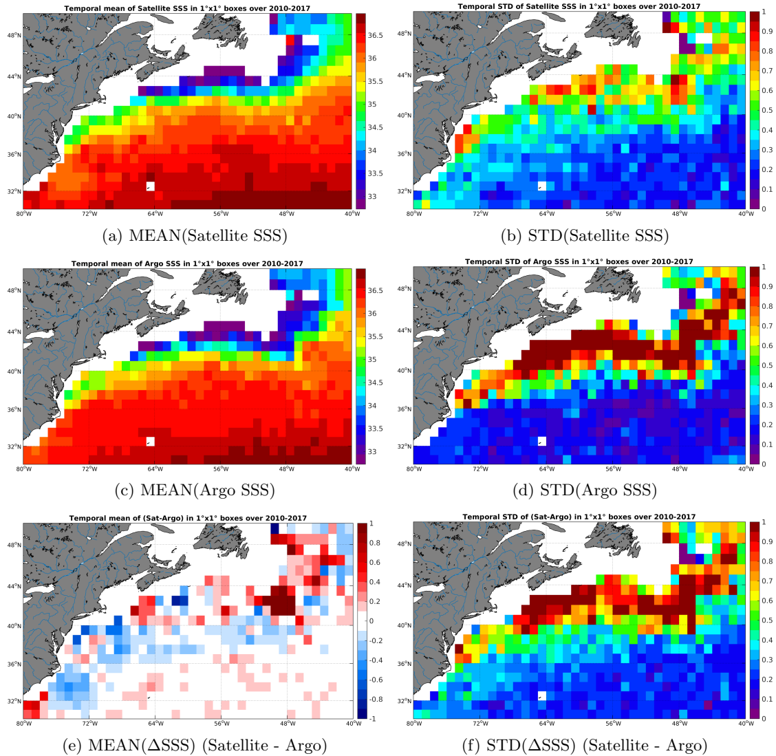
Figure 6: Temporal mean (left) and STD (right) of SSS from SMOS-L4-CATDS-CECOS-IFREMER-V2-WEEKLY-0.5DEG (top), Argo (middle), and of \Delta SSS (Satellite - Argo). Only match-up pairs are used to generate these maps.
