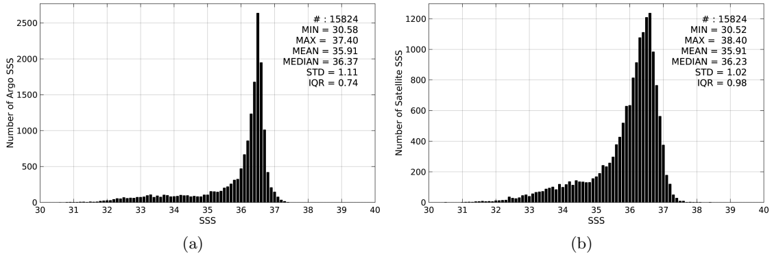
Figure 2: Histograms of SSS from Argo (a) and SMOS-L4-CATDS-CECOS-IFREMER-V2-WEEKLY-0.5DEG (b) considering all match-up pairs per bins of 0.1 over the Gulf Stream Pi-MEP region and for the full satellite product period.
