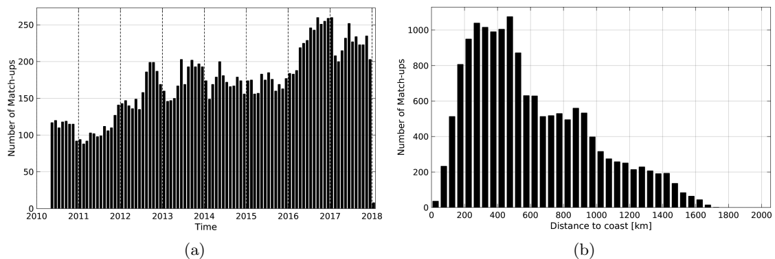
Figure 1: Number of match-ups between Argo and SMOS-L4-CATDS-CECOS-IFREMER-V2-WEEKLY-0.5DEG SSS as a function of time (a) and as function of the distance to coast (b) over the Gulf Stream Pi-MEP region and for the full satellite product period.
