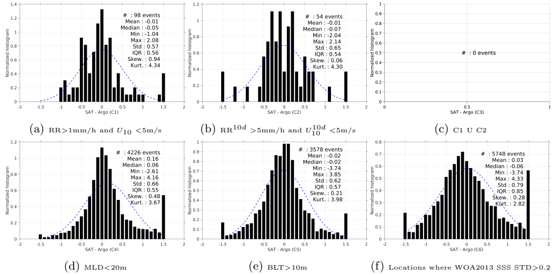
Figure 13: Normalized histogram of \Delta SSS (SMOS-L4-CATDS-CECOS-IFREMER-V2-WEEKLY-0.5DEG - Argo) for 6 different subdatasets corresponding to: RR > 1mm/h and U_{10} < 5 m/s (a), RR^{10d} > 5 mm/h and U_{10}^{10d} < 5 m/s (b), C1 U C2 (c), MLD < 20m (d), BLT > 10m (e), Locations where WOA2013 SSS STD > 0.2 (f).
