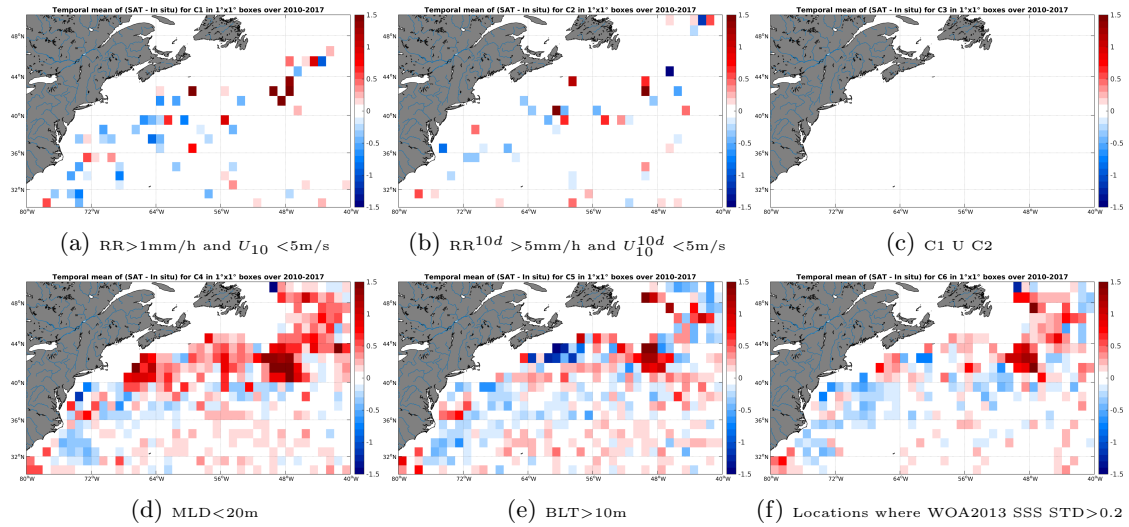
Figure 12: Temporal mean gridded over spatial boxes of size 1^\circ \times 1^\circ of \Delta SSS (SMOS-L4-CATDS-CECOS-IFREMER-V2-WEEKLY-0.5DEG - Argo) for 6 different subdatasets corresponding to:RR >1 mm/h and U_{10} < 5 m/s (a), RR ^{10d} > 5 mm/h and U_{10}^{10d} < 5 m/s (b), C1 U C2 (c),MLD <20 m (d),BLT >10 m (e),Locations where WOA2013 SSS STD >0.2 (f).
