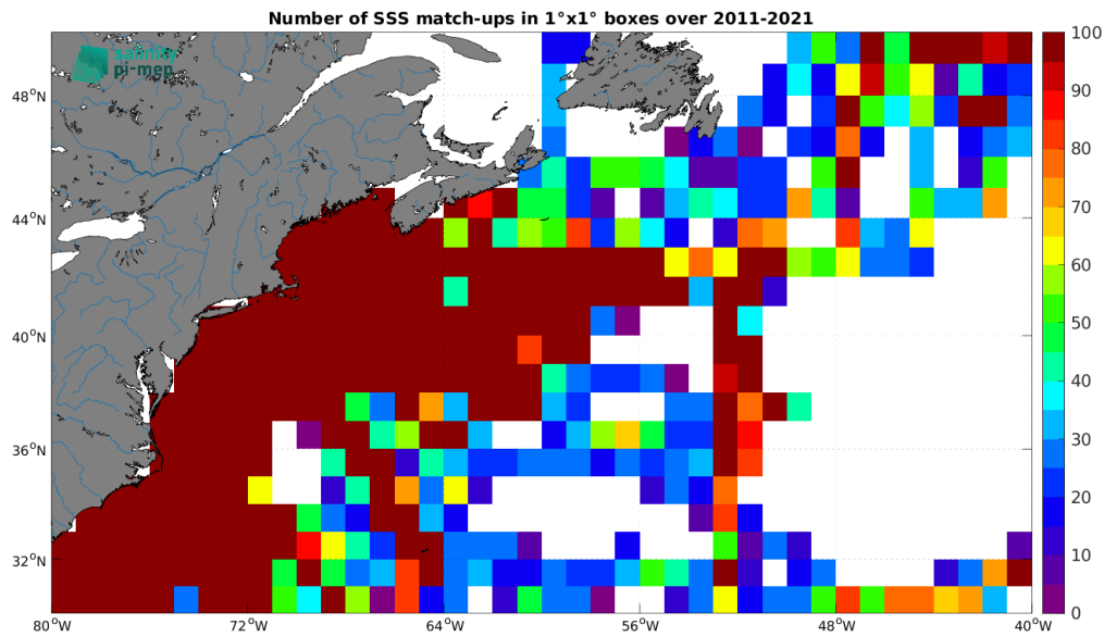
Figure 5: Number of SSS match-ups between TSG (SAMOS) SSS and the SMOS SSS L4 v2 - Daily (BEC) SSS product for the Gulf Stream Pi-MEP region over 1^{\circ} \times 1^{\circ} boxes and for the full satellite product period.
