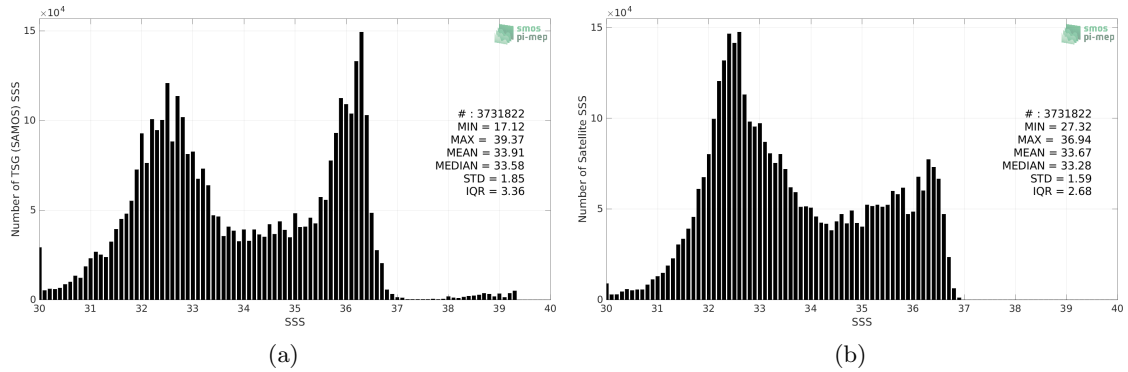
Figure 2: Histograms of SSS from TSG (SAMOS) (a) and SMOS SSS L4 v2 - Daily (BEC) (b) considering all match-up pairs per bins of 0.1 over the Gulf Stream Pi-MEP region and for the full satellite product period.
