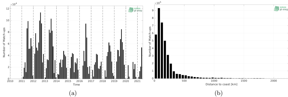
Figure 1: Number of match-ups between TSG (SAMOS) and SMOS SSS L4 v2 - Daily (BEC) SSS as a function of time (a) and as function of the distance to coast (b) over the Gulf Stream Pi-MEP region and for the full satellite product period.
