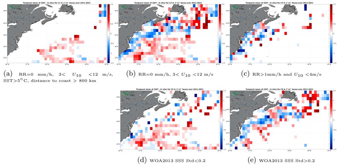
Figure 12: Temporal mean gridded over spatial boxes of size 1^\circ \times 1^\circ of \Delta SSS (SMOS SSS L4 v2 - Daily (BEC) - TSG (SAMOS)) for 5 different subdatasets corresponding to:RR=0 mm/h, 3 < U_{10} < 12 m/s, SST >5^\circ C, distance to coast > 800 km (a), RR=0 mm/h, 3 < U_{10} < 12 m/s (b), RR >1 mm/h and U_{10} < 4 m/s (c), WOA2013 SSS Std <0.2 (d), WOA2013 SSS Std >0.2 (e).
