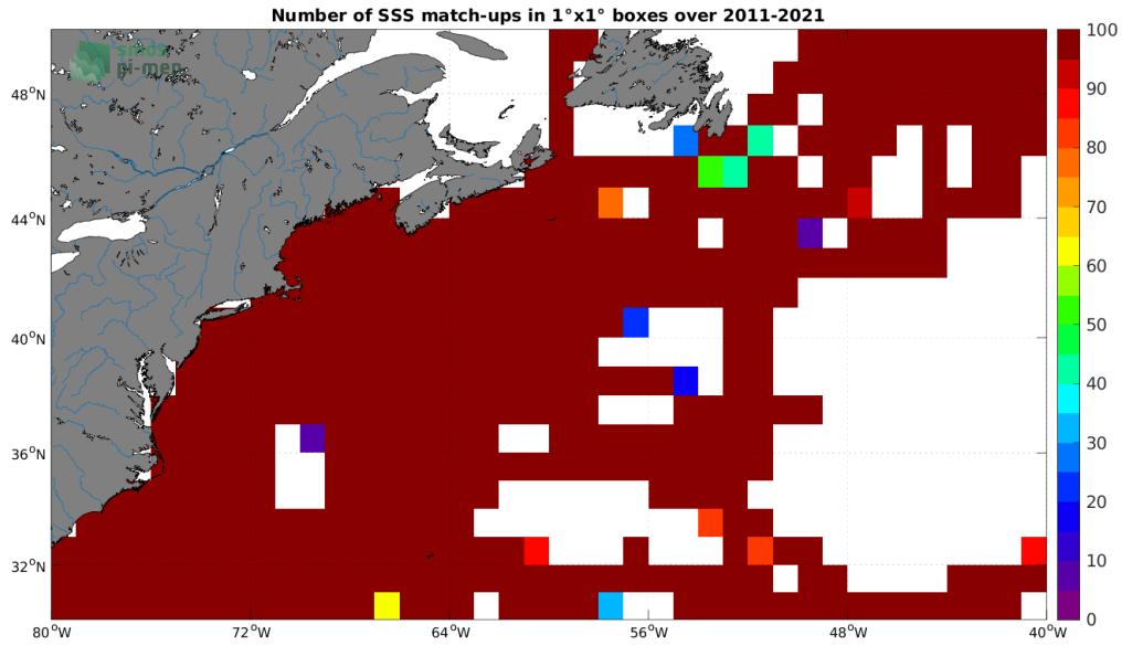
Figure 4: Number of SSS match-ups between TSG (SAMOS) SSS and the SMOS SSS L4 v2 - Daily (BEC) SSS product for the Gulf Stream Pi-MEP region over 1^\circ \times 1^\circ boxes and for the full satellite product period.
