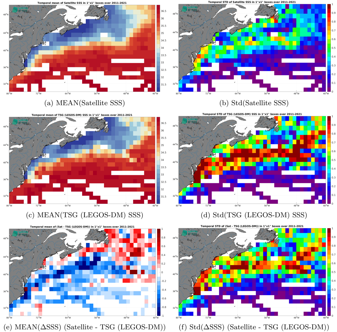
Figure 7: Temporal mean (left) and Std (right) of SSS from SMOS SSS L4 v2 - Daily (BEC) (top), TSG (LEGOS-DM) (middle), and of \Delta SSS (Satellite - TSG (LEGOS-DM)). Only match-up pairs are used to generate these maps.
