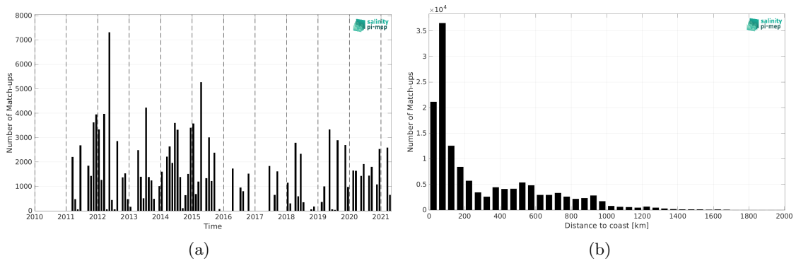
Figure 2: Number of match-ups between TSG (LEGOS-DM) and SMOS SSS L4 v2 - Daily (BEC) SSS as a function of time (a) and as function of the distance to coast (b) over the Gulf Stream Pi-MEP region and for the full satellite product period.
