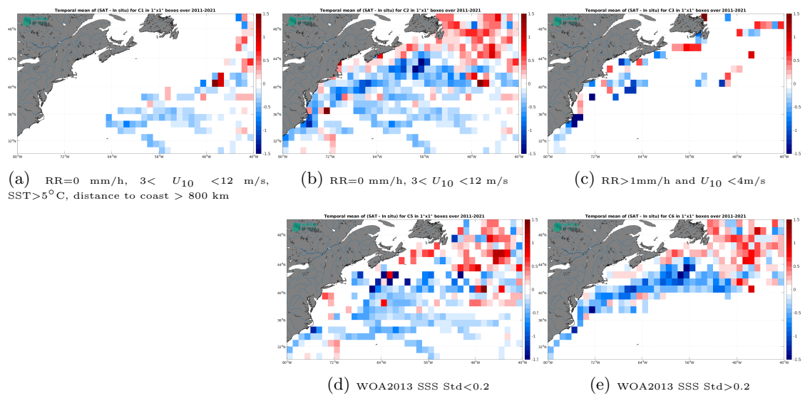
Figure 14: Temporal mean gridded over spatial boxes of size 1^\circ \times 1^\circ of \Delta SSS (SMOS SSS L4 v2 - Daily (BEC) - TSG (LEGOS-DM)) for 5 different subdatasets corresponding to:RR=0 mm/h, 3 < U_{10} < 12 m/s, SST>5°C, distance to coast > 800 km (a), RR=0 mm/h, 3 < U_{10} < 12 m/s (b), RR>1mm/h and U_{10} < 4 m/s (c), WOA2013 SSS Std<0.2 (d), WOA2013 SSS Std>0.2 (e).
