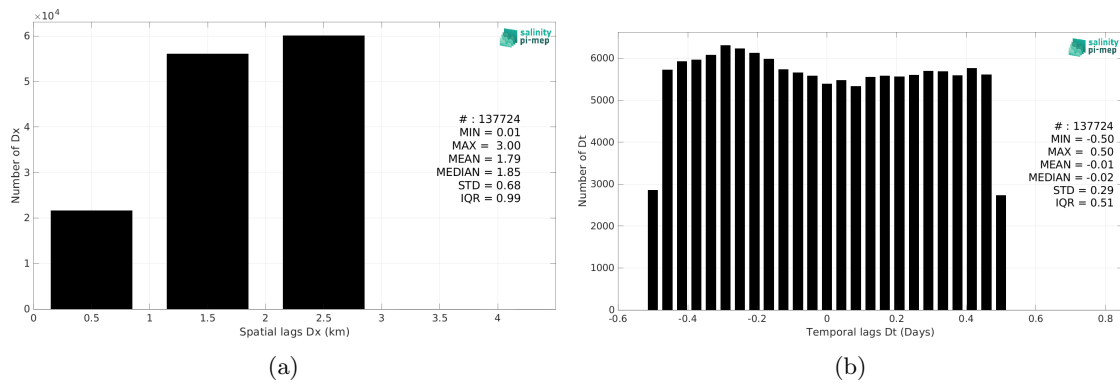
Figure 6: Histograms of the spatial (a) and temporal (b) lags between the location/time of the TSG (LEGOS-DM) measurement and the date of the corresponding SMOS SSS L4 v2 - Daily (BEC) SSS pixel.
