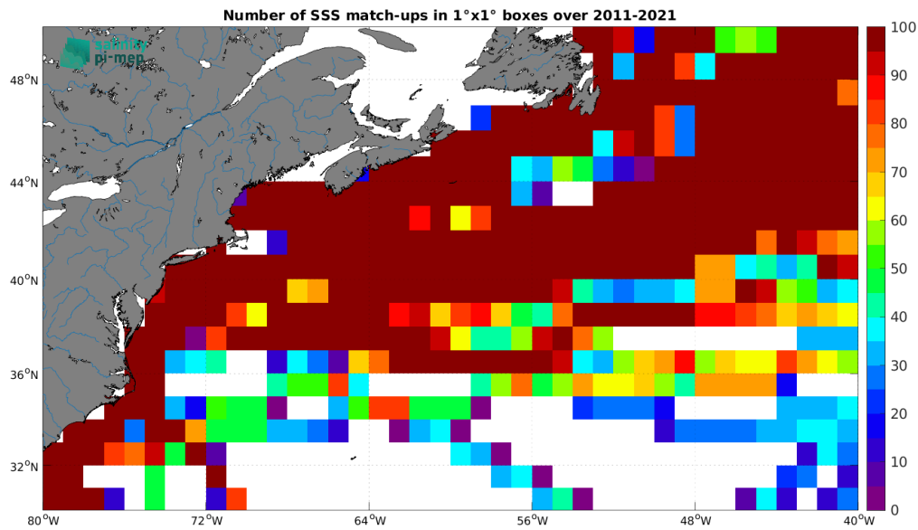
Figure 5: Number of SSS match-ups between TSG (LEGOS-DM) SSS and the SMOS SSS L4 v2 - Daily (BEC) SSS product for the Gulf Stream Pi-MEP region over 1^\circ \times 1^\circ boxes and for the full satellite product period.
