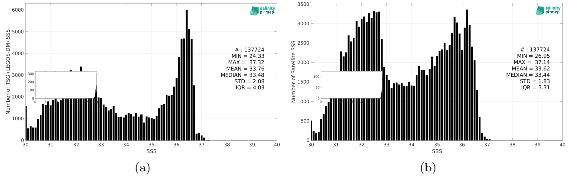
Figure 3: Histograms of SSS from TSG (LEGOS-DM) (a) and SMOS SSS L4 v2 - Daily (BEC) (b) considering all match-up pairs per bins of 0.1 over the Gulf Stream Pi-MEP region and for the full satellite product period.
