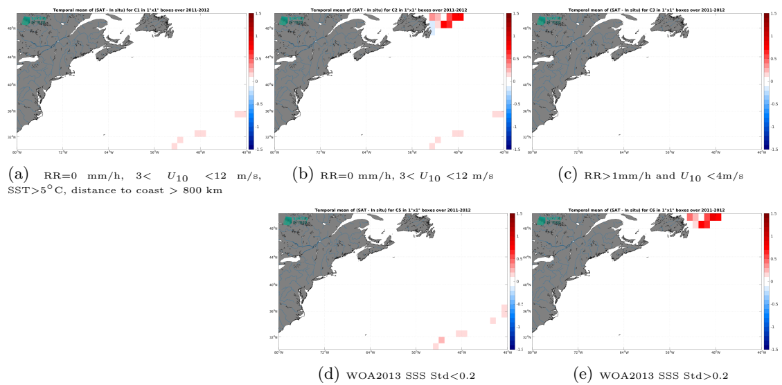
Figure 14: Temporal mean gridded over spatial boxes of size 1^\circ \times 1^\circ of \Delta SSS (SMOS SSS L4 v2 - Daily (BEC) - TSG (CSIC-UTM)) for 5 different subdatasets corresponding to: RR=0 mm/h, 3 < U_{10} < 12 m/s, SST > 5°C, distance to coast > 800 km (a), RR=0 mm/h, 3 < U_{10} < 12 m/s (b), RR > 1mm/h and U_{10} < 4 m/s (c), WOA2013 SSS Std < 0.2 (d), WOA2013 SSS Std > 0.2 (e).
