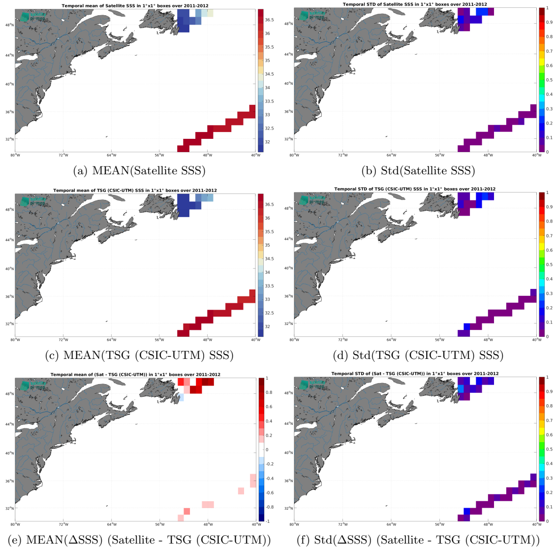
Figure 7: Temporal mean (left) and Std (right) of SSS from SMOS SSS L4 v2 - Daily (BEC) (top), TSG (CSIC-UTM) (middle), and of \Delta SSS (Satellite - TSG (CSIC-UTM)). Only match-up pairs are used to generate these maps.
