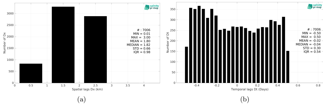
Figure 6: Histograms of the spatial (a) and temporal (b) lags between the location/time of the TSG (CSIC-UTM) measurement and the date of the corresponding SMOS SSS L4 v2 - Daily (BEC) SSS pixel.
