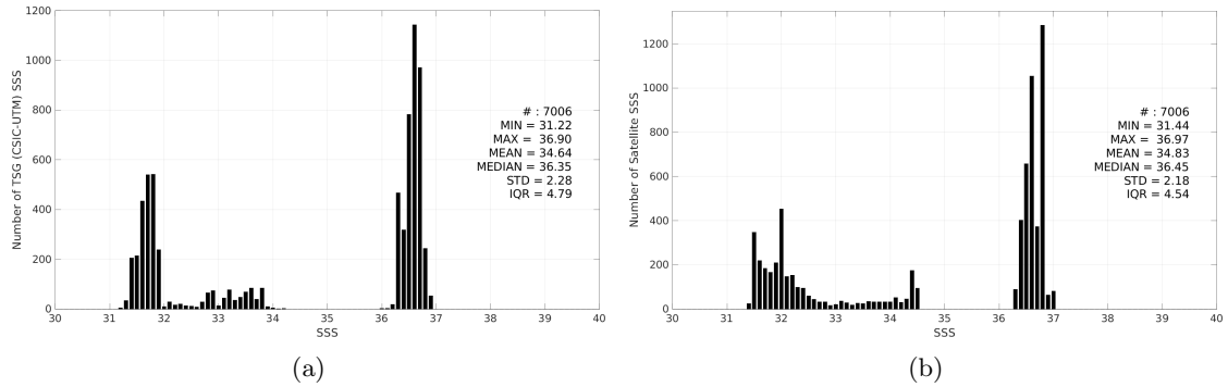
Figure 3: Histograms of SSS from TSG (CSIC-UTM) (a) and SMOS SSS L4 v2 - Daily (BEC) (b) considering all match-up pairs per bins of 0.1 over the Gulf Stream Pi-MEP region and for the full satellite product period.
