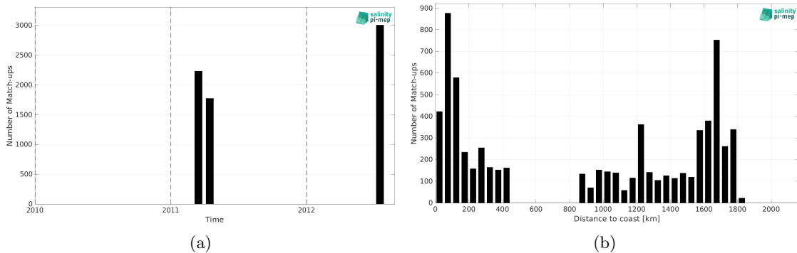
Figure 2: Number of match-ups between TSG (CSIC-UTM) and SMOS SSS L4 v2 - Daily (BEC) SSS as a function of time (a) and as function of the distance to coast (b) over the Gulf Stream Pi-MEP region and for the full satellite product period.
