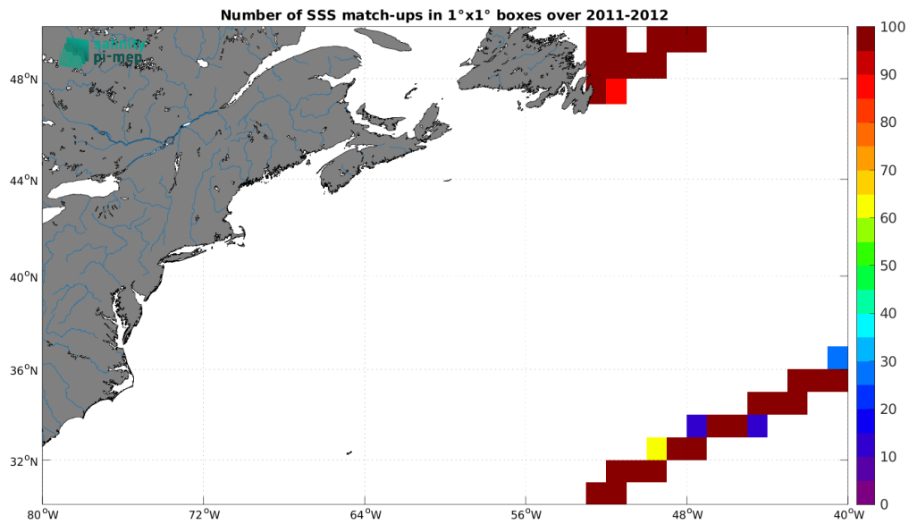
Figure 5: Number of SSS match-ups between TSG (CSIC-UTM) SSS and the SMOS SSS L4 v2 - Daily (BEC) SSS product for the Gulf Stream Pi-MEP region over 1^\circ \times 1^\circ boxes and for the full satellite product period.
