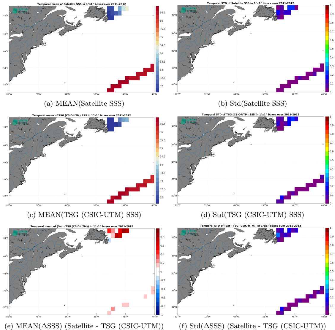
Figure 6: Temporal mean (left) and Std (right) of SSS from SMOS SSS L4 v2 - Daily (BEC) (top), TSG (CSIC-UTM) (middle), and of \Delta SSS (Satellite - TSG (CSIC-UTM)). Only match-up pairs are used to generate these maps.
