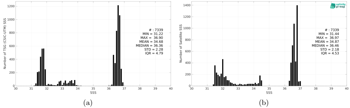
Figure 2: Histograms of SSS from TSG (CSIC-UTM) (a) and SMOS SSS L4 v2 - Daily (BEC) (b) considering all match-up pairs per bins of 0.1 over the Gulf Stream Pi-MEP region and for the full satellite product period.
