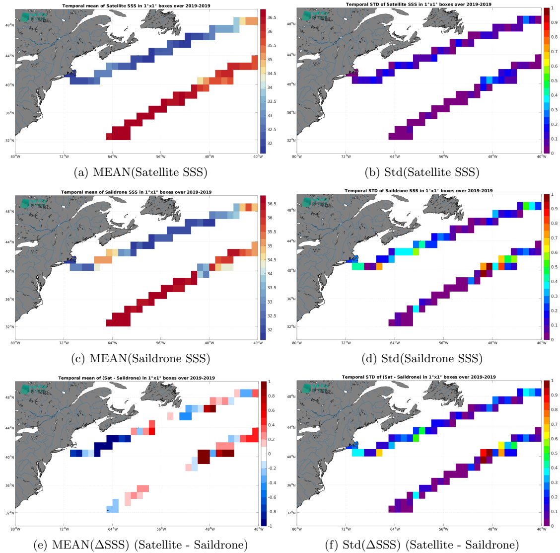
Figure 7: Temporal mean (left) and Std (right) of SSS from SMOS SSS L4 v2 - Daily (BEC) (top), Saildrone (middle), and of \Delta SSS (Satellite - Saildrone). Only match-up pairs are used to generate these maps.
