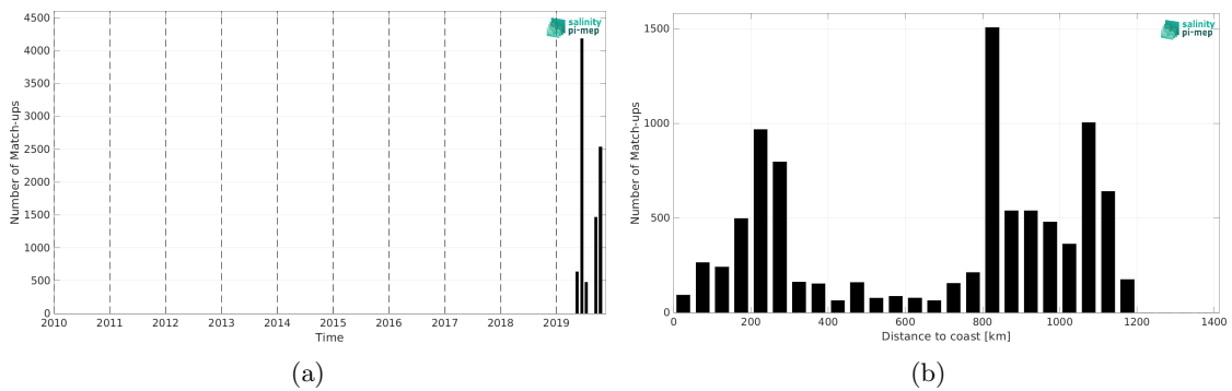
Figure 2: Number of match-ups between Saildrone and SMOS SSS L4 v2 - Daily (BEC) SSS as a function of time (a) and as function of the distance to coast (b) over the Gulf Stream Pi-MEP region and for the full satellite product period.
