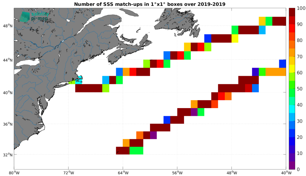
Figure 5: Number of SSS match-ups between Saildrone SSS and the SMOS SSS L4 v2 - Daily (BEC) SSS product for the Gulf Stream Pi-MEP region over 1^\circ \times 1^\circ boxes and for the full satellite product period.
