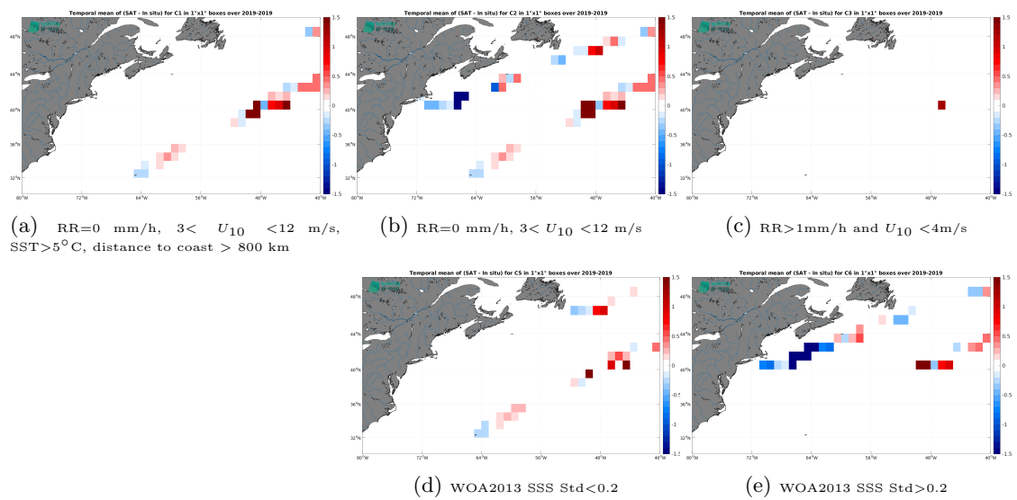
Figure 14: Temporal mean gridded over spatial boxes of size 1^\circ \times 1^\circ of \Delta SSS (SMOS SSS L4 v2 - Daily (BEC) - Sairdrone) for 5 different subdatasets corresponding to: RR=0 mm/h, 3 < U_{10} < 12 m/s, SST > 5°C, distance to coast > 800 km (a), RR=0 mm/h, 3 < U_{10} < 12 m/s (b), RR > 1mm/h and U_{10} < 4 m/s (c), WOA2013 SSS Std < 0.2 (d), WOA2013 SSS Std > 0.2 (e).
