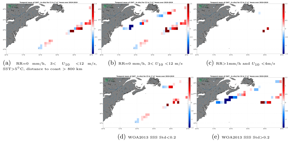
Figure 12: Temporal mean gridded over spatial boxes of size 1^\circ \times 1^\circ of \Delta SSS (SMOS SSS L4 v2 - Daily (BEC) - Sairdrone) for 5 different subdatasets corresponding to:RR=0 mm/h, 3 < U_{10} < 12 m/s, SST >5^\circ C, distance to coast > 800 km (a), RR=0 mm/h, 3 < U_{10} < 12 m/s (b), RR >1 mm/h and U_{10} < 4 m/s (c), WOA2013 SSS Std <0.2 (d), WOA2013 SSS Std >0.2 (e).
