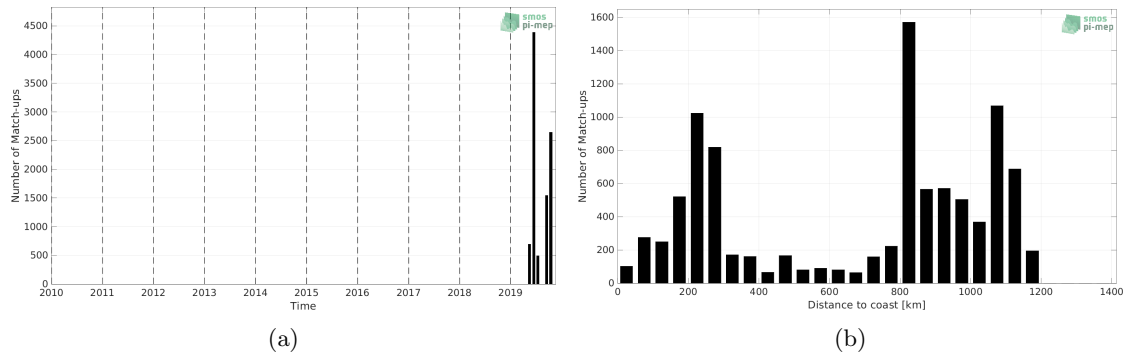
Figure 1: Number of match-ups between Saildrone and SMOS SSS L4 v2 - Daily (BEC) SSS as a function of time (a) and as function of the distance to coast (b) over the Gulf Stream Pi-MEP region and for the full satellite product period.
