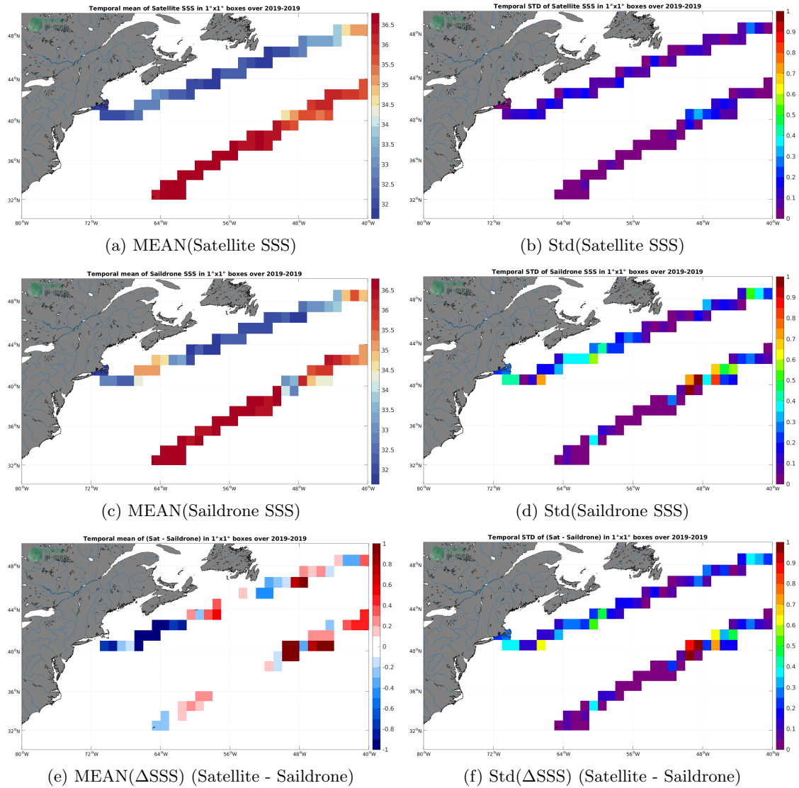
Figure 6: Temporal mean (left) and Std (right) of SSS from SMOS SSS L4 v2 - Daily (BEC) (top), Saildrone (middle), and of \Delta SSS (Satellite - Saildrone). Only match-up pairs are used to generate these maps.
