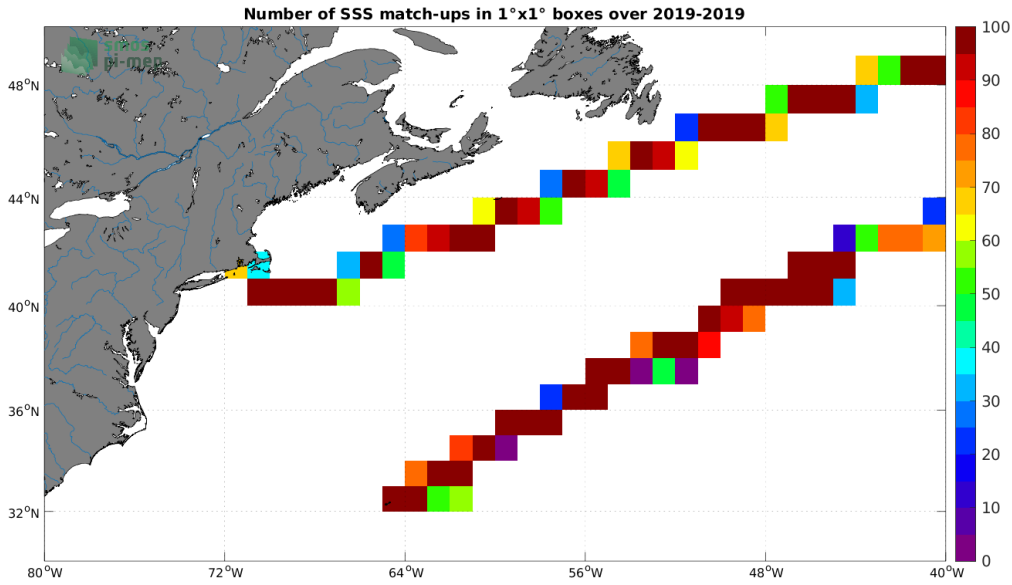
Figure 4: Number of SSS match-ups between Saildrone SSS and the SMOS SSS L4 v2 - Daily (BEC) SSS product for the Gulf Stream Pi-MEP region over 1^\circ \times 1^\circ boxes and for the full satellite product period.
