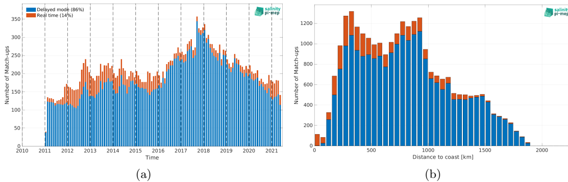
Figure 2: Number of match-ups between Argo and SMOS SSS L4 v2 - Daily (BEC) SSS as a function of time (a) and as function of the distance to coast (b) over the Gulf Stream Pi-MEP region and for the full satellite product period.
