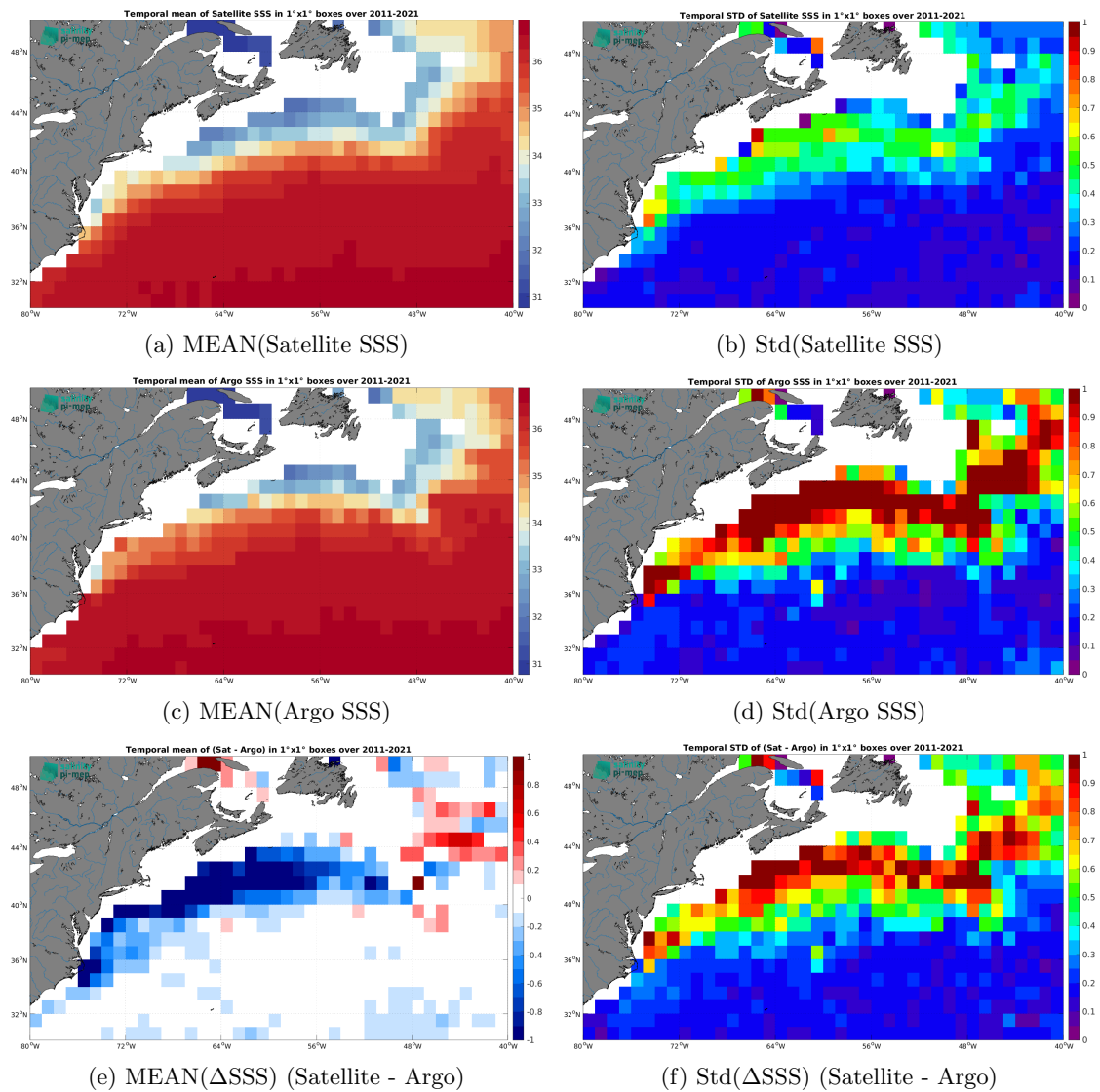
Figure 7: Temporal mean (left) and Std (right) of SSS from SMOS SSS L4 v2 - Daily (BEC) (top), Argo (middle), and of \Delta SSS (Satellite - Argo). Only match-up pairs are used to generate these maps.
