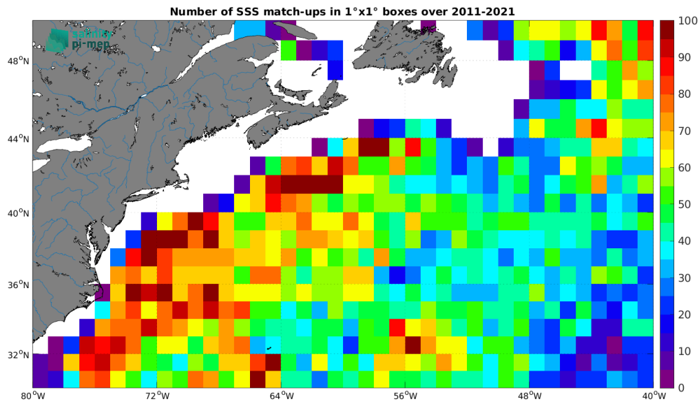
Figure 5: Number of SSS match-ups between Argo SSS and the SMOS SSS L4 v2 - Daily (BEC) SSS product for the Gulf Stream Pi-MEP region over 1^\circ \times 1^\circ boxes and for the full satellite product period.
