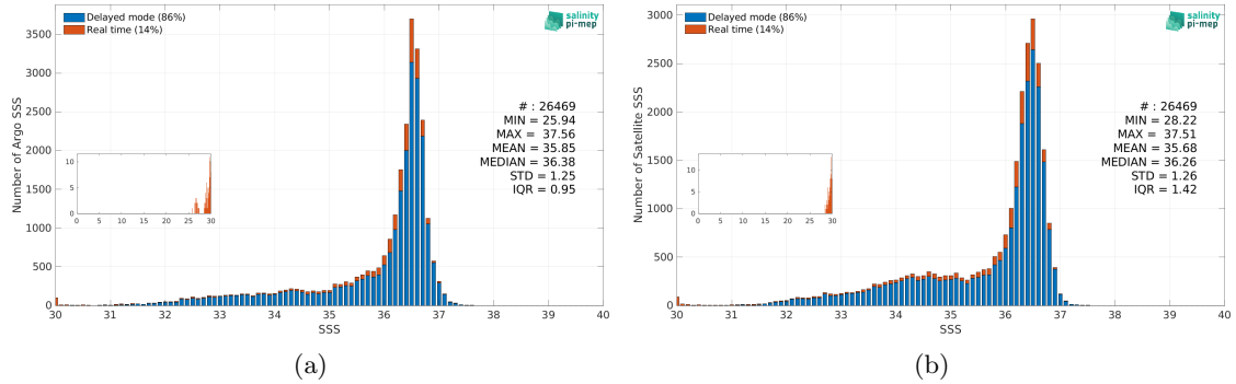
Figure 3: Histograms of SSS from Argo (a) and SMOS SSS L4 v2 - Daily (BEC) (b) considering all match-up pairs per bins of 0.1 over the Gulf Stream Pi-MEP region and for the full satellite product period.
