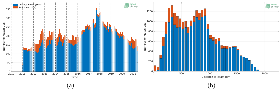
Figure 1: Number of match-ups between Argo and SMOS SSS L4 v2 - Daily (BEC) SSS as a function of time (a) and as function of the distance to coast (b) over the Gulf Stream Pi-MEP region and for the full satellite product period.
