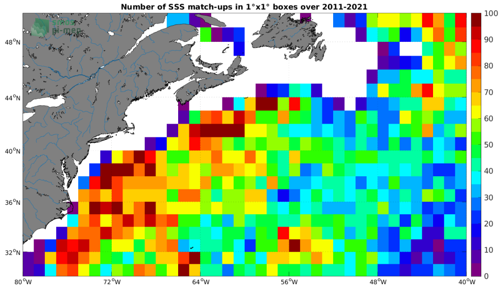
Figure 4: Number of SSS match-ups between Argo SSS and the SMOS SSS L4 v2 - Daily (BEC) SSS product for the Gulf Stream Pi-MEP region over 1^\circ \times 1^\circ boxes and for the full satellite product period.
