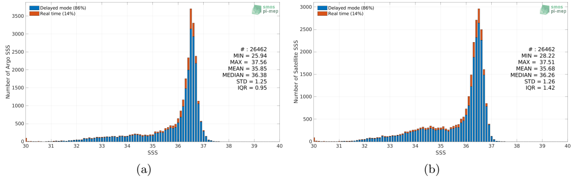
Figure 2: Histograms of SSS from Argo (a) and SMOS SSS L4 v2 - Daily (BEC) (b) considering all match-up pairs per bins of 0.1 over the Gulf Stream Pi-MEP region and for the full satellite product period.
