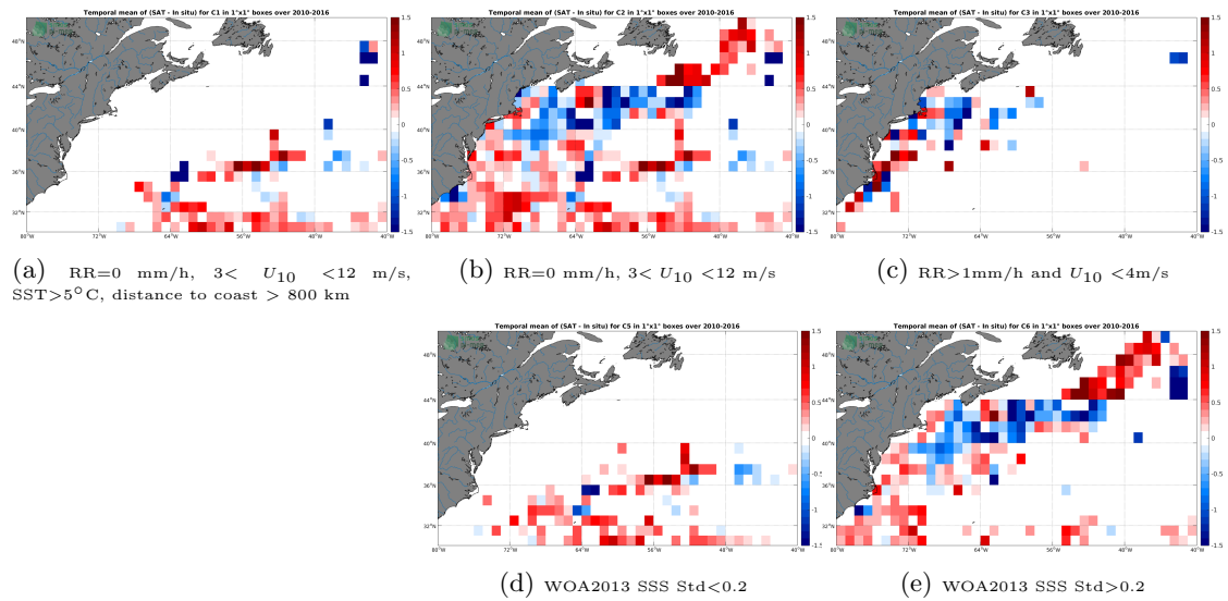
Figure 12: Temporal mean gridded over spatial boxes of size 1^\circ \times 1^\circ of \Delta SSS (SMOS-L3-ICDC-V3-MONTHLY-0.5DEG - TSG-SAMOS) for 5 different subdatasets corresponding to:RR=0 mm/h, 3 < U_{10} < 12 m/s, SST >5^\circ C, distance to coast > 800 km (a), RR=0 mm/h, 3 < U_{10} < 12 m/s (b), RR >1 mm/h and U_{10} < 4 m/s (c), WOA2013 SSS Std <0.2 (d), WOA2013 SSS Std >0.2 (e).
