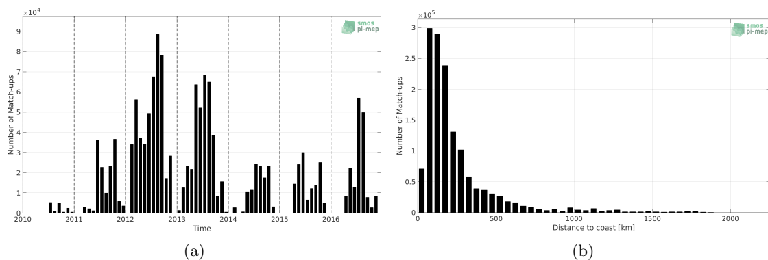
Figure 1: Number of match-ups between TSG-SAMOS and SMOS-L3-ICDC-V3-MONTHLY-0.5DEG SSS as a function of time (a) and as function of the distance to coast (b) over the Gulf Stream Pi-MEP region and for the full satellite product period.
