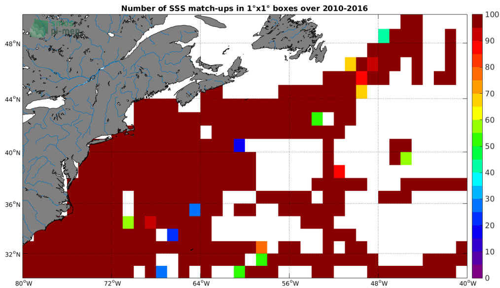
Figure 4: Number of SSS match-ups between TSG-SAMOS SSS and the SMOS-L3-ICDC-V3-MONTHLY-0.5DEG SSS product for the Gulf Stream Pi-MEP region over 1^\circ \times 1^\circ boxes and for the full satellite product period.
