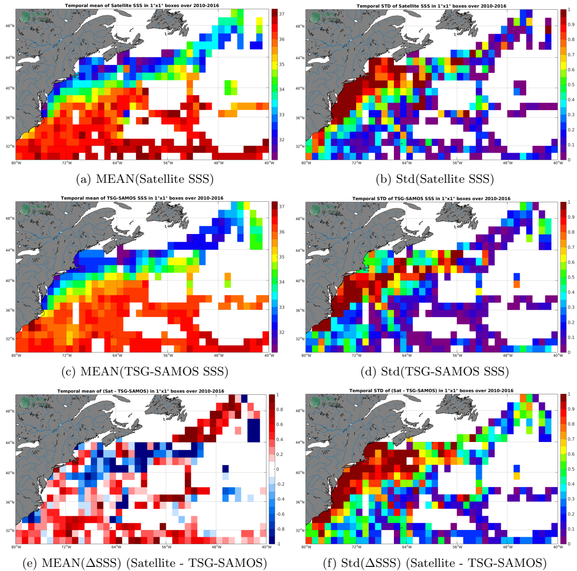
Figure 6: Temporal mean (left) and Std (right) of SSS from SMOS-L3-ICDC-V3-MONTHLY-0.5DEG (top), TSG-SAMOS (middle), and of \Delta SSS (Satellite - TSG-SAMOS). Only match-up pairs are used to generate these maps.
