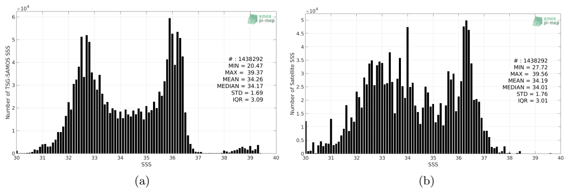
Figure 2: Histograms of SSS from TSG-SAMOS (a) and SMOS-L3-ICDC-V3-MONTHLY-0.5DEG (b) considering all match-up pairs per bins of 0.1 over the Gulf Stream Pi-MEP region and for the full satellite product period.
