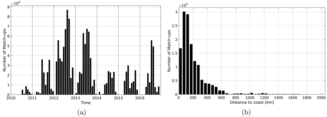
Figure 1: Number of match-ups between TSG-SAMOS and SMOS-L3-ICDC-V3-MONTHLY-0.5DEG SSS as a function of time (a) and as function of the distance to coast (b) over the Gulf Stream Pi-MEP region and for the full satellite product period.
