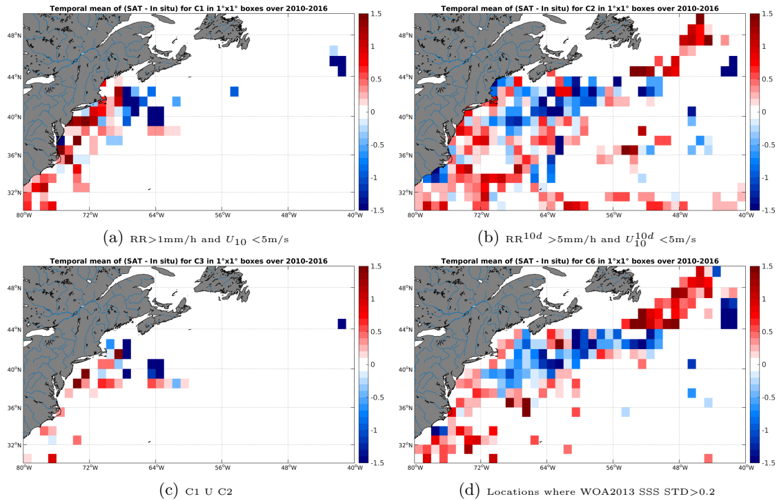
Figure 12: Temporal mean gridded over spatial boxes of size 1^\circ \times 1^\circ of \Delta SSS (SMOS-L3-ICDC-V3-MONTHLY-0.5DEG - TSG-SAMOS) for 4 different subdatasets corresponding to:RR>1mm/h and U_{10} < 5\text{m/s} (a), RR^{10d} > 5\text{mm/h} and U_{10}^{10d} < 5\text{m/s} (b), C1 U C2 (c),Locations where WOA2013 SSS STD>0.2 (d).
