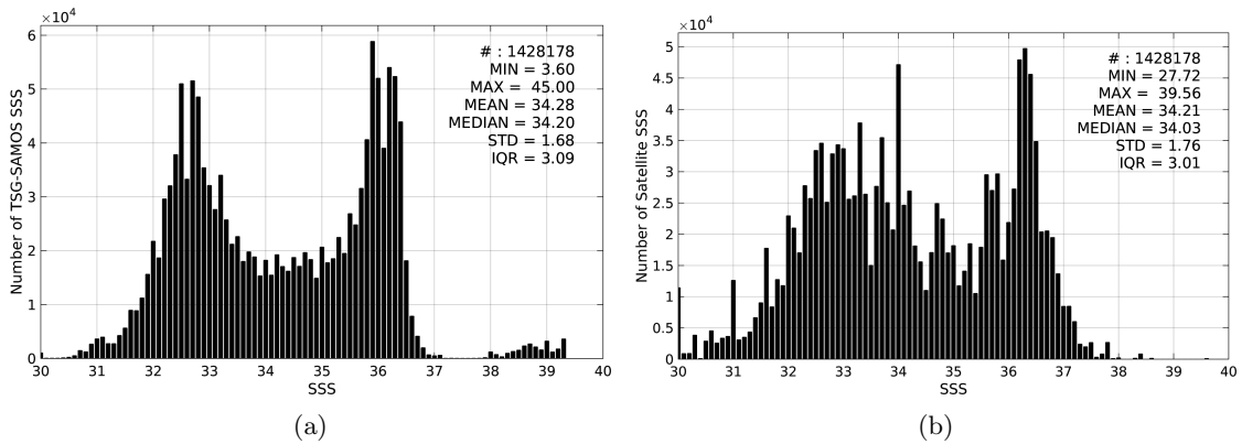
Figure 2: Histograms of SSS from TSG-SAMOS (a) and SMOS-L3-ICDC-V3-MONTHLY-0.5DEG (b) considering all match-up pairs per bins of 0.1 over the Gulf Stream Pi-MEP region and for the full satellite product period.
