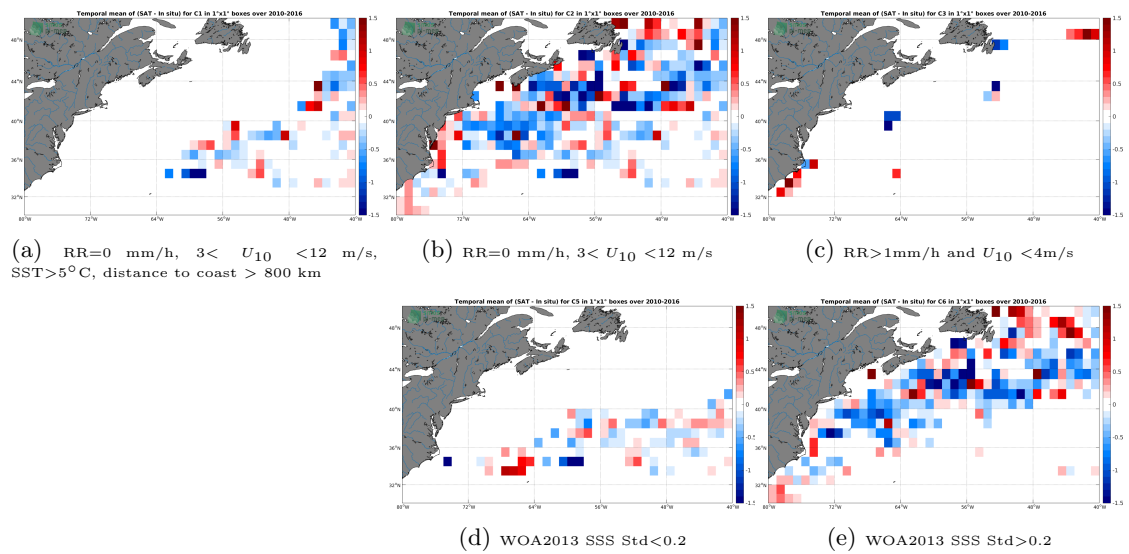
Figure 12: Temporal mean gridded over spatial boxes of size 1^\circ \times 1^\circ of \Delta SSS (SMOS SSS L3 v3 Monthly (ICDC) - TSG (LEGOS-DM)) for 5 different subdatasets corresponding to:RR=0 mm/h, 3 < U_{10} < 12 m/s, SST > 5^\circ\text{C} , distance to coast > 800 km (a), RR=0 mm/h, 3 < U_{10} < 12 m/s (b), RR > 1 mm/h and U_{10} < 4 m/s (c), WOA2013 SSS Std < 0.2 (d), WOA2013 SSS Std > 0.2 (e).
