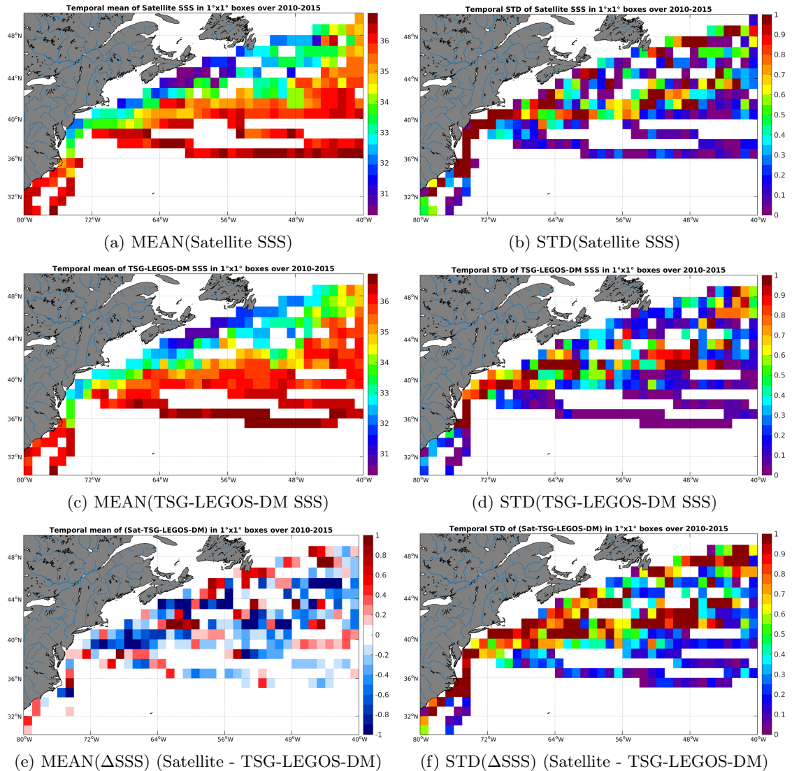
Figure 6: Temporal mean (left) and STD (right) of SSS from SMOS-L3-ICDC-V3-MONTHLY-0.5DEG (top), TSG-LEGOS-DM (middle), and of \Delta SSS (Satellite - TSG-LEGOS-DM). Only match-up pairs are used to generate these maps.
