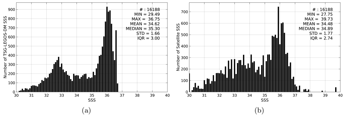
Figure 2: Histograms of SSS from TSG-LEGOS-DM (a) and SMOS-L3-ICDC-V3-MONTHLY-0.5DEG (b) considering all match-up pairs per bins of 0.1 over the Gulf Stream Pi-MEP region and for the full satellite product period.
