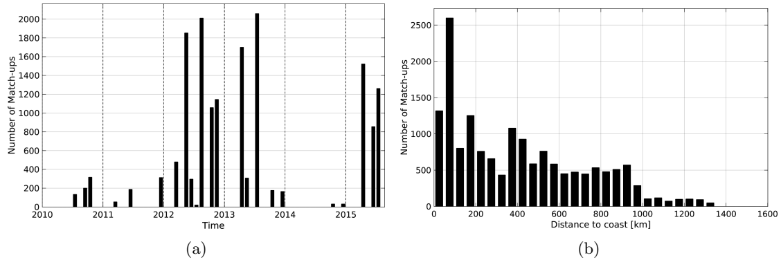
Figure 1: Number of match-ups between TSG-LEGOS-DM and SMOS-L3-ICDC-V3-MONTHLY-0.5DEG SSS as a function of time (a) and as function of the distance to coast (b) over the Gulf Stream Pi-MEP region and for the full satellite product period.
