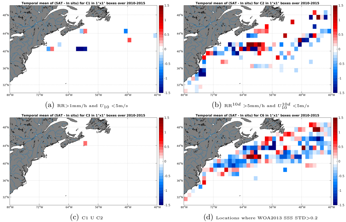
Figure 12: Temporal mean gridded over spatial boxes of size 1^\circ \times 1^\circ of \Delta SSS (SMOS-L3-ICDC-V3-MONTHLY-0.5DEG - TSG-LEGOS-DM) for 4 different subdatasets corresponding to: RR > 1\text{mm/h} and U_{10} < 5\text{m/s} (a), RR^{10d} > 5\text{mm/h} and U_{10}^{10d} < 5\text{m/s} (b), C1 U C2 (c), Locations where WOA2013 SSS STD > 0.2 (d).
