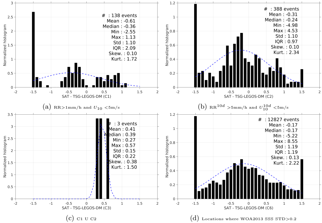
Figure 13: Normalized histogram of \Delta\text{SSS} (SMOS-L3-ICDC-V3-MONTHLY-0.5DEG - TSG-LEGOS-DM) for 6 different subdatasets corresponding to: RR > 1mm/h and U_{10} < 5\text{m/s} (a), \text{RR}^{10d} > 5\text{mm/h} and U_{10}^{10d} < 5\text{m/s} (b), C1 U C2 (c), Locations where WOA2013 SSS STD > 0.2 (d).
