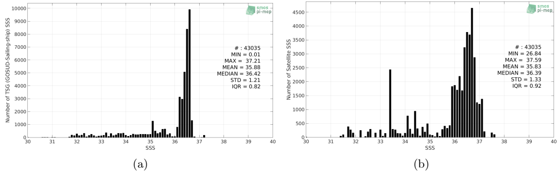
Figure 2: Histograms of SSS from TSG (GOSUD-Sailing-ship) (a) and SMOS SSS L3 v3 Monthly (ICDC) (b) considering all match-up pairs per bins of 0.1 over the Gulf Stream Pi-MEP region and for the full satellite product period.
