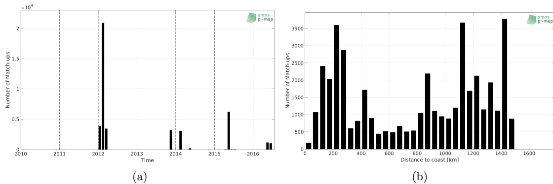
Figure 1: Number of match-ups between TSG (GOSUD-Sailing-ship) and SMOS SSS L3 v3 Monthly (ICDC) SSS as a function of time (a) and as function of the distance to coast (b) over the Gulf Stream Pi-MEP region and for the full satellite product period.
