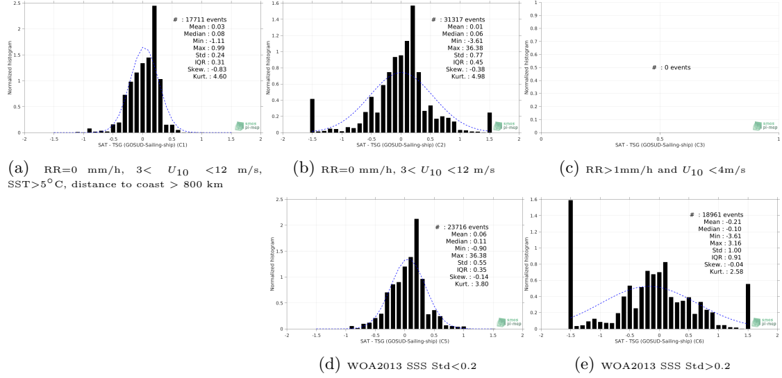
Figure 13: Normalized histogram of \Delta SSS (SMOS SSS L3 v3 Monthly (ICDC) - TSG (GOSUD-Sailing-ship)) for 5 different subdatasets corresponding to: RR=0 mm/h, 3 < U_{10} < 12 m/s, SST > 5°C, distance to coast > 800 km (a), RR=0 mm/h, 3 < U_{10} < 12 m/s (b), RR > 1mm/h and U_{10} < 4 m/s (c), WOA2013 SSS Std < 0.2 (d), WOA2013 SSS Std > 0.2 (e).
