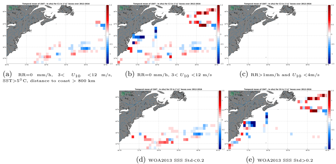
Figure 12: Temporal mean gridded over spatial boxes of size 1^\circ \times 1^\circ of \Delta SSS (SMOS SSS L3 v3 Monthly (ICDC) - TSG (GOSUD-Sailing-ship)) for 5 different subdatasets corresponding to: RR=0 mm/h, 3 < U_{10} < 12 m/s, SST > 5°C, distance to coast > 800 km (a), RR=0 mm/h, 3 < U_{10} < 12 m/s (b), RR > 1mm/h and U_{10} < 4 m/s (c), WOA2013 SSS Std < 0.2 (d), WOA2013 SSS Std > 0.2 (e).
