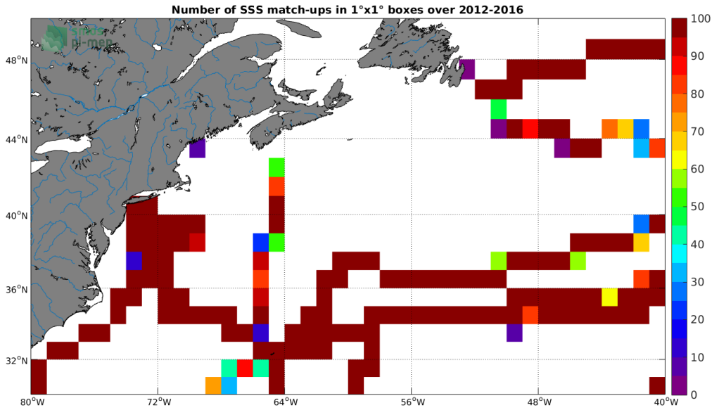
Figure 4: Number of SSS match-ups between TSG (GOSUD-Sailing-ship) SSS and the SMOS SSS L3 v3 Monthly (ICDC) SSS product for the Gulf Stream Pi-MEP region over 1^{\circ} \times 1^{\circ} boxes and for the full satellite product period.
