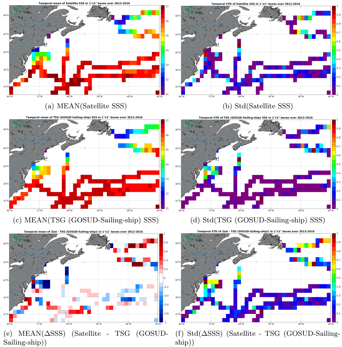
Figure 6: Temporal mean (left) and Std (right) of SSS from SMOS SSS L3 v3 Monthly (ICDC) (top), TSG (GOSUD-Sailing-ship) (middle), and of \Delta SSS (Satellite - TSG (GOSUD-Sailing-ship)). Only match-up pairs are used to generate these maps.
