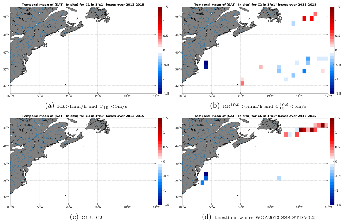
Figure 12: Temporal mean gridded over spatial boxes of size 1^\circ \times 1^\circ of \Delta SSS (SMOS-L3-ICDC-V3-MONTHLY-0.5DEG - TSG-GOSUD-Sailing-ship) for 4 different subdatasets corresponding to: RR > 1\text{mm/h} and U_{10} < 5\text{m/s} (a), RR^{10d} > 5\text{mm/h} and U_{10}^{10d} < 5\text{m/s} (b), C1 U C2 (c), Locations where WOA2013 SSS STD > 0.2 (d).
