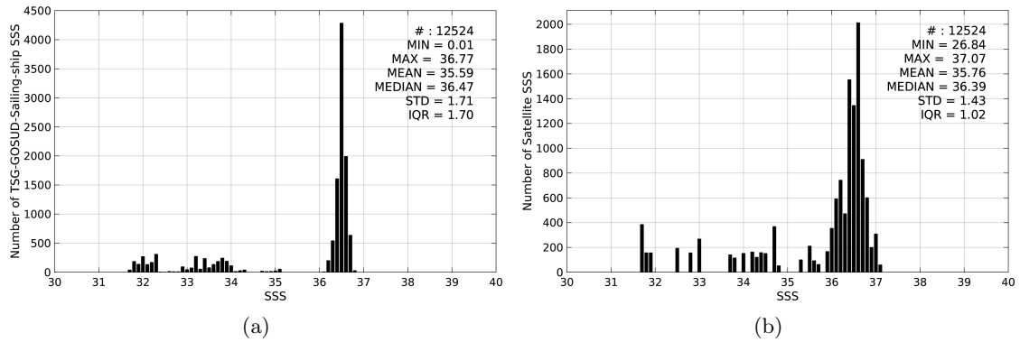
Figure 2: Histograms of SSS from TSG-GOSUD-Sailing-ship (a) and SMOS-L3-ICDC-V3-MONTHLY-0.5DEG (b) considering all match-up pairs per bins of 0.1 over the Gulf Stream Pi-MEP region and for the full satellite product period.
