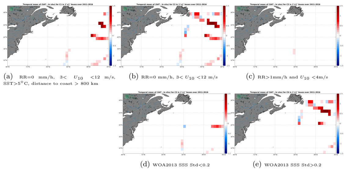
Figure 12: Temporal mean gridded over spatial boxes of size 1^\circ \times 1^\circ of \Delta\text{SSS} (SMOS SSS L3 v3 Monthly (ICDC) - TSG (GOSUD-Research-vessel)) for 5 different subdatasets corresponding to: RR=0 mm/h, 3 < U_{10} < 12 m/s, SST > 5°C, distance to coast > 800 km (a), RR=0 mm/h, 3 < U_{10} < 12 m/s (b), RR > 1mm/h and U_{10} < 4 m/s (c), WOA2013 SSS Std < 0.2 (d), WOA2013 SSS Std > 0.2 (e).
