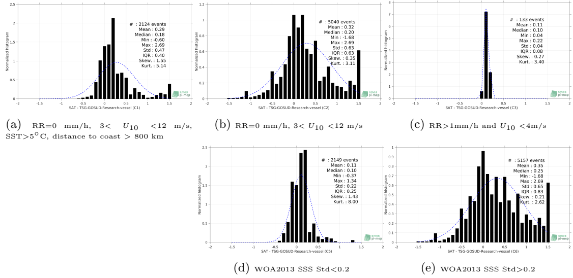
Figure 13: Normalized histogram of \Delta SSS (SMOS-L3-ICDC-V3-MONTHLY-0.5DEG - TSG-GOSUD-Research-vessel) for 5 different subdatasets corresponding to: RR=0 mm/h, 3 < U_{10} < 12 m/s, SST > 5^\circ\text{C} , distance to coast > 800 km (a), RR=0 mm/h, 3 < U_{10} < 12 m/s (b), RR > 1 mm/h and U_{10} < 4 m/s (c), WOA2013 SSS Std < 0.2 (d), WOA2013 SSS Std > 0.2 (e).
