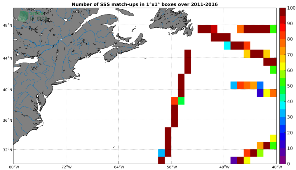
Figure 4: Number of SSS match-ups between TSG-GOSUD-Research-vessel SSS and the SMOS-L3-ICDC-V3-MONTHLY-0.5DEG SSS product for the Gulf Stream Pi-MEP region over 1°x1° boxes and for the full satellite product period.
